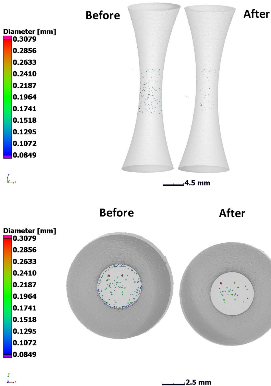
Figure 2: 3D visualizations of porosity in the central 10 mm of the gauge section before (left) and after peening (right). This clearly shows the reduction of porosity, especially for the near-surface pores, shown in (a) front and (b) top views.
