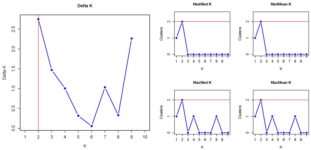
Figure S1. Delineated results of Evanno (Evanno et al., 2005) (on the left) and Puechmaille (Puechmaille, 2016) (on the right) methods for determining optimal number of K.
