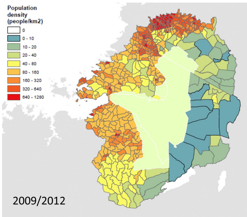
Fig. S3. Population densities for wards (Tanzania) and sub-locations (Kenya) within 60 km from the boundaries of the Core Protected Areas (CPA) 1999/2002 (top) and 2009/2012 (bottom).
