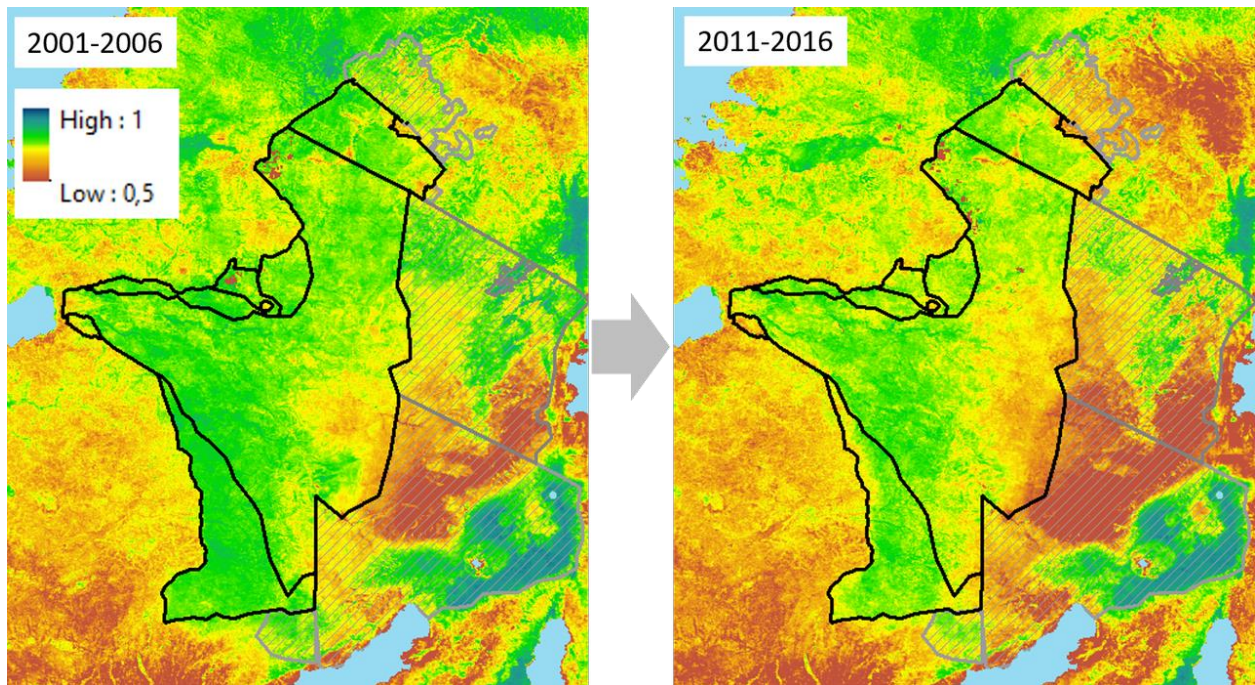
Fig. S9. Mean annual maximum NDVI for 2001-2006 (left) and 2011-2016 (right).
