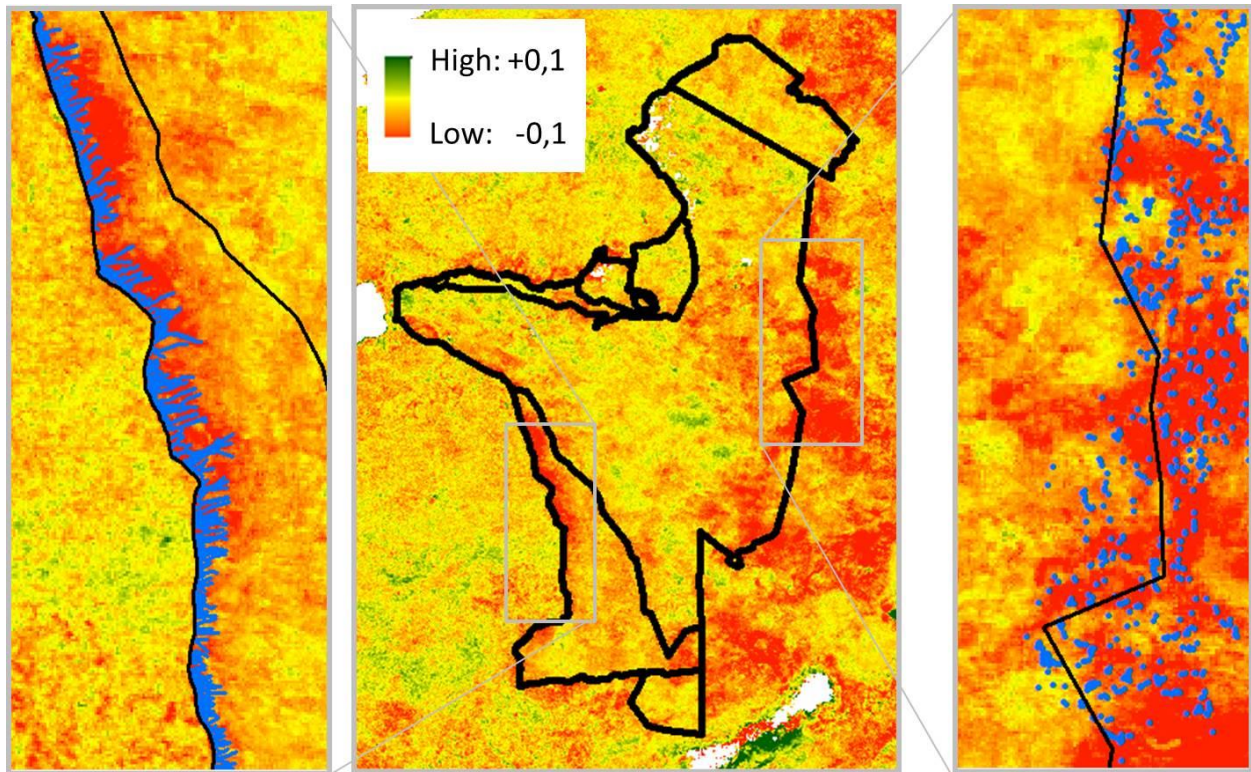
Fig. S10. Changes in mean maximum NDVI between 2001-2006 and 2011-2016. Enlargements of the border of Maswa Game Reserve overlaid with the livestock paths (left) and the Eastern border of the Serengeti National Park overlaid with mapped bomas (right).
