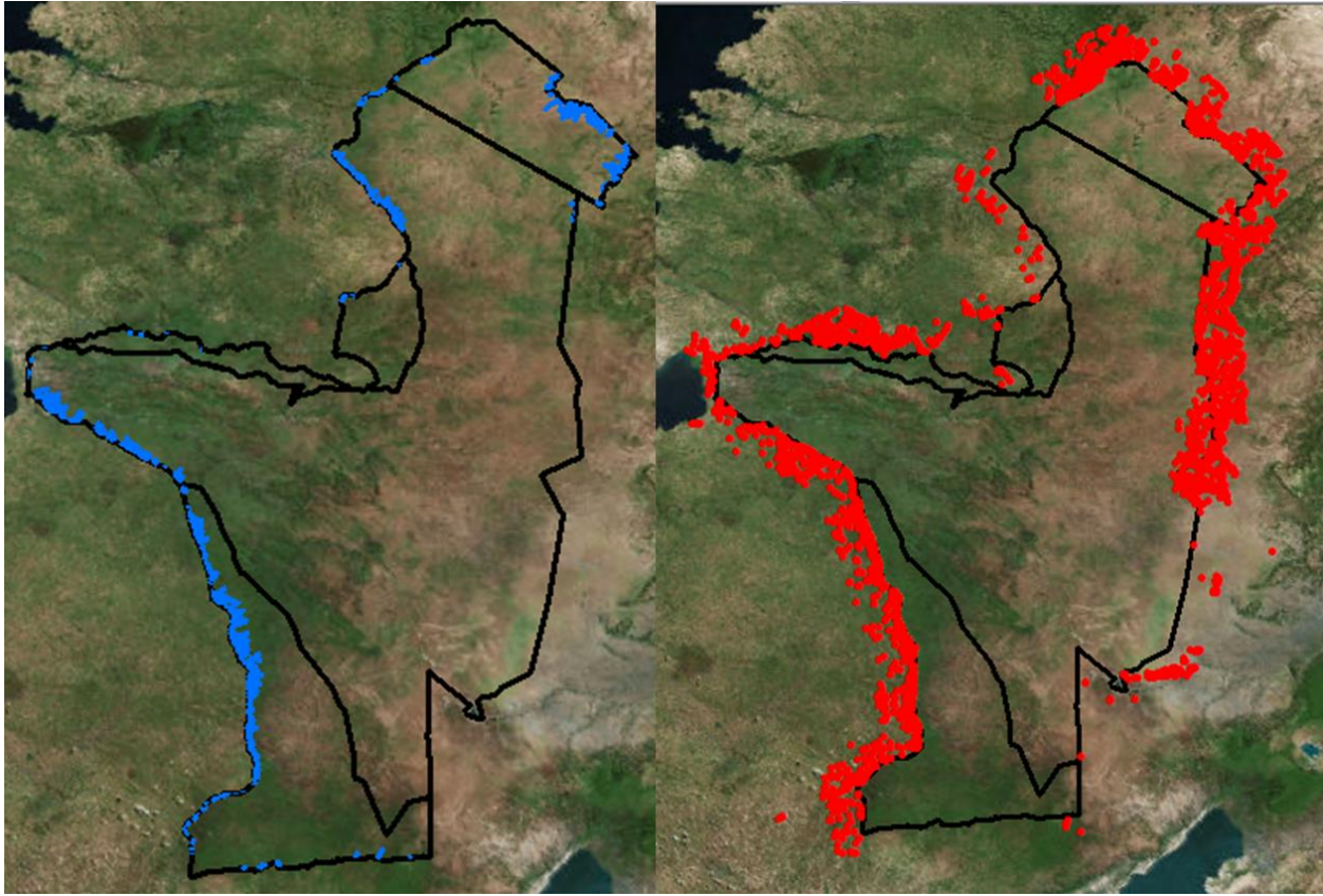
Fig. S22. Maps of livestock paths (left) and bomas (right). Livestock paths and bomas were identified using Google Earths Pro's (28 August 2017) (72).
