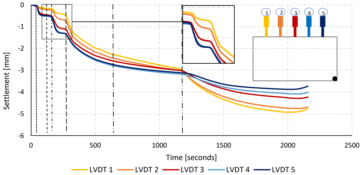
Figure 4-6: Soil surface settlement with time for GSI Test
