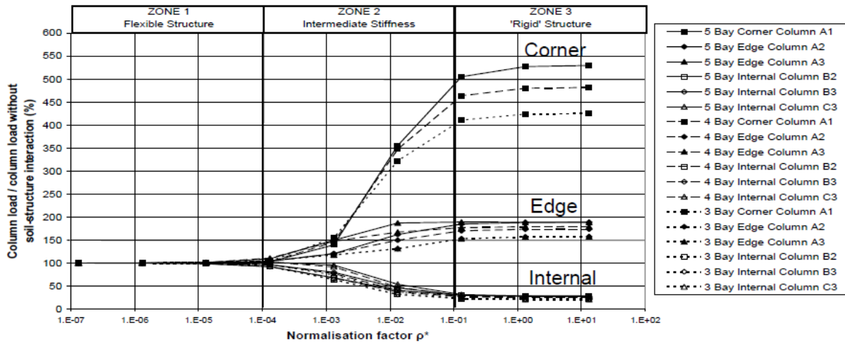
Figure 2-22: Structure normalisation (Smit and Clayton, 2011)
