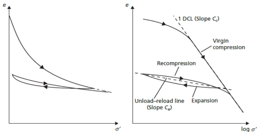
Figure 2-3: Void ratio-effective stress relationship (adopted from (Knappett and Craig, 2012))
