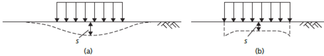
Figure 2-12: Distribution of vertical displacement beneath a flexible area: (a) clay and (b) sand (Knappett and Craig, 2012)
