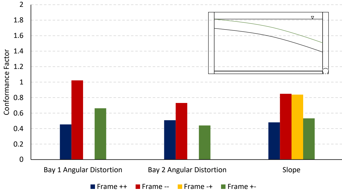
Figure 4-28: Deformation parameters at Max Differential Settlement
