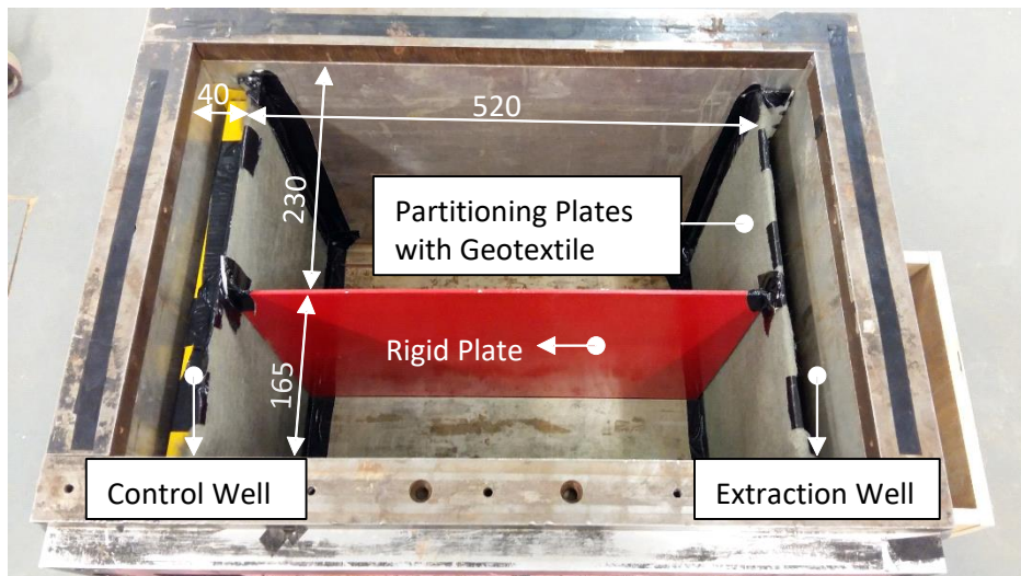
Figure 3-3: Centrifuge strongbox
