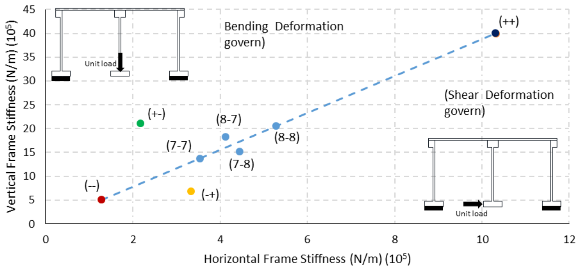
Figure 3-10: Vertical and horizontal frame stiffness
