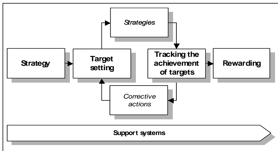
Figure 6: Implementation cycle
