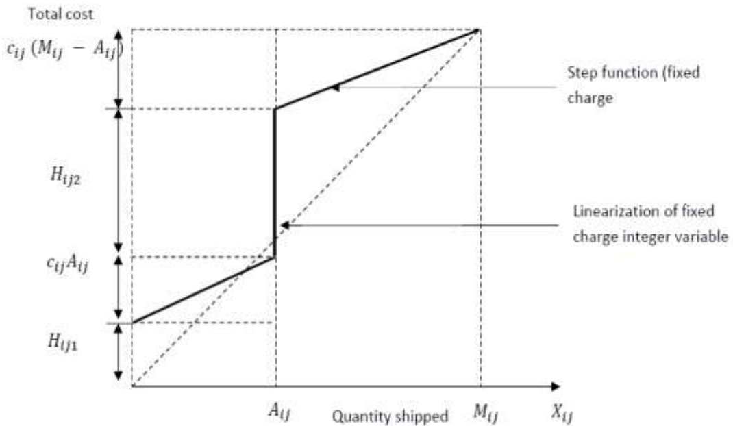
Fig. 2: Linearization and relaxation structure when H_{ij1} < H_{ij2}
