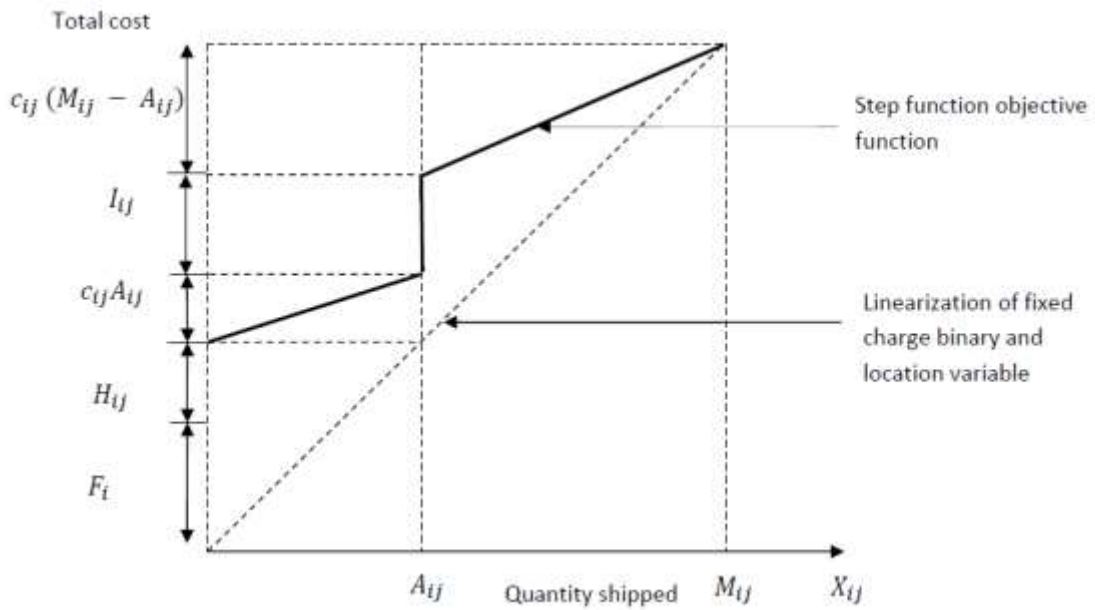
Fig. 1: Two-step linearization and relaxation Structure [5]
