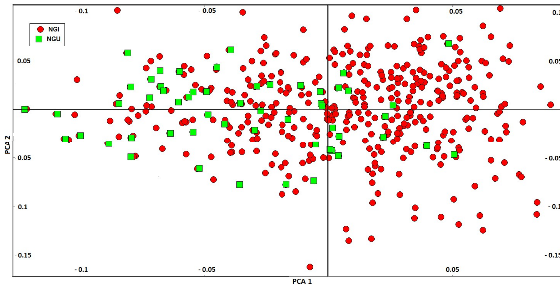
Figure 4: The clustering of samples from two Nguni populations (NGI and NGU) using the Nguni putative breed-specific SNPs.
