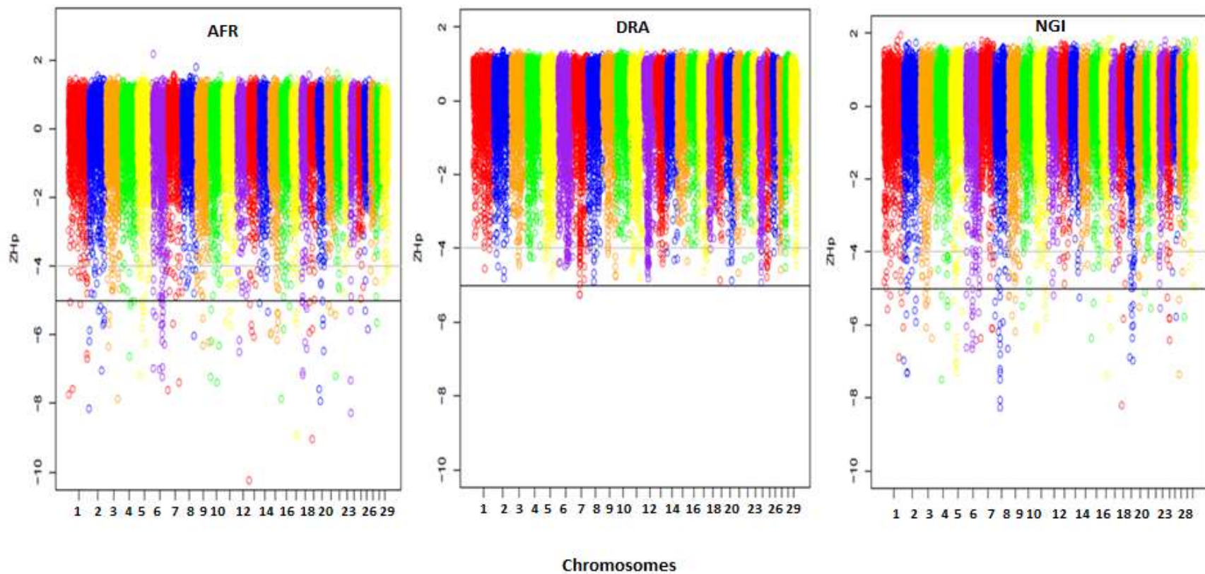
Figure 2: Distribution of Z Hp Z-scores across all 29 autosomes for Afrikaner (AFR), Drakensberger (DRA), and Nguni (NGI). The horizontal lines indicate Z Hp Z-score thresholds of -4 and -5 used to define candidate and putative selective sweep regions in this study.
