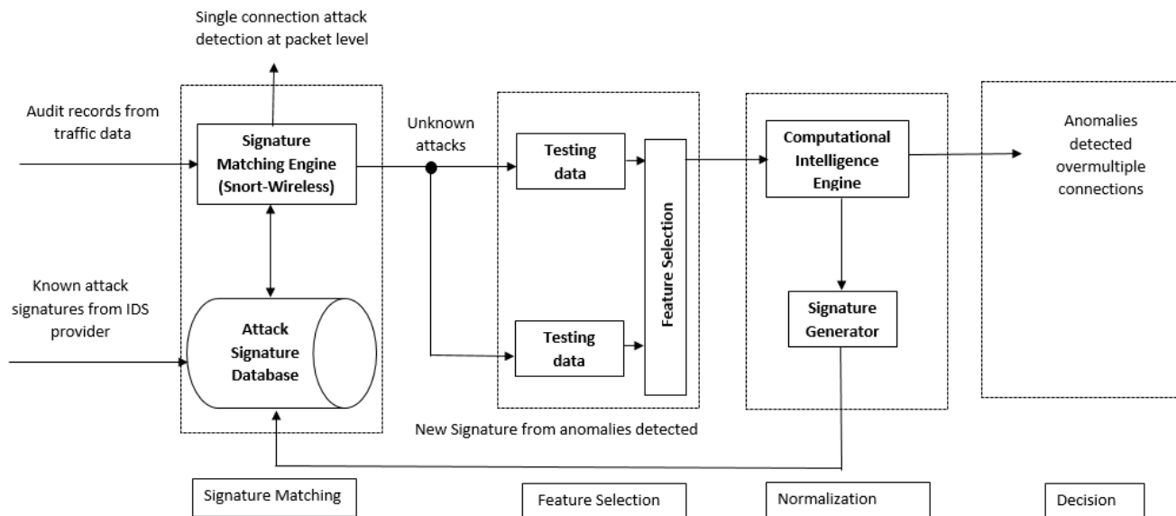
FIGURE 5. Intelligent intrusion detection and prevention system (IIDPS) architecture for WSNs (adapted from [69]).
