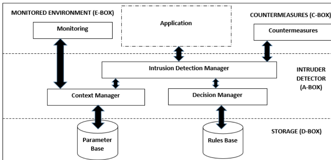
FIGURE 7. Logical architecture of danger theory immune-inspired IDS (adapted from [53]).
