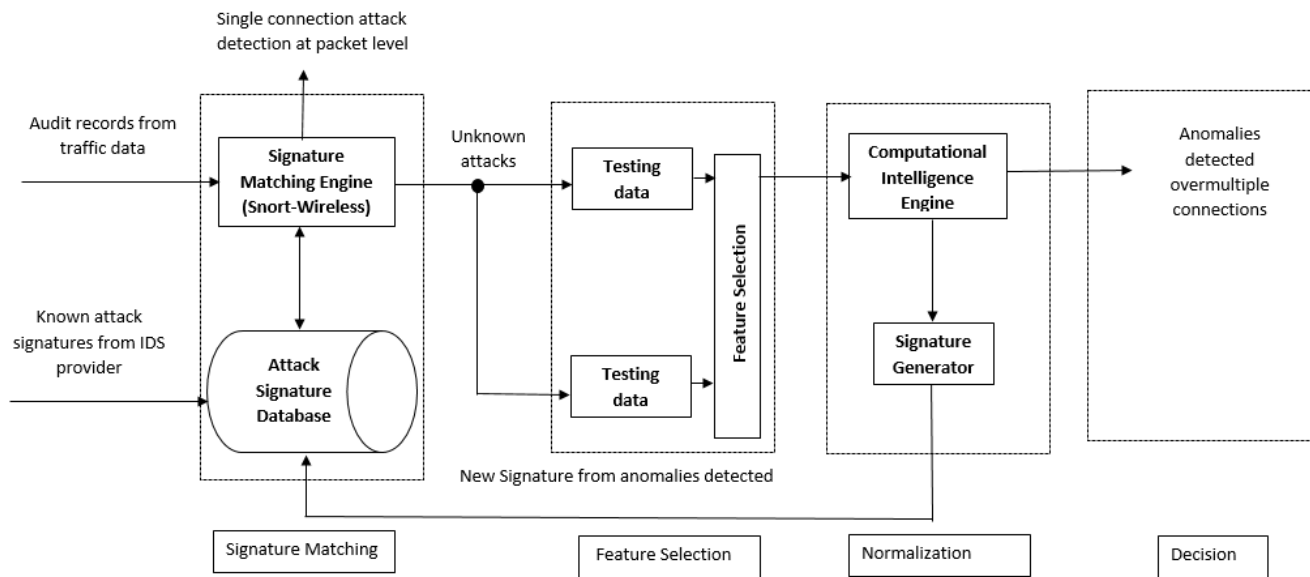
Fig. 5. Intelligent intrusion detection and prevention system (IIDPS) architecture for WSNs (adapted from [69])
