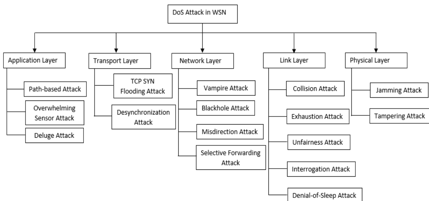
Fig. 3. DoS attack taxonomy in WSN
