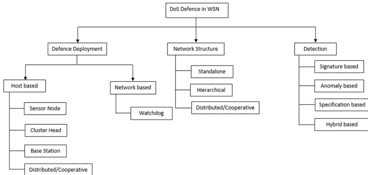
Fig. 4. DoS defence taxonomy in WSN
