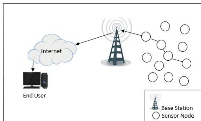
Fig. 1. Flat-based WSN topology
