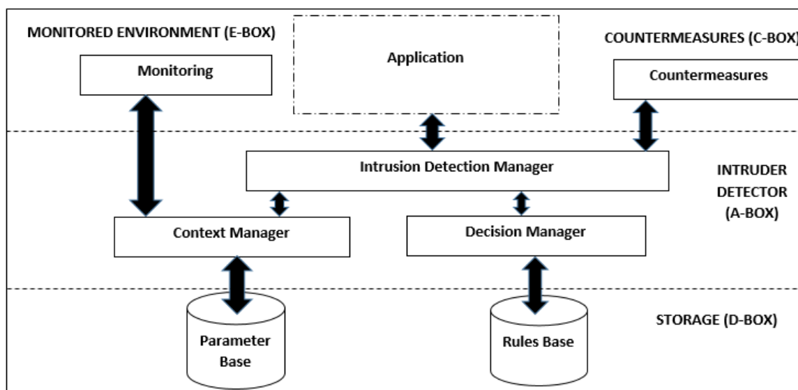
Fig. 7. Logical architecture of danger theory immune-inspired IDS (adapted from [53])
