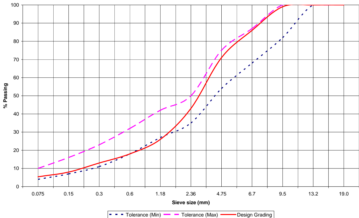
Figure 1 Grading Analysis of asphalt aggregate
