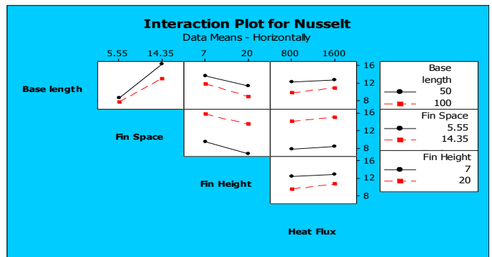
Figure 13 Interactions for heatsinks in the horizontal.
