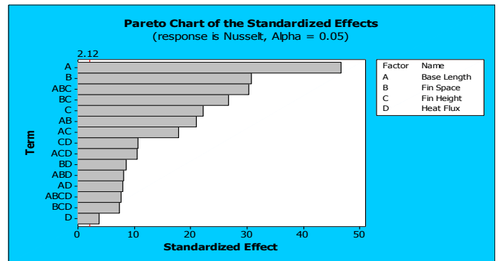
Figure 8 Pareto chart for heatsinks positioned vertically.
