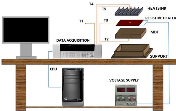
Figure 2 Arrangement of experimental bench
