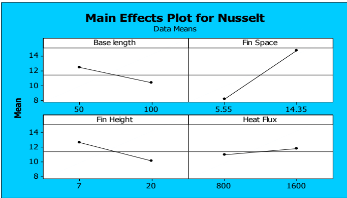
Figure 5 Main effects diagram for horizontal heatsinks.
