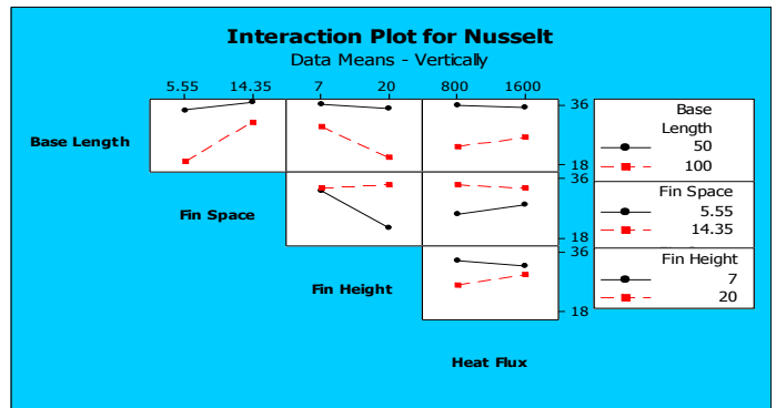
Figure 14 Interactions for heatsinks in the vertical.
