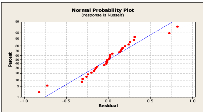
Figure 10 Normal probability plot for horizontal heatsinks.
