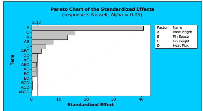
Figure 7 Pareto chart for heatsinks positioned horizontally.
