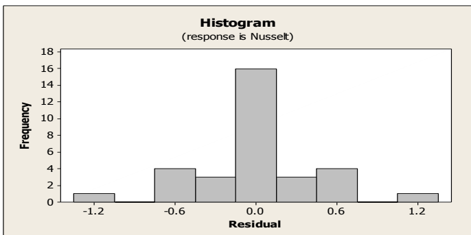
Figure 11 Residual histogram for vertical heatsinks.
