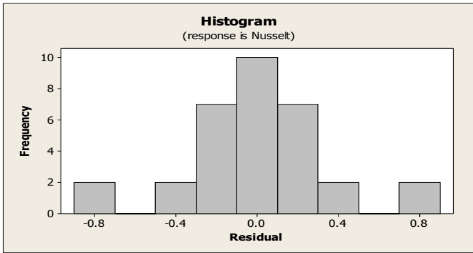
Figure 9 Residual histogram for horizontal heatsinks.
