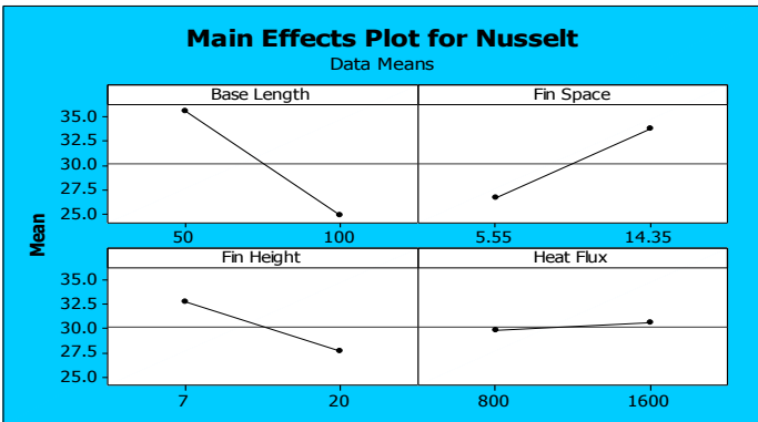
Figure 6 Main effects diagram for vertical heatsinks.
