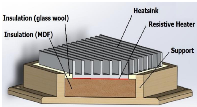
Figure 3 Assembly sectional view
