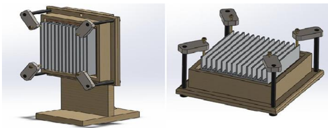
Figure 4 Vertical and horizontal settings
