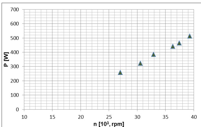
Figure 8 Power characteristics of turbogenerator 2nd stage with load resistance of 131 \Omega
