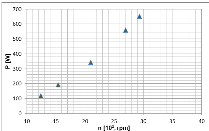
Figure 7 Power characteristics of turbogenerator 1st stage with load resistance of 60 \Omega
