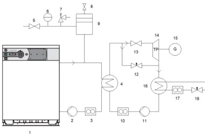
Figure 1 Schematic of the laboratory installation; 1- gas boiler, 2- oil circulation pump, 3- oil flow meter, 4- evaporator, 5,8,13,18- ball valve, 6- manometer, 7- safety valve, 9- compensation vessel, 10- mass flow meter, 11- pump of working fluid, 12- throttle valve, 14- expander, 15- alternator, 16- condenser, 17- water flow meter,
