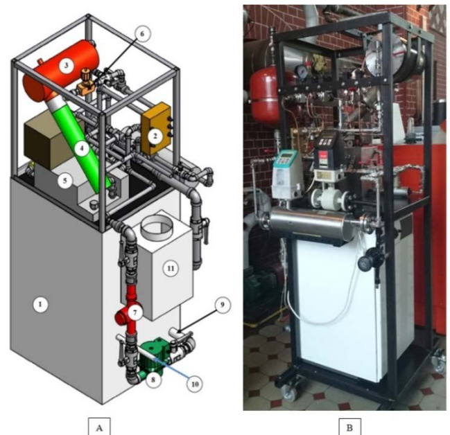
Figure 2A) Micro-CHP – axonometric view: 1- gas boiler, 2- evaporator, 3- turbogenerator, 4- condenser, 5- tank with ethanol, 6- throttle valve, 7- oil flow meter, 8- oil circulating pump, 9- inlet oil, 10- gas connector, 11- exhaust, B) overview of micro-CHP with gas boiler
