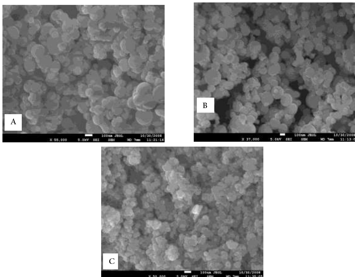
Fig. 1. SEM images of three silica NMs with different average particle sizes. (A) Silica fume (100-400) nm; (B) Calcined silica fume (50-300) nm; and (C) Precipitated silica (20-100) nm.
