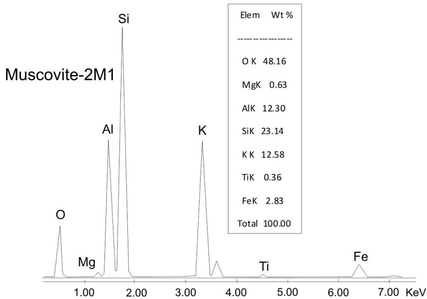
Fig. 7. Analytical data of the tubular microfossils from the Neoproterozoic Omdraavlei Formation. SEM/EDS analyses of a fragment of mineralized tube-like microfossil (SEM/BSE at the top) showing different elemental composition of the mineral cell coating and the mineralized internal strand. Two aluminosilicate phases are identified stoichiometrically: one close to Mg chamosite (blue frame on top image) and the other suggestive for muscovite (yellow frame on top image). Sample SA2-178. Scale bar equals 50 \mu\text{m} .
