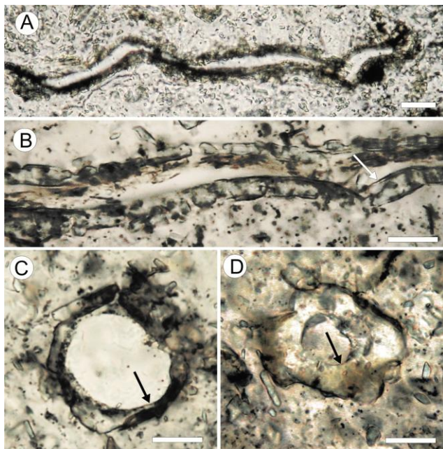
Fig. 4. Optical micrographs of siphonous microalgae-like tubular microfossils from the Neoproterozoic Omdraavlei Formation. (A) Elongated fragment of mineralized siphonous thalli-like microfossil in longitudinal axial section. (B) Slightly magnified fragment of thallus in longitudinal section showing the blocky and/or granular character of silicate material forming the coating on the cell wall (arrow). The carbon-enriched, striated internal silicate strand, which fills not entirely the tube interior and can be interpreted as remain of shrunken cell content. (C-D) Cross sections fragments of externally rough mineralized tubular thalli showing smooth internal surface of the crystalline mineral coating delimiting the position of the former cell wall (arrows). The tube mineral coatings are in part composed of blocky silicate crystals, and in part of almost homogenous silicate material with various admixture of fine kerogenous matter. Scale bars: (A), 50 \mu\text{m} ; (B-E), 30 \mu\text{m} . All from sample SA-31.
