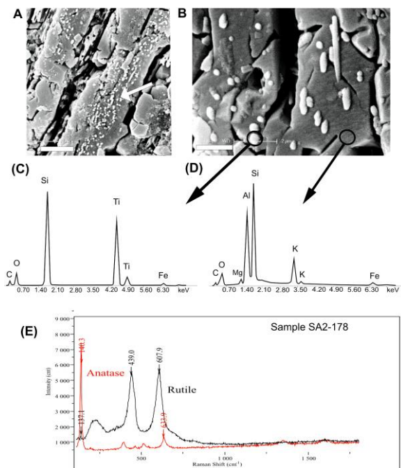
Fig. 9. HF-etched mineral coatings of tubular microfossils from the Neoproterozoic Omdraivlei Formation with embedded fossils of mineralized bacteria-like structures. (A and B) SEM images of longitudinal sections of HF-etched thick mineral (Al-silicate) coating of Omdraivlei Fm. microfossils with numerous minute whitish bodies exposed by etching (arrowed). The bodies in higher magnification (B) are identifiable as remains of mineralized rod-like and coccoid bacteria-like structures. (C and D) Elemental electron dispersive spectra (SEM/EDS) of the same mineral coating; in contrast to the titanium-rich bacteria-like bodies (C), the bulk of the mineral coating shows Al-K-Mg-Fe-silicate composition (D). (E) Raman spectra suggest mixture of anatase and rutile for the titanium-rich bacteria-like objects. Scale bars: (A), 5 µm; (B), 2 µm. Sample SA2-178.
