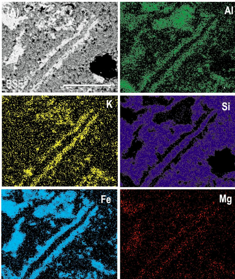
Fig. 6. Analytical data of the tubular microfossils from the Neoproterozoic Omdraavlei Formation. Energy Dispersive Spectroscopy (SEM/EDS) maps showing distribution of elements in a fragment of matrix embedded mineral tubes imaged as SEM/BSE in panel (A). Sample S2-31. Scale bar for all equals 100 \mu\text{m} .
