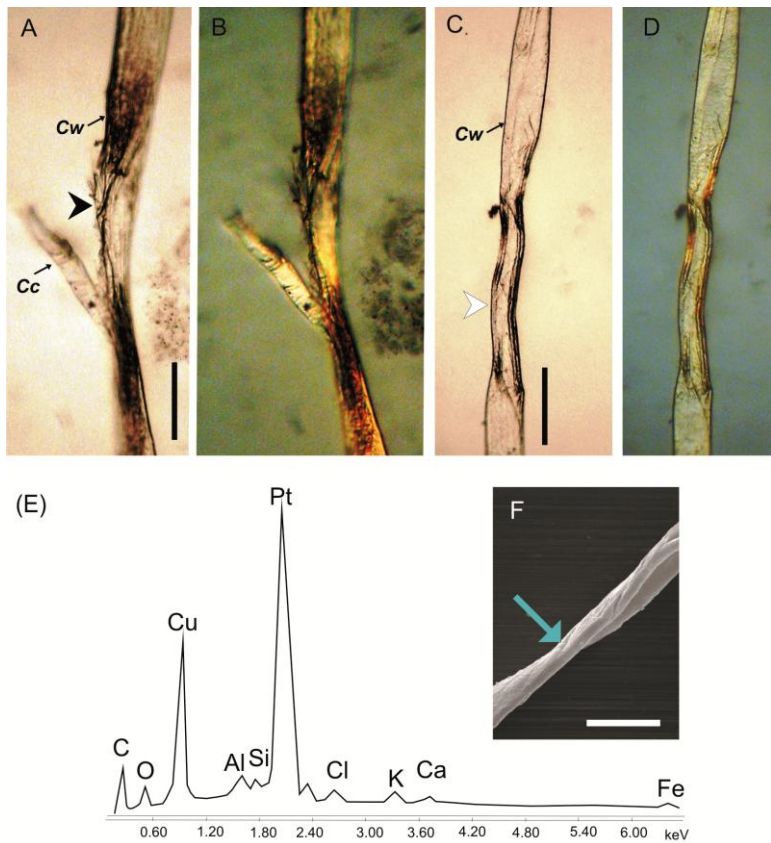
Fig. 11. Tubular microfossils from the Neoproterozoic Omdraivlei Formation reminiscent of modern siphonous microalgae. (A-D) Optical micrographs of fragments of HF-macerated tubular microfossils imaged in plain (A and C) and polarized (B and D) light. Polarization reveals traces of permineralization preserved in the macerates. Cw – cell wall, Cc – remains of shrunken and detached from the cell wall epiparietal protoplast. Arrow heads indicate mechanical ruptures in cell walls caused either by maceration procedure (A and C) or early diagenetic degradation processes (?dehydration). (E and F) SEM/EDS spectrum (G) of a fragment of macerated tubular microfossil (H), analyzed on Cu-band and sputtered with Pt, shows the presence of C and elements typical for silicate minerals. Scale bars for all 50 \mu\text{m} . Sample SA2-178.
