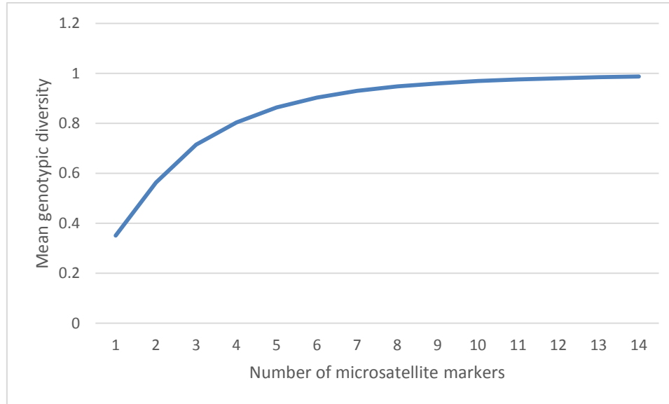
Suppl. Fig. 1. Mean genotypic diversity plotted against the number of microsatellite markers, which shows a plateau at 12 markers.
