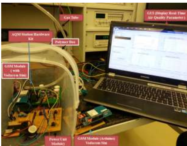
Fig. 8 (a & b). Calibration setup and control cross sensitivity or interfering gases setup.
