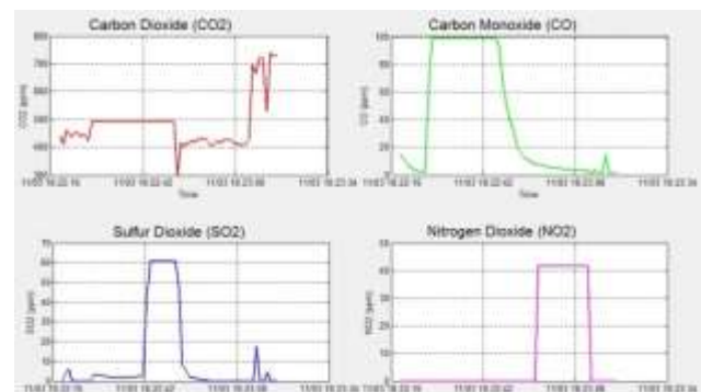
Fig. 10. On-line data updating on GUI based on Real-time measurements of greenhouse gases.
