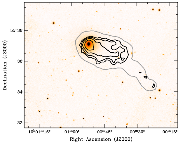
Figure 7. Integrated H I image of NGC 3073 showing the full extent of the two tails of NGC 3073. Black contour levels are at 3, 5, 10, 20, 50, 100 \times 10^{19} \text{cm}^{-2} ( 45'' \times 48'' resolution), and the grey contour level is 1.5 \times 10^{19} \text{cm}^{-2} ( 78'' \times 80'' resolution).
