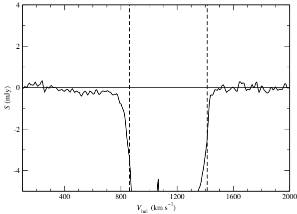
Figure 3. A zoom-in plot of the H I absorption. The vertical line represents the systemic velocity. The dashed lines represent the velocity range of the H I emission as indicated in Fig. 2.
