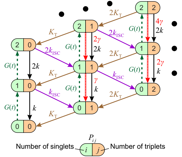
Fig. 5 Stochastic model of S-T annihilation. Color ovals represent various possible states of the system containing different numbers of singlets and triplets. The probability of each state is P_{i,j} and arrows demonstrate possible transition between these states. k and K_{\text{T}} are the relaxation rates of singlet and triplet states, respectively; k_{\text{ISC}} is the rate of inter-system crossing; \gamma is the rate of S-T annihilation; and G(t) denotes the generation rate of singlet states. The black dots indicate that the model can be further extended to higher numbers of singlet and triplet states.
