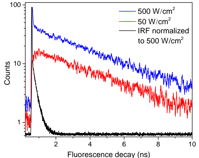
Fig. 1 Fluorescence decay traces of a single LHCII complex at different excitation intensities of 50 (red line) and 500 W/cm 2 (blue line). The black line indicates the instrument response function (IRF) with a full width at half-maximum of 38 ps.
