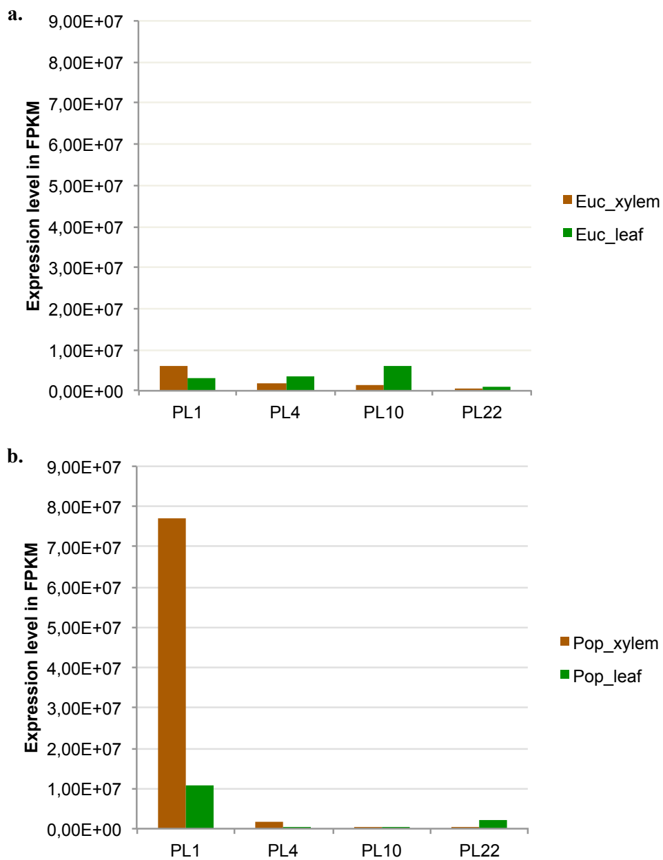
Figure S9 Comparative expression patterns of PL domain families in E. grandis and P. trichocarpa .
