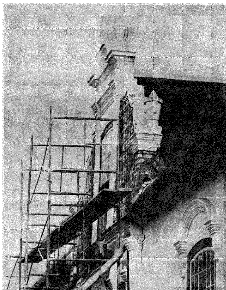
Dangerous disintegration was halted after step-by-step repair programme. Strengthening mesh and tie rods were placed unobtrusively in undecorated areas.
