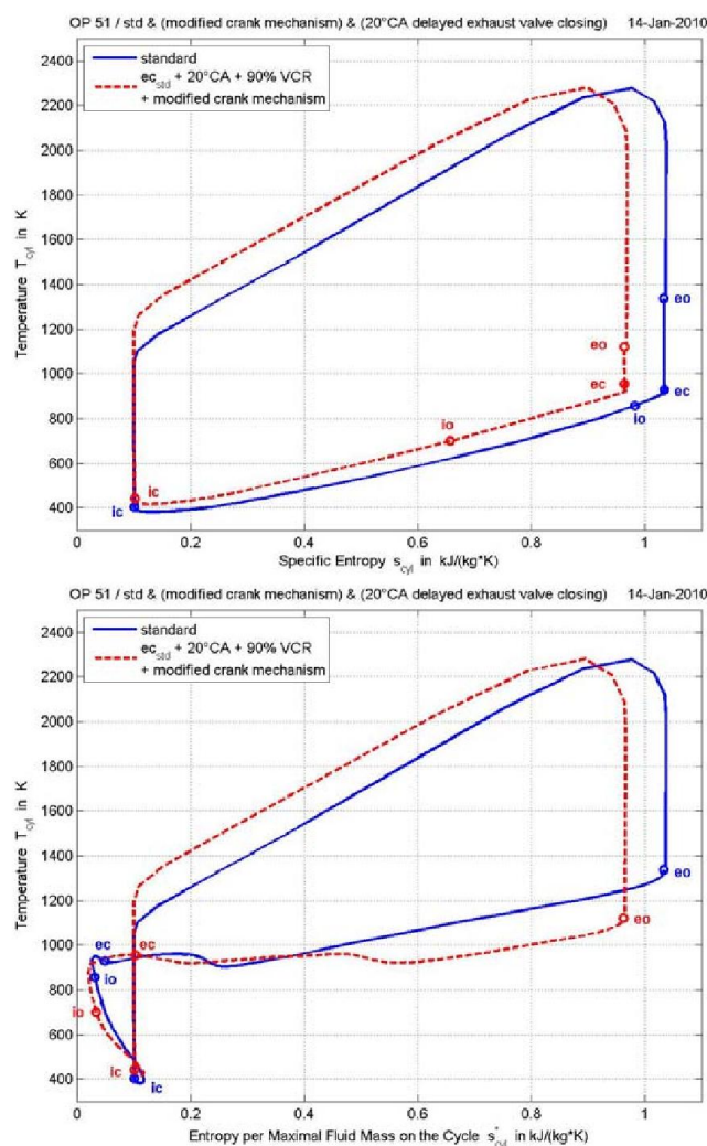
Figure 17. Temperature – Specific Entropy (T,s) [4] and Temperature – Entropy per Max. Fluid Mass diagrams (T,s*)
