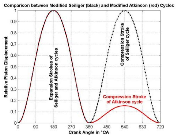
Figure 15b. Relative Piston Displacement – CA Diagram for a very high pressure supercharged engine [8]. The intake and compression strokes are very much shorter than expansion and exhaust strokes
