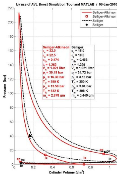
Figure 11. Pressure - Volume Diagrams of standard Seiliger and 2V-TC Atkinson Cycles
