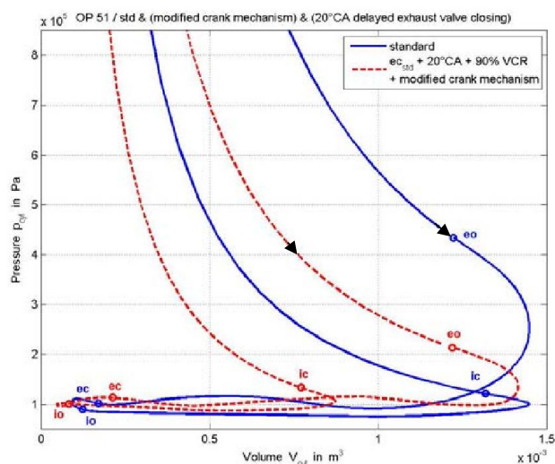
Figure 16. Pressure – Volume Diagram [4]
