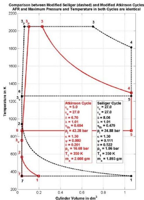
Figure 22. Temperature–Volume Diagram of V,p,T–Seiliger and –Atkinson Cycles
