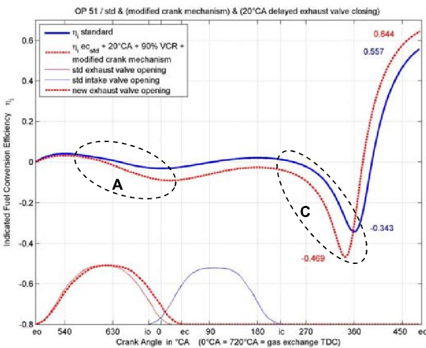
Figure 19. IFCE – Crank Angle Diagram [4]
