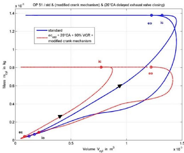
Figure 18. Fluid Mass – Volume Diagram [4]
