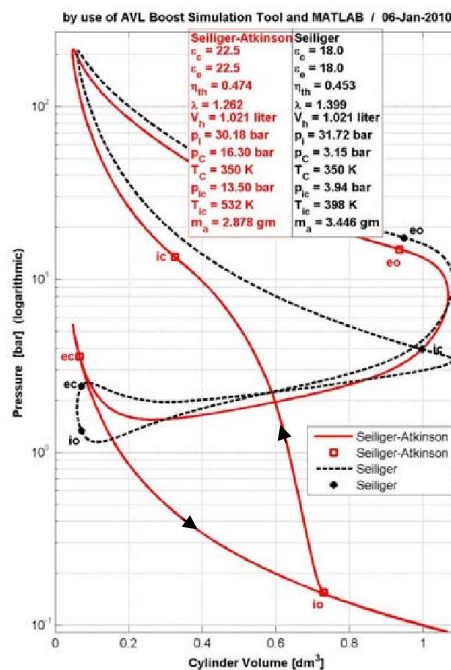
Figure 12. Pressure (logarithmic) - Volume Diagrams of standard Seiliger and 2V-TC Atkinson Cycles
