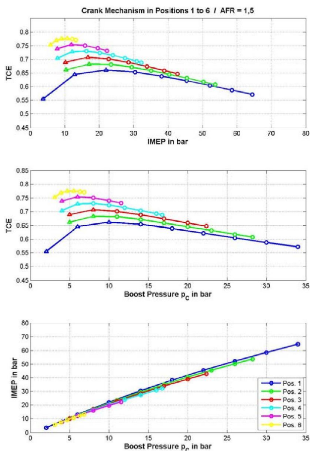
Figure 30. Correlation between TCE, IMEP, Boost Pressure and Crank Mechanism Positions at Full and many Part Loads with AFR = 1.5
