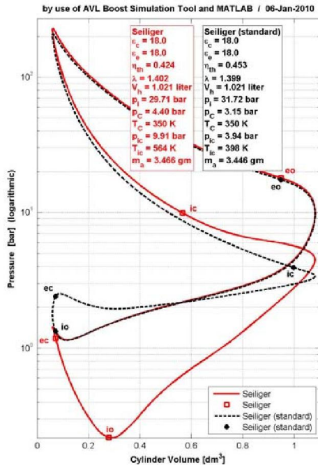
Figure 7. Pressure (logarithmic) – Volume Diagram of Seiliger (standard) and Atkinson (Seiliger Cycle with 60°C Delayed Suction = 1V-TC) Cycles
