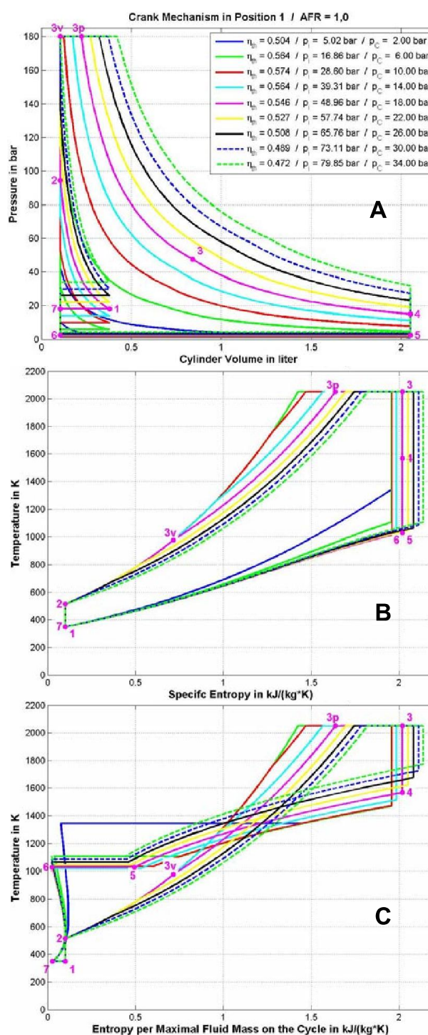
Figure 27. Simulated Ideal V,p,T Atkinson Cycles for the Crank Mechanism in Position 1 (see Fig. 26) at Full and many Part Loads with Stoichiometric AFR. A represent Pressure-Volume (p,V), B Temperature-Specific Entropy (T,s) and C Temperature-Entropy per Max. Fluid Mass diagrams (T,s*)
