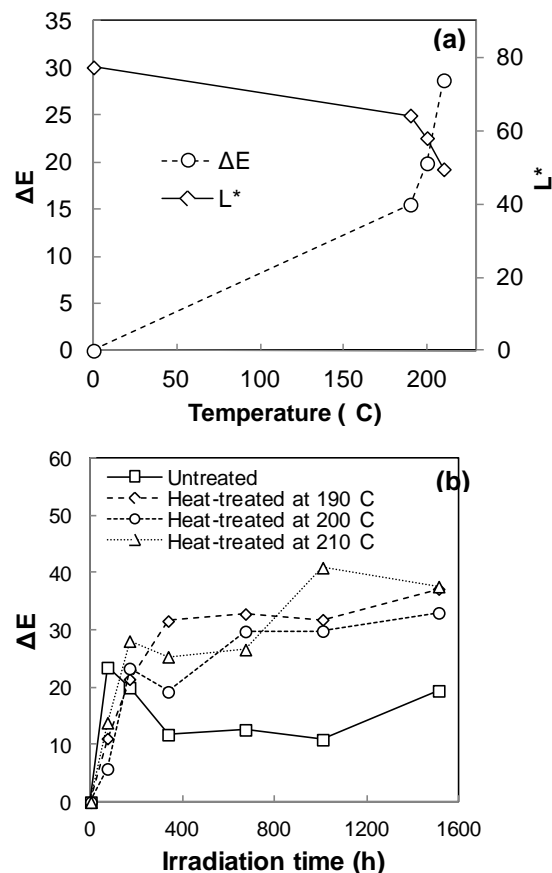
Figure 1 Color changes of heat-treated jack pine reported using CIE- L^*a^*b^* system: (a) total color difference ( \Delta E ) and lightness ( L^* ) during heat-treatment, (b) \Delta E during artificial weathering
