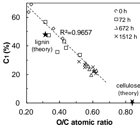
Figure 5 Correlation of the O/C atomic concentration ratio with the percentage of C 1 carbon for heat-treated jack pine
