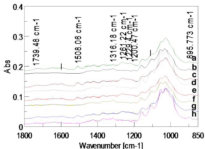
Figure 4 FTIR spectra of heat-treated jack pine before and after weathering for 1512 h: (a) untreated before weathering, (b) untreated after weathering, (c) heat-treated at 190°C before weathering, (d) heat-treated at 190°C after weathering, (e) heat-treated at 200°C before weathering, (f) heat-treated at 200°C after weathering, (g) heat-treated at 210°C before weathering, (h) heat-treated at 210°C before weathering
