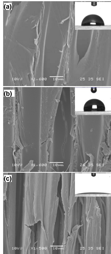
Figure 3 SEM image and initial contact angle of heat-treated jack pine surface: (a) untreated before weathering, (b) heat-treated at 210°C before weathering, (c) heat-treated at 210°C after weathering of 1512 h
