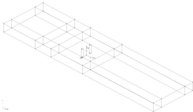
Figure 2 Isometric view of the computational domain
