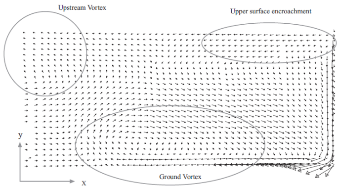
Figure 5 SRANS: jet plane velocity vectors (left jet)
