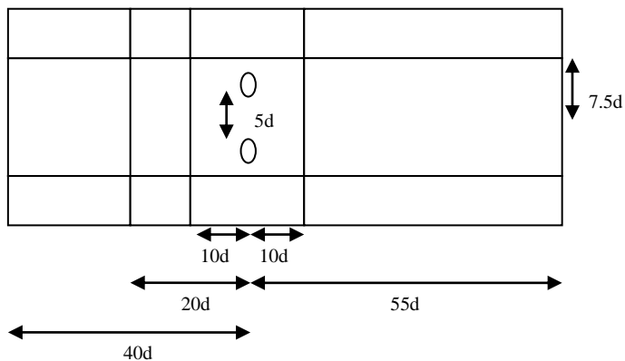
Figure 1 Top view of the computational domain
