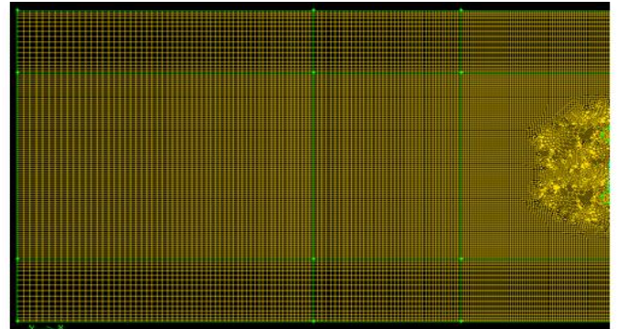
Figure 3 Top view of the mesh
