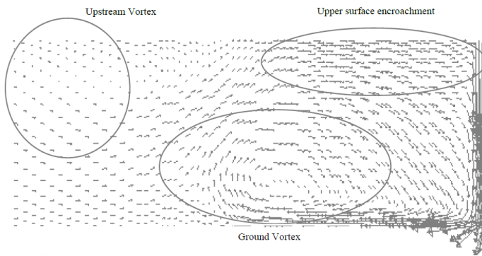
Figure 4 URANS: jet plane velocity vectors (left jet)
