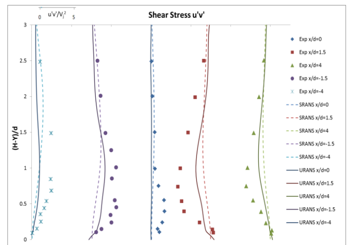
Figure 7 Comparison between the predicted shear stress and the experimental data
