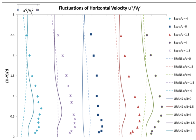
Figure 8 Comparison between the predicted streamwise normal stress and the experimental data
