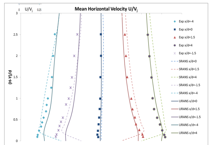
Figure 6 Comparison between the predicted velocity profiles and the experimental data
