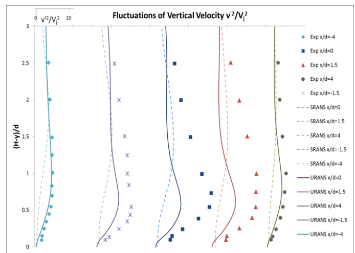
Figure 9 Comparison between the predicted vertical normal stress and the experimental data
