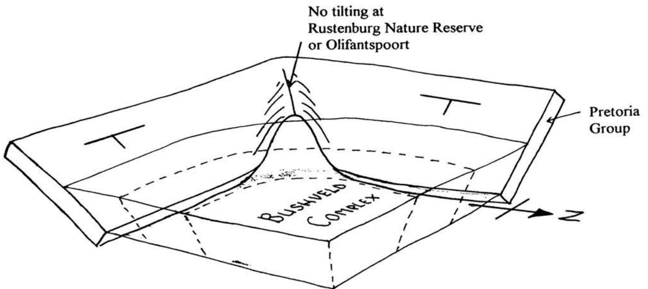
Figure 4.7: Schematic drawing showing why areas at corners of the Transvaal basin may fail to be accommodated during thermal collapse of the Bushveld Complex.
