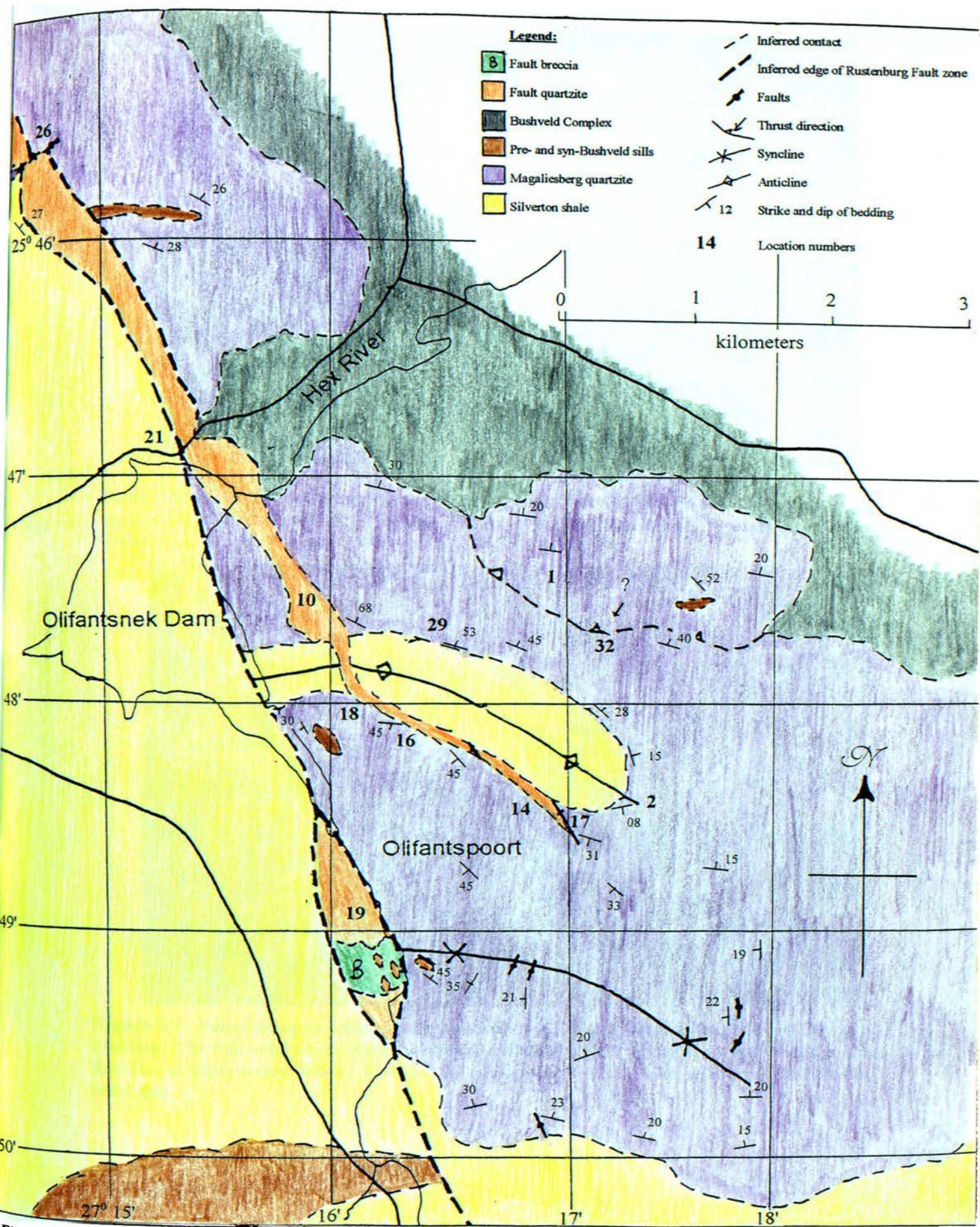
Figure 3.5: Detailed geological map of the Olifantspoort area, showing curved fold axial traces, and tightened folding on the anticline.
