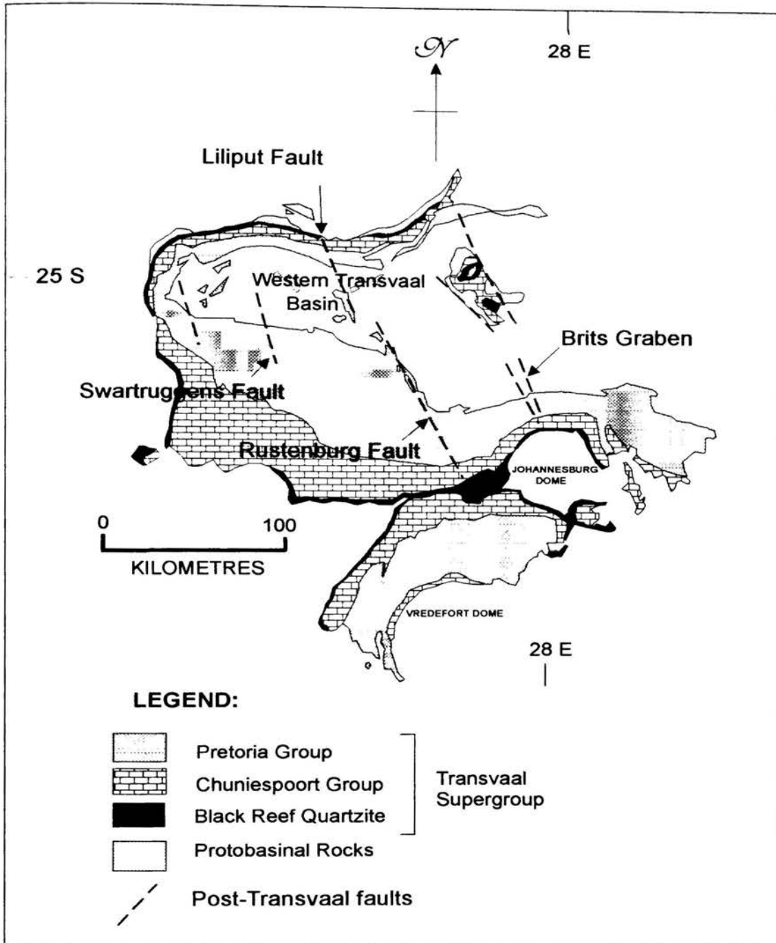
Figure 4.1: Parallel post-Transvaal Supergroup faults in the western Transvaal basin ( after Dietvorst, 1991).
