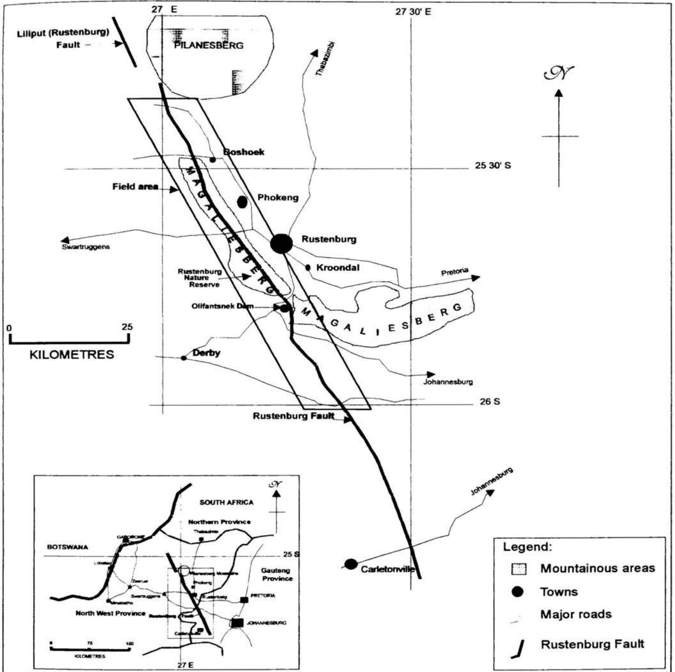
Figure 1.2: Location of the field area.
