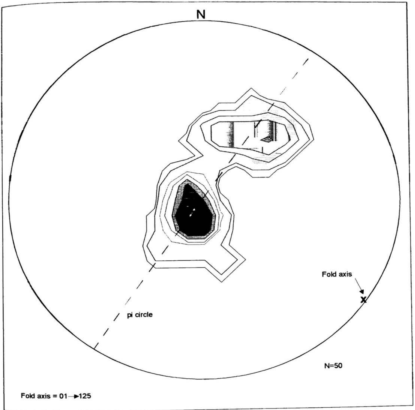
Figure 3.12: Stereographic projection of the density distribution of poles to bedding in the Rustenburg Nature Reserve syncline. Fold axis plunges 01 → 125.
