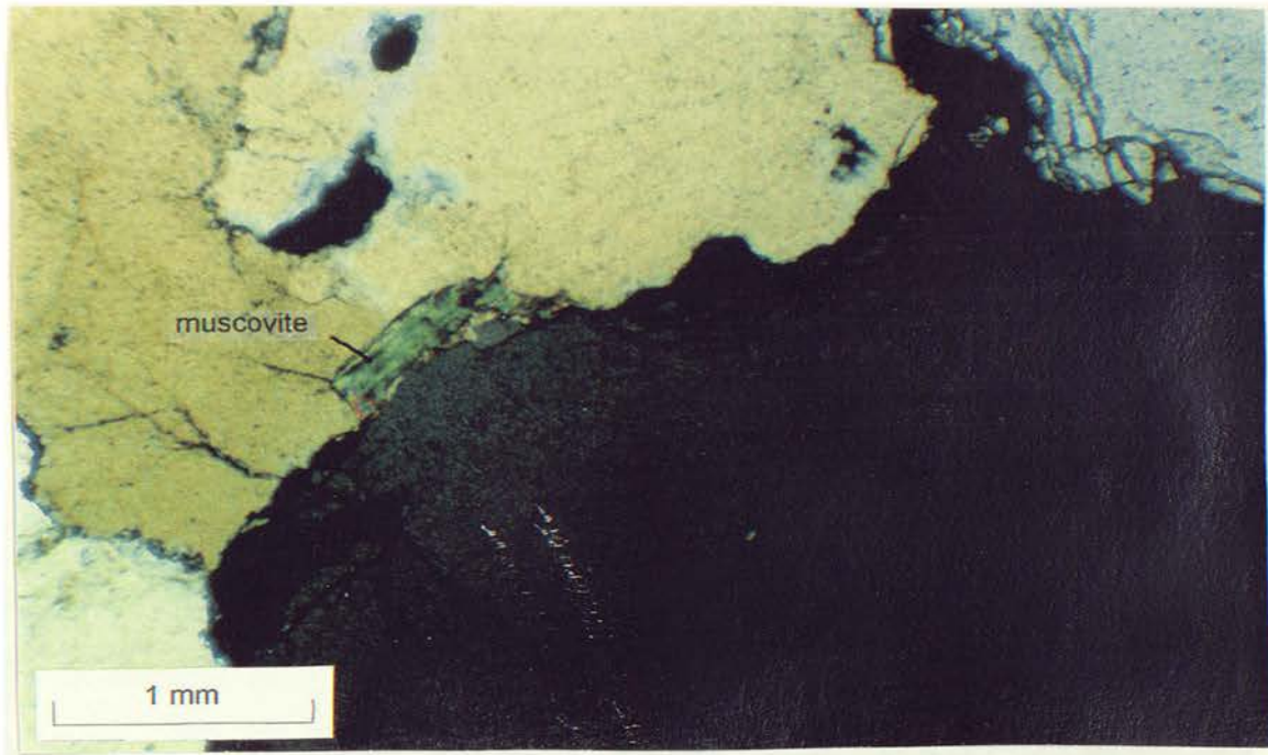
Figure 2.16: Photomicrograph of very coarsely recrystallised Magaliesberg quartzite from 25° 47.52' S; 27° 17.12' E. Note lack of inclusions in quartz crystals and rare muscovite (crossed poles).
