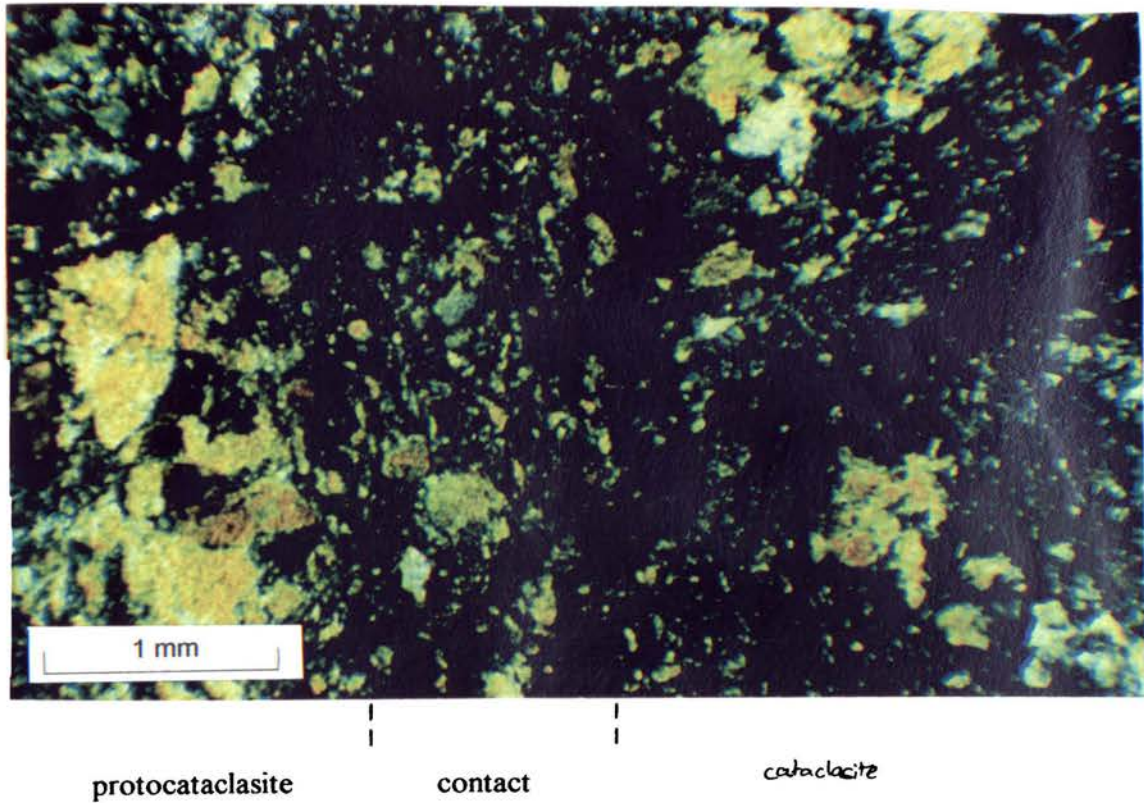
Figure 3.47: Photomicrograph of protocataclasite from location 36, showing larger quartz grains in protocataclasite, grading into cataclasite in the centre.
