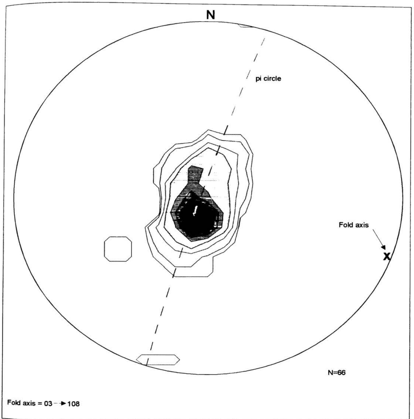
Figure 3.14: Stereographic projection of the density distribution of poles to bedding in the Magaliesberg quartzite in the partially fault-bounded area between Olifantsnek dam and the synclinal fold axis (location 9) in Rustenburg Nature Reserve. Fold axis plunges 03 -> 108.
