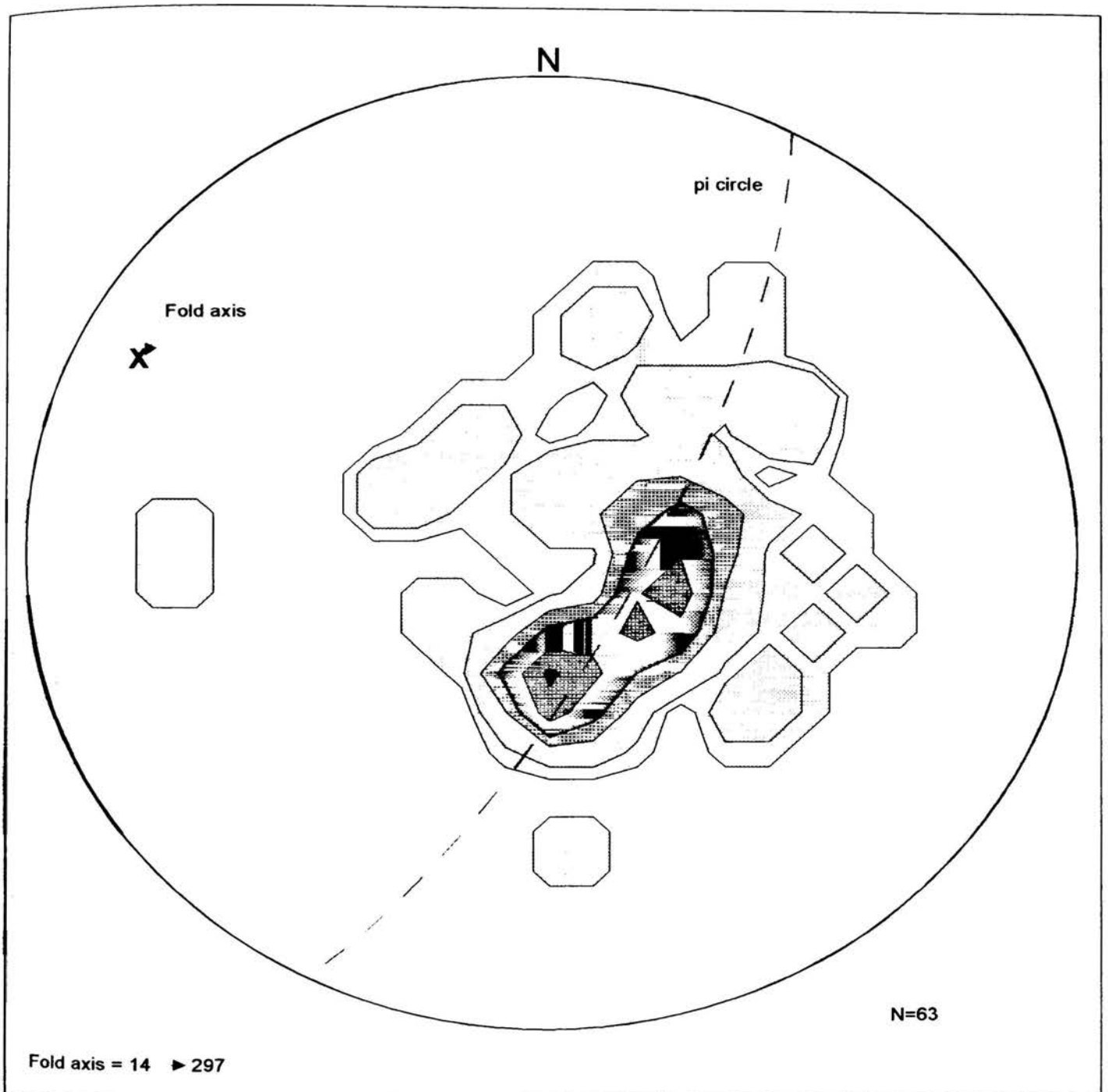
Figure 3.10: Stereographic Projection of the density distribution of poles to bedding in the Olifantspoort syncline. Fold axis plunges 14 ▶ 297.
