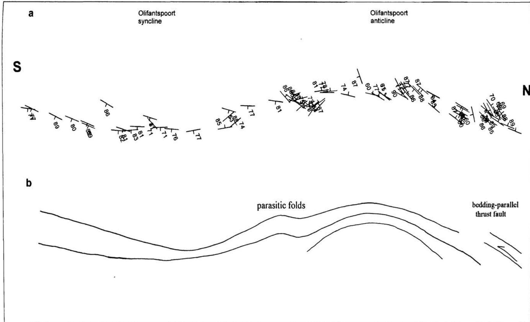
Figure 3.17: a.: Down-plunge projection of the Olifantspoort folds. The variable nature of the dips around vertical results from the curved fold axial surfaces.
