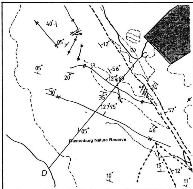
Figure 4.3: Locations of cross-sections constructed in Figure 4.2.
