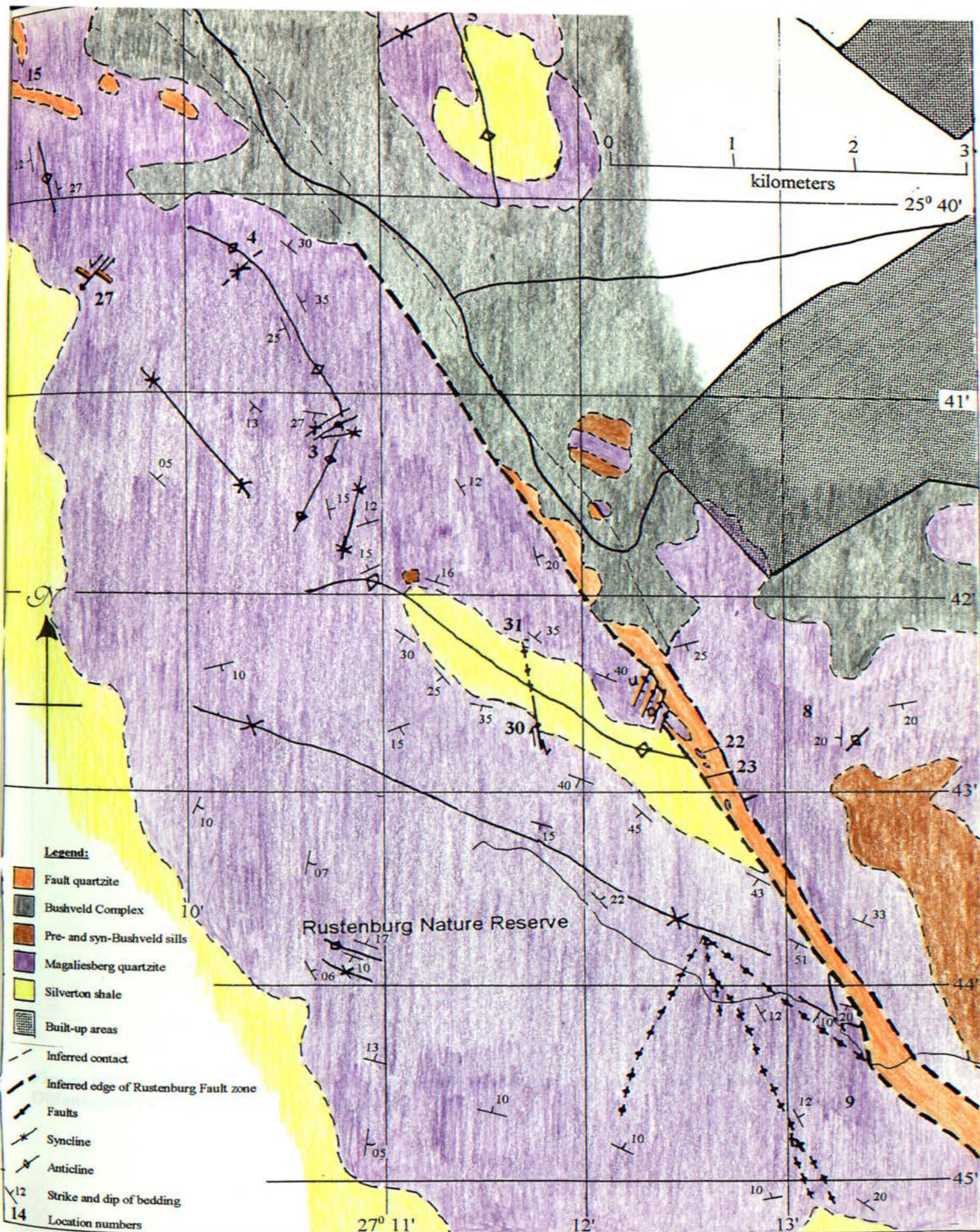
Figure 3.8: Detailed geological map of the Rustenburg Nature Reserve area, showing curved fold axial traces, and tightened folding on the anticline.
