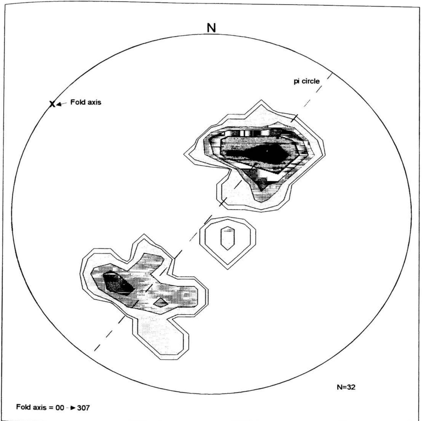
Figure 3.11: Stereographic projection of the density distribution of poles to bedding in the Rustenburg Nature Reserve anticline. Fold axis plunges 00 -> 307.
