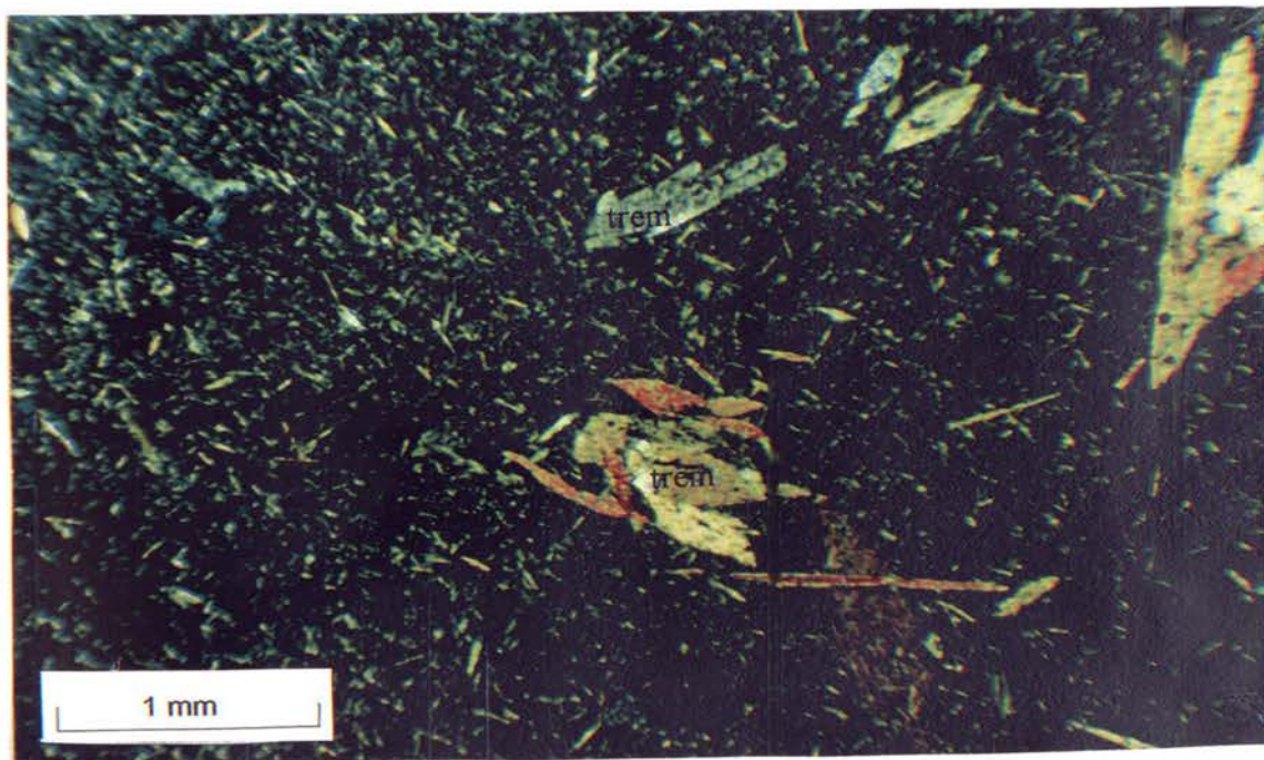
Figure 2.19: Photomicrograph of meta-diabase consisting of needles of tremolite, and glomerocrysts of tremolite at 25° 55.60' S; 27° 20.50' E (crossed poles).
