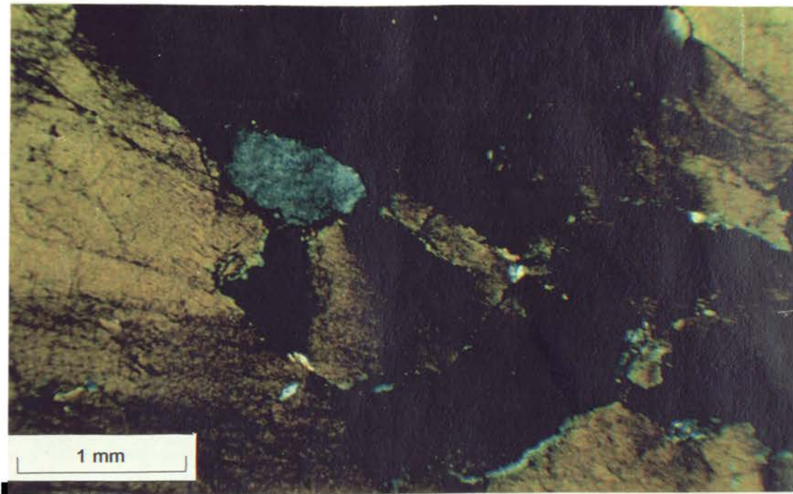
Figure 3.24: Photomicrograph showing undulose extinction in Fault quartzite from location 14.
