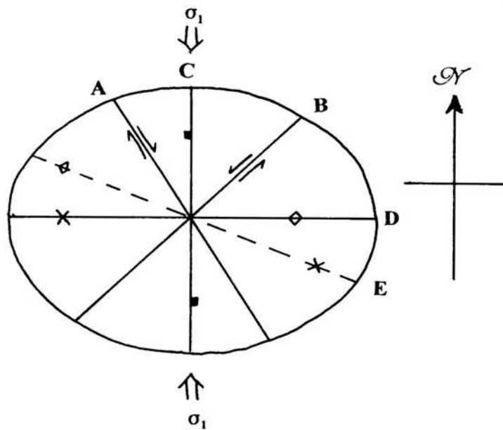
Figure 4.5: Model for the creation of en-échelon folds and sinistral conjugate faults by dextral shear in the Rustenburg Fault.
