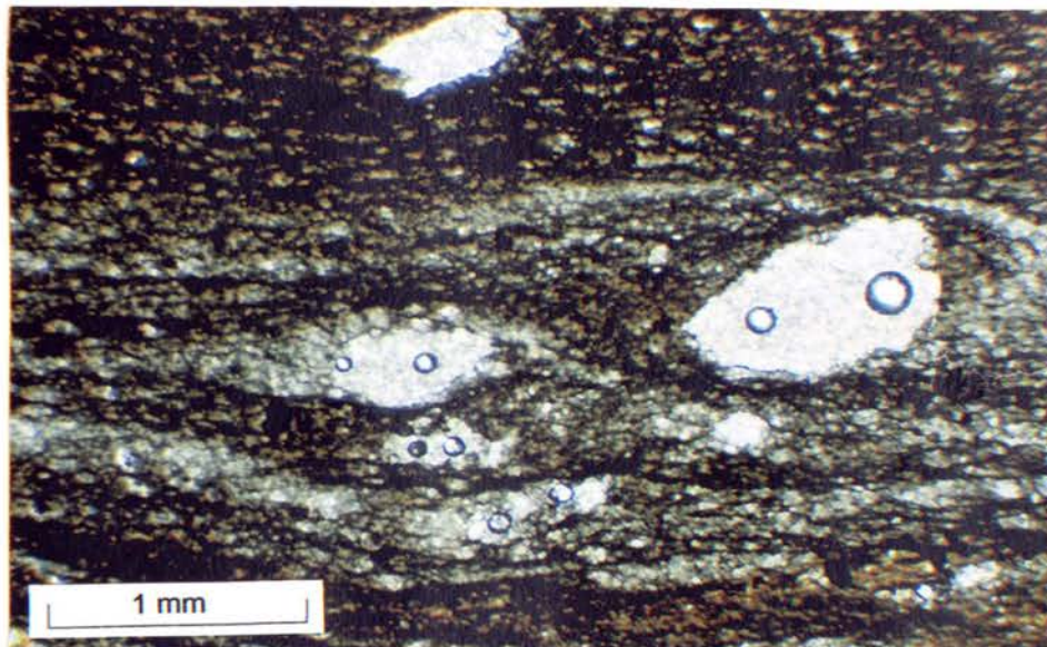
Figure 3.50: Photomicrograph from location 37. Slaty cleavage has developed, with mica-rich domains typically anastomosing around either silt lenses or lenticular metamorphic minerals, which have now weathered out (voids are filled with Canada balsam during section preparation). The lenses have developed quartz overgrowths, and are aligned parallel to the orientation of the cleavage plane.
