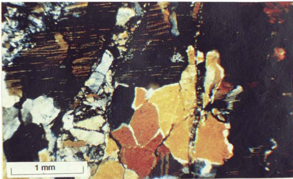
Figure 3.32: Photomicrograph showing brecciation of Fault quartzite (from location 19).
