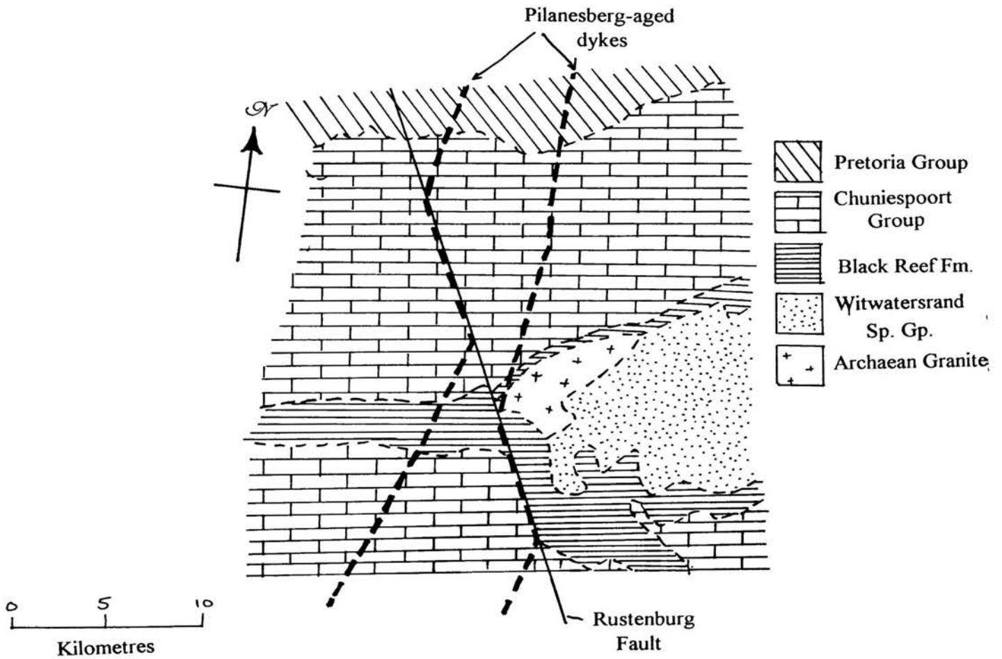
Figure 4.8: Exploitation of the Rustenburg Fault by Pilanesberg-aged dykes, rather than displacement (after Meadon, 1973).
