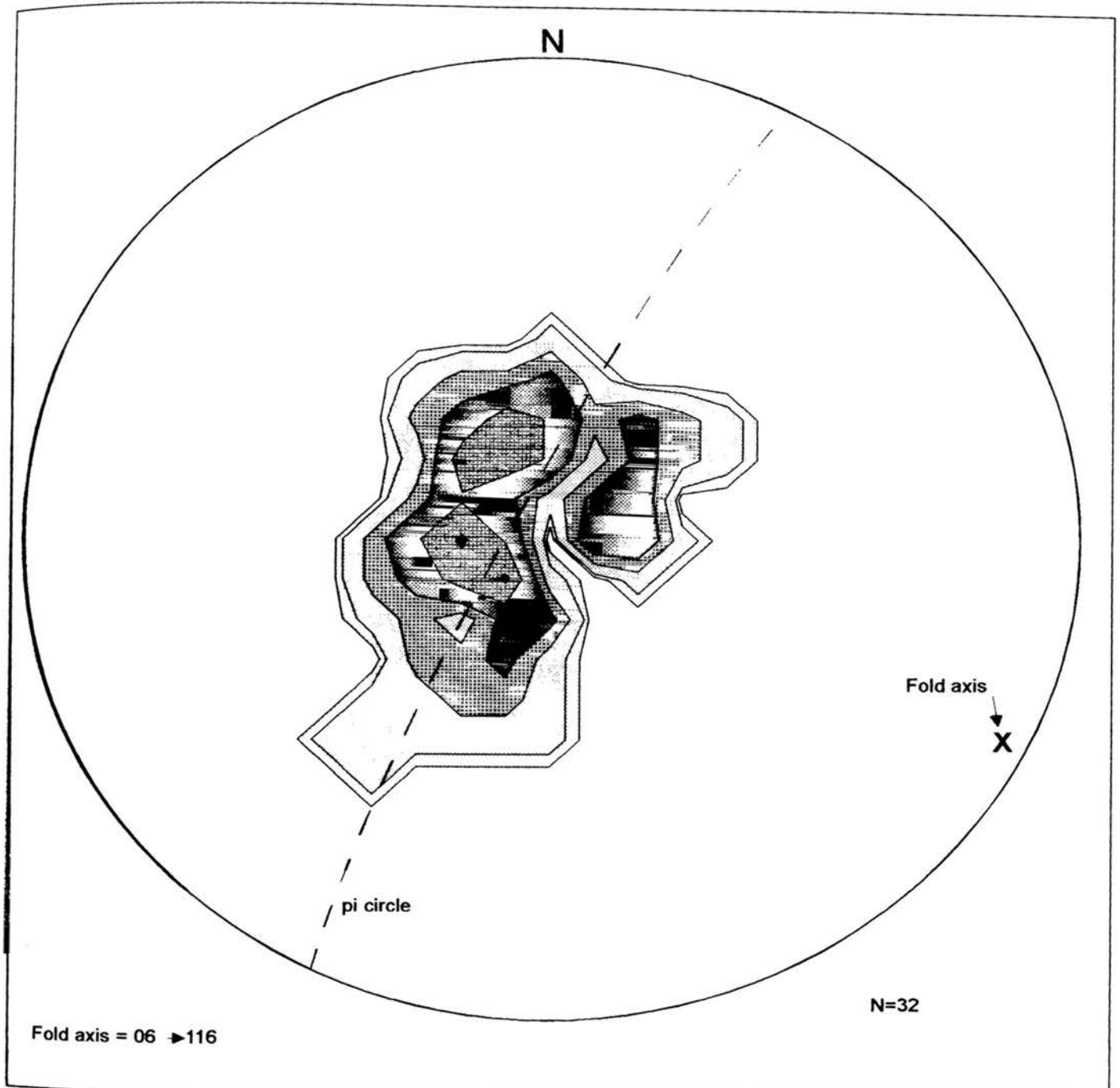
Figure 3.13: Stereographic projection of the density distribution of poles to bedding in the area east of the Rustenburg Fault (location 8) in Rustenburg Nature Reserve. Fold axis plunges 06 ->116.
