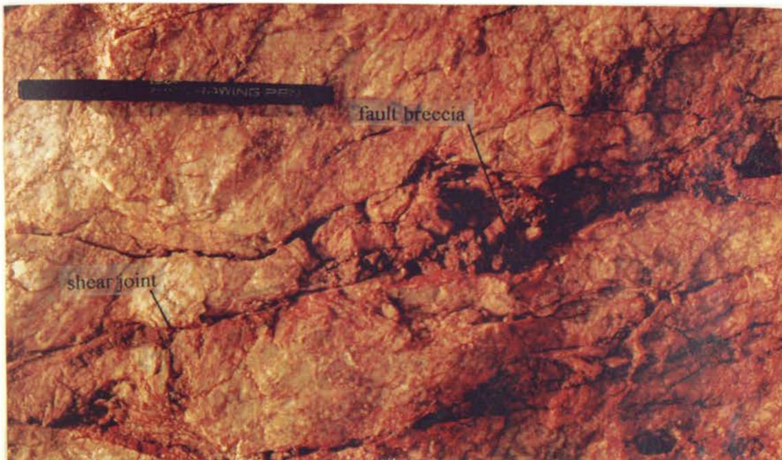
Figure 3.35: Fault breccia produced by shear jointing in Fault quartzite at location 20. Pen is 13 cm long.
