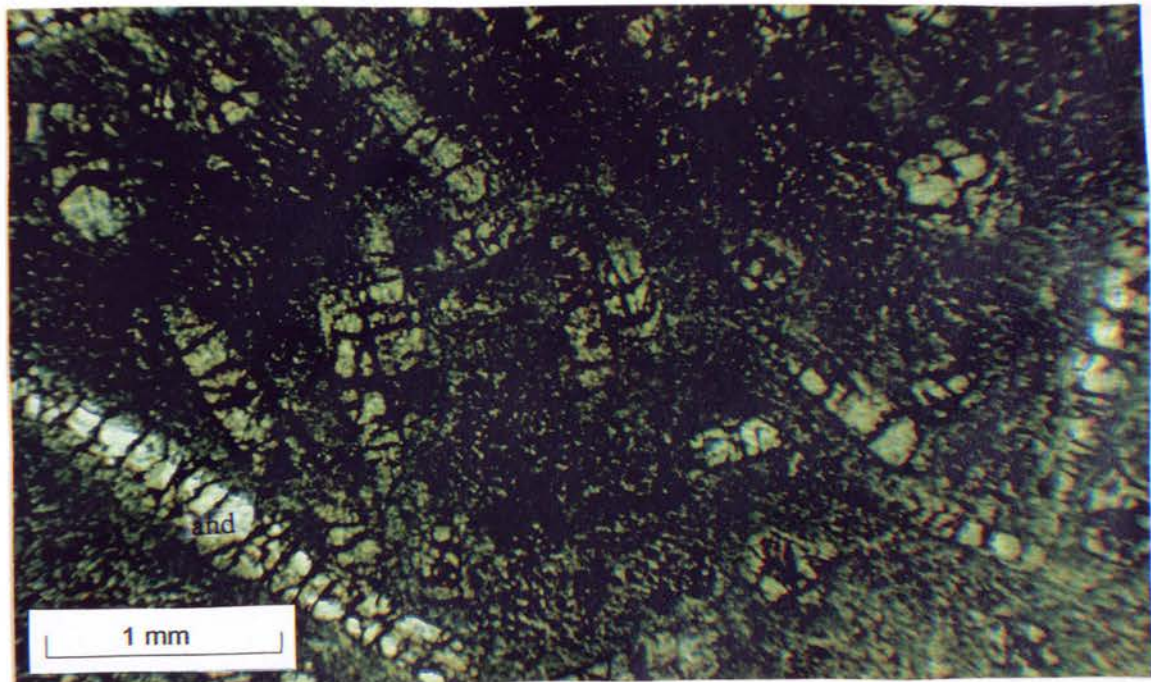
Figure 2.18: Photomicrograph of hornfels in the Magaliesberg Formation, showing acicular andalusite crystals in a fine-grained chloritic groundmass (plane poles).
