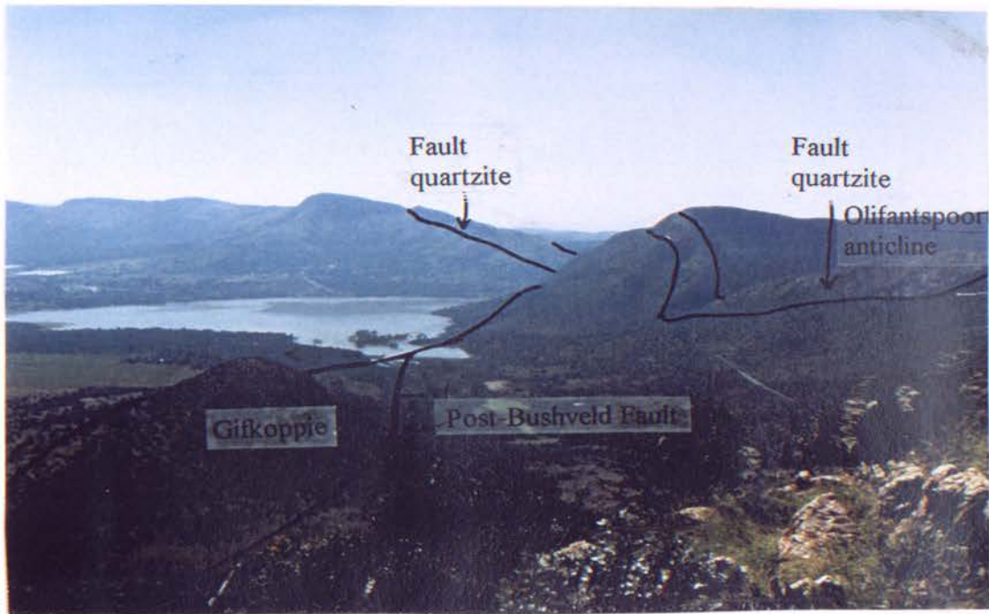
Figure 4.6: Inferred fault geometry at location 19, looking northwards. The unbroken line of Fault quartzite passes from left to right across the top of the photograph. Gifkoppie may have been faulted from beneath Olifantnek dam and dragged southwards to its present location, without disturbing the trend of the Fault quartzite above.
