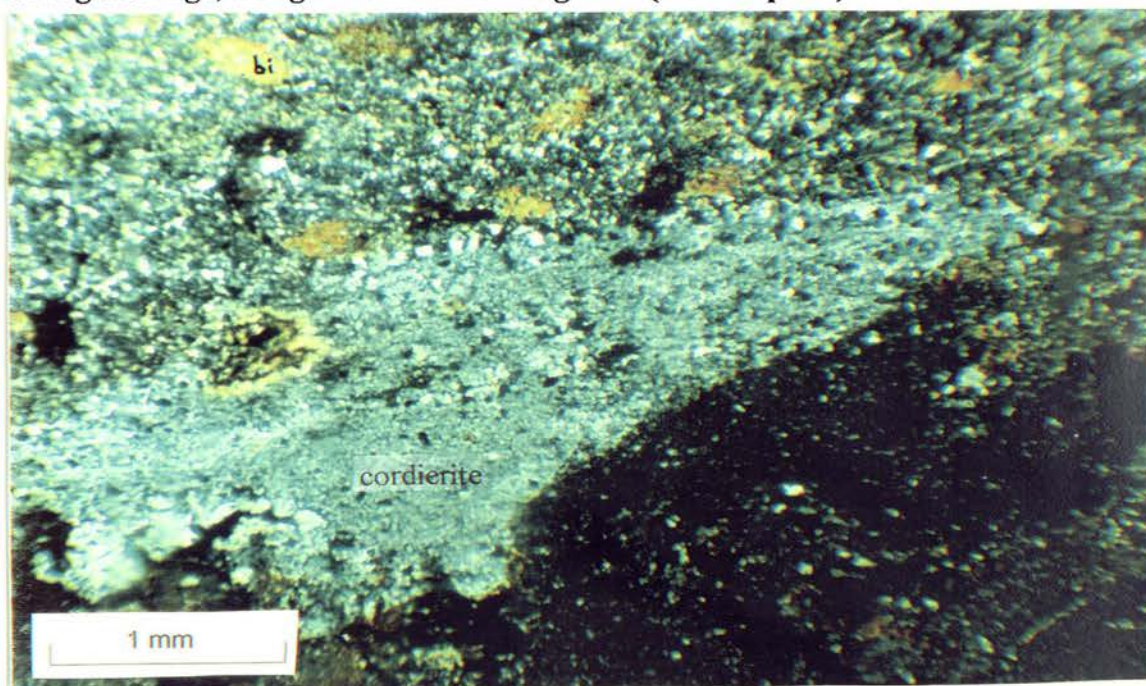
Figure 2.7: Photomicrograph of a cordierite-biotite hornfels in the Silverton Formation at 25° 56.25' S: 27° 20.10' E. Cordierite has grown in preference to andalusite due to lack of Fe (less secondary haematite compared to Figure 2.6). The large, partly pinitised cordierite poikiloblast shows diagnostic twinning (crossed poles). The poikiloblasts of either cordierite or andalusite give the characteristic 'spots' in hornfels.
