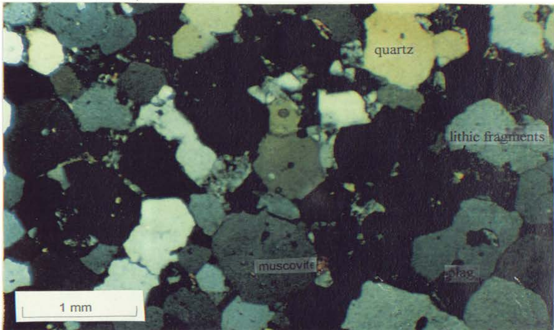
Figure 2.13: Photomicrograph of Magaliesberg sandstone from 25° 47.50' S; 27° 16.84' E, showing quartz, plagioclase, lithic fragments and secondary sillimanite and muscovite (crossed poles).
