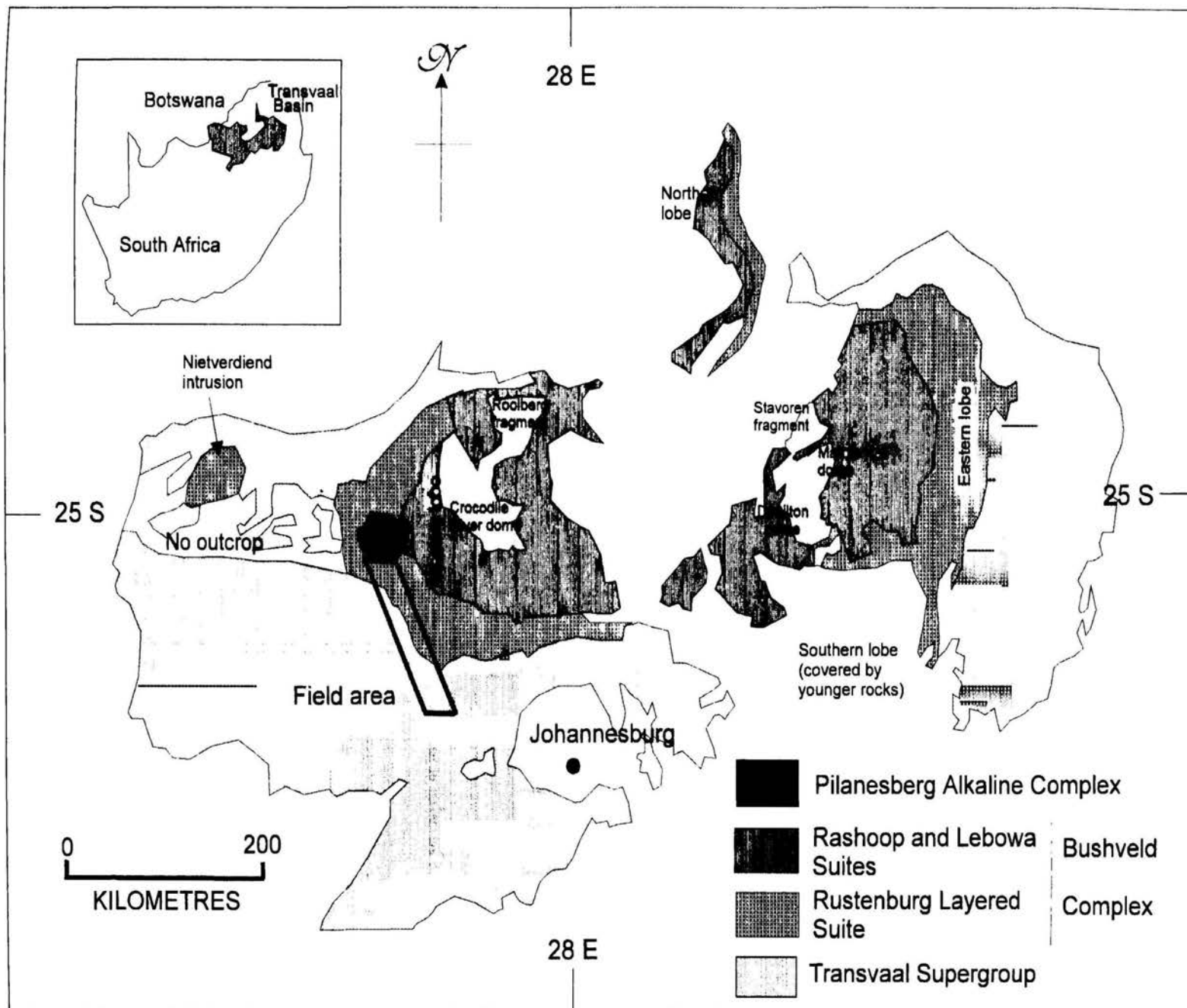
Figure 1.4: Map of the Bushveld Complex (After Eriksson et al., 1995).
