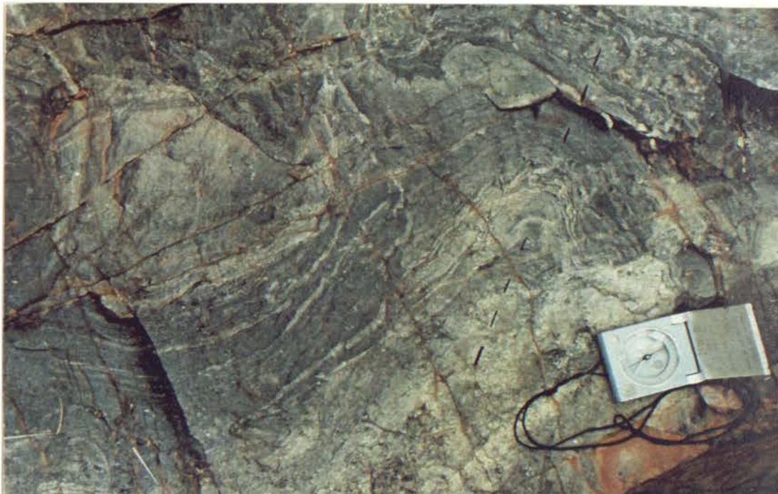
Figure 3.36: Folding of psammitic and pelitic laminations in Silverton shale at location 23. The indicated fold axial trace has a trend of 120^{\circ} (note north arrow on compass). Parasitic folds of the same orientation are also visible on the fold limbs. It was not possible to measure the plunge or fold axial plane on this outcrop. Note that the trend of this fold axial trace is parallel to the F_1 folds identified in section 3.1.2.3. Compass is 8 cm wide.
