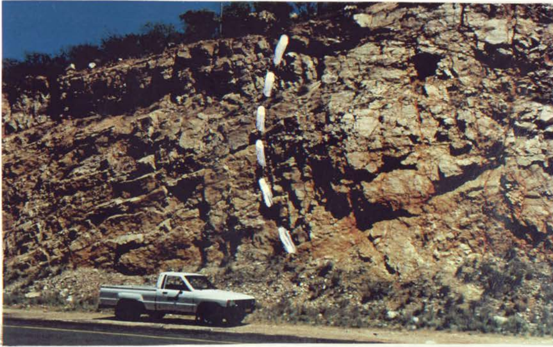
Figure 3.33: Rustenburg Fault zone at location 20. Photograph is taken looking southwards. A 20m diameter block of Magaliesberg quartzite (note bedding planes on the left) is enclosed within a matrix of Fault quartzite to the right. The edge of the Magaliesberg block is marked by a dashed white line. Note the intense jointing at the interface between these two lithologies (also Figure 3.34).
