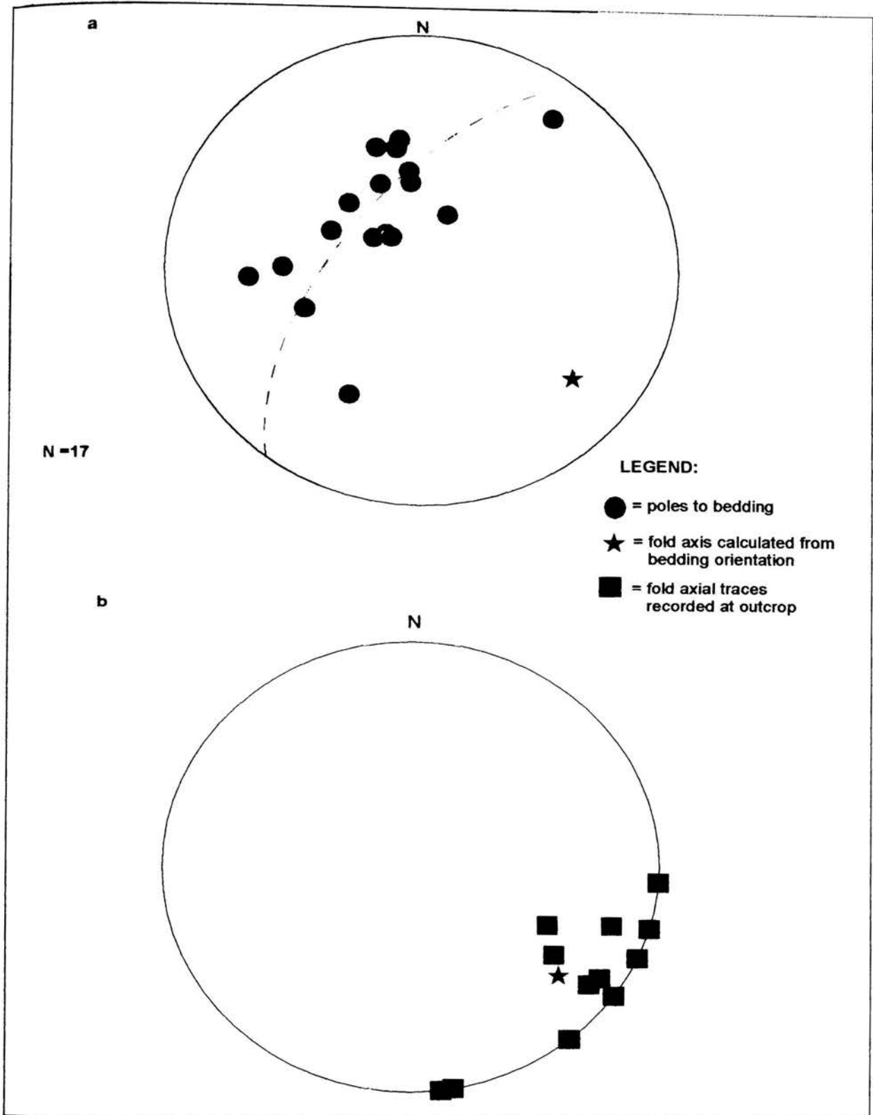
Figure 3.54: Stereographic projections of poles to bedding and fold axes at location 39. a. shows the orientation of poles to bedding, the best fit pi circle, and the fold axis. b. shows the orientation of fold axial traces recorded throughout the outcrop, which are of similar orientation to the fold axis predicted in a.
