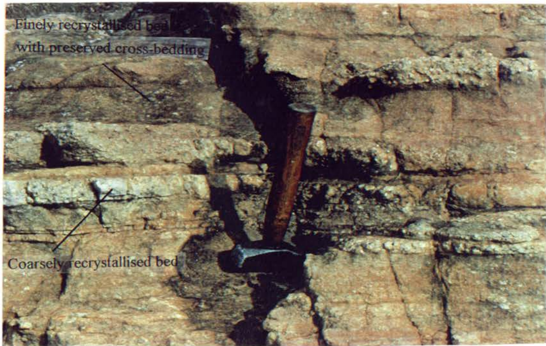
Figure 2.12: Differential degrees of recrystallisation in beds of Magaliesberg quartzite (25° 42.97' S; 27° 12.12' E).
