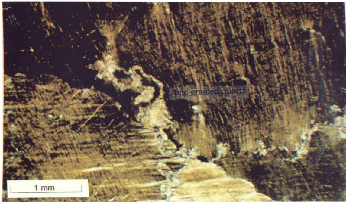
Figure 3.25: Photomicrograph showing deformation lamellae in Fault quartzite from location 12. Note that all crystals possess the same type of deformation within each photomicrograph (also figure 3.24). Extremely fine-grained quartz can be seen along the large crystal boundaries.
