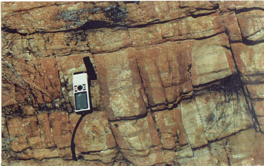
Figure 3.40: Shearing and fluid transport along joints at location 28, showing 2 cm of normal displacement, with downthrow to the S.W.. The joints have also acted as fluid conduits, with each joint showing a 3cm wide band of strong haematite staining on each side. G.P.S. receiver is 15 cm tall.
