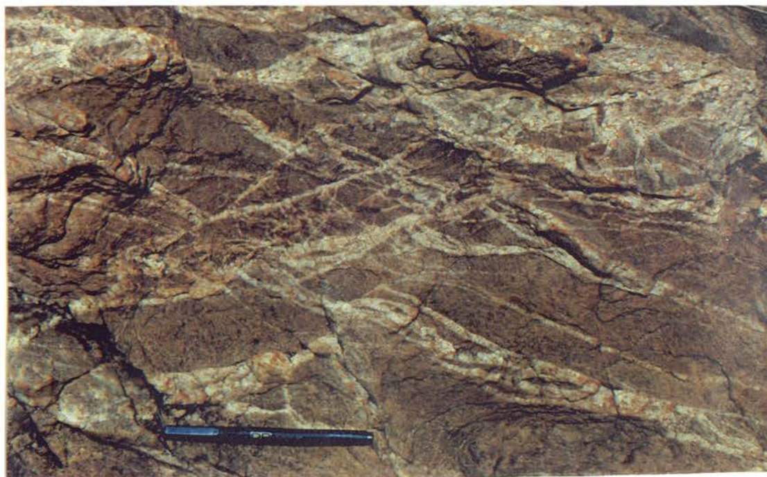
Figure 3.28: Veins cross cutting Fault quartzite at location 12. The haematite staining is untypical of Fault quartzite. Note that at least two sets of veins are present (from top right to bottom left, and top left to bottom right). Pen is 13 cm long.
