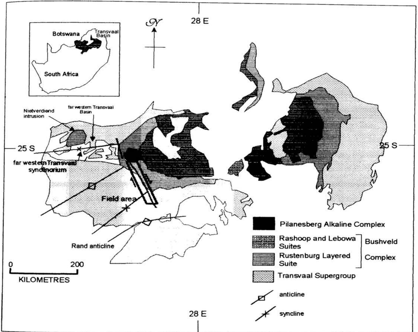
Figure 4.10: Geological map of the Transvaal Basin, showing compression of the far-western Transvaal Basin, as indicated by E.N.E.-W.S.W. to N.E.-S.W. trending folds. (after Dietvorst, 1991; Eriksson et al., 1995.)
