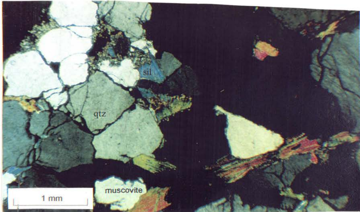
Figure 2.14: Photomicrograph of slightly recrystallised Magaliesberg quartzite from 25° 39.80' S: 27° 09.60' E, with high percentage of sillimanite, muscovite and primary matrix. Note the original rounded grain boundaries at the crystal/matrix interfaces in the top left hand corner (crossed poles).
