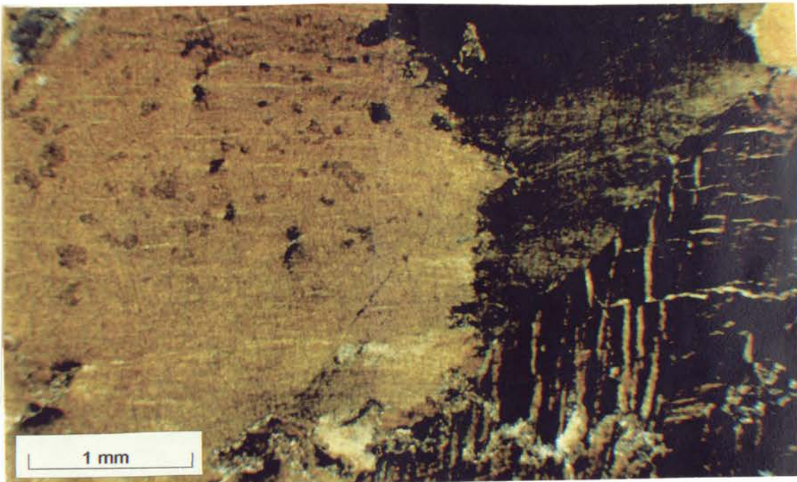
Figure 3.22: Photomicrograph of Fault quartzite from location 12 showing undulose extinction and deformation lamellae (at bottom right) and very large crystal size (about 5mm).
