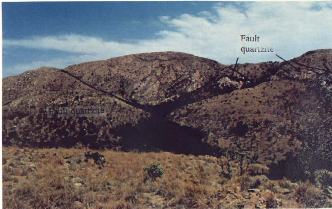
Figure 3.39: Disruption of the Rustenburg Fault zone at location 26 by later faults. The western edge of the steeply N.E.-dipping Rustenburg Fault zone (i.e. the contact of the Fault quartzite with The Magaliesberg Formation quartzite) is shown by the solid line, and the cross-cutting N.E.-striking faults are shown by dashed lines.
