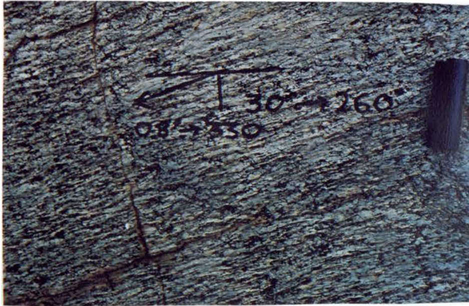
Figure 3.49: Lineation at location 37, caused by intersection of bedding and foliation in “mylonite”. S_0 = 170^\circ 30' W ( 30^\circ \rightarrow 260^\circ ) and S_1 ( 160^\circ 45' W ) intersect to form L_1 ( 08^\circ \rightarrow 330^\circ ). Pen tip is 3 cm long.
