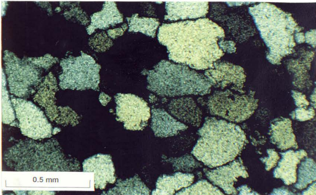
Figure 2.5: Photomicrograph of Daspoort sandstone at 25° 58.41' S: 27° 21.26' E, showing good sorting of medium-sized quartz grains, a lack of cement, and pressure solution at grain boundaries creating angular grain shapes (crossed poles).
