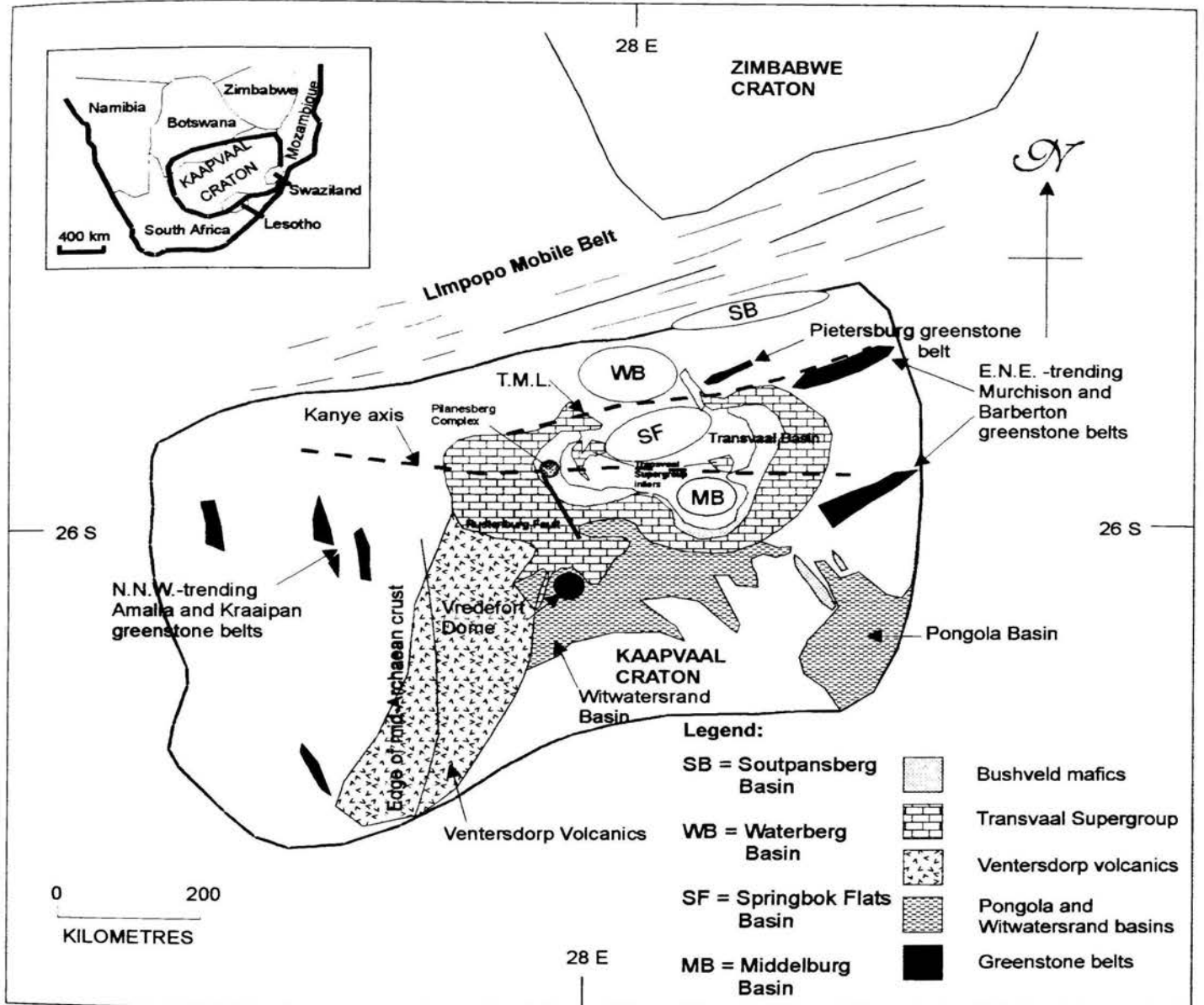
Figure 1.5: Major structural elements of the Kaapvaal craton (after Burke et al., 1985; Stanistreet & McCarthy, 1991; de Wit et al., 1992; Eriksson et al., 1995).
