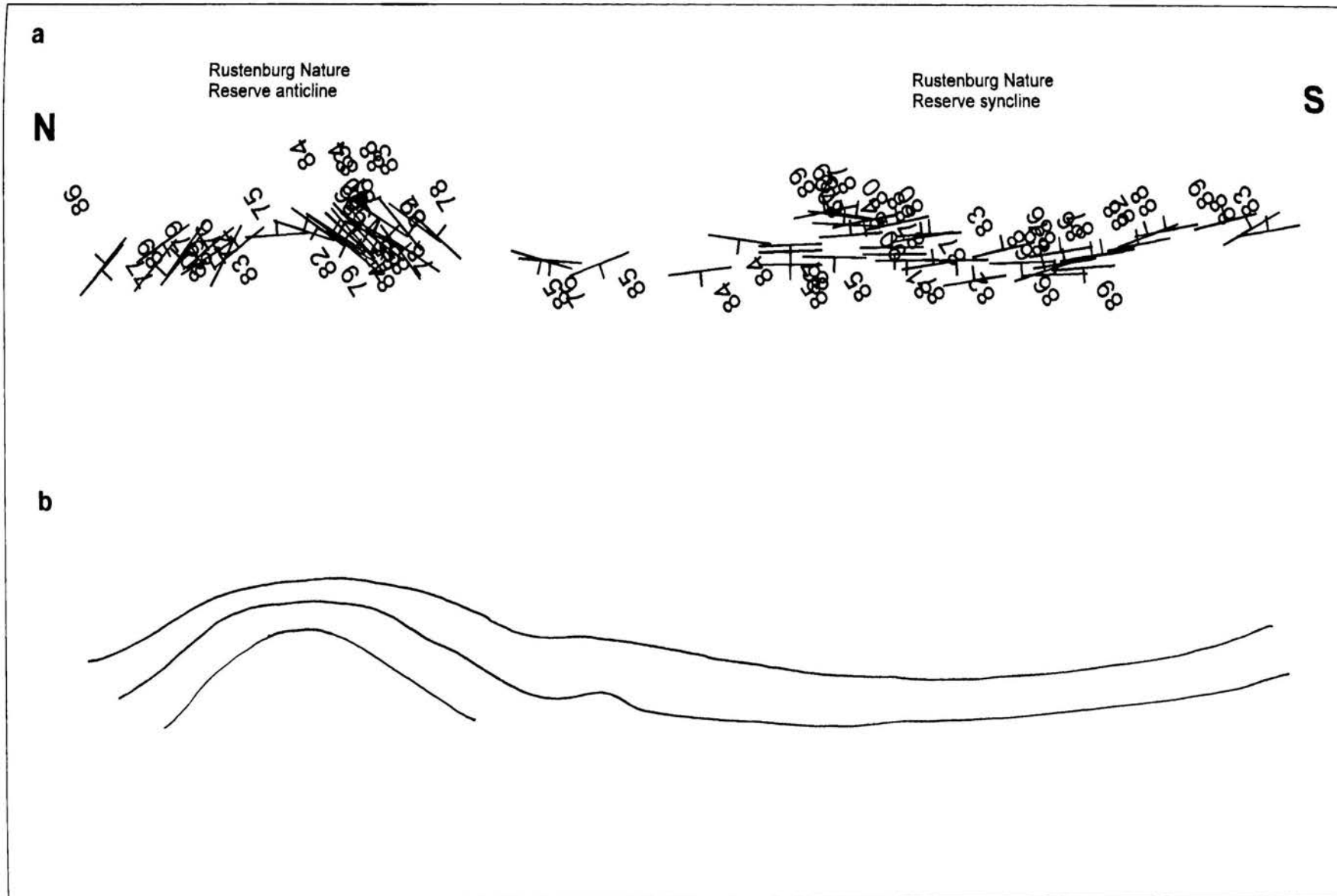
Figure 3.18: a.: Down-plunge projection of the Rustenburg Nature Reserve folds. The variable nature of the dips around vertical results from the curved fold axial surfaces.
