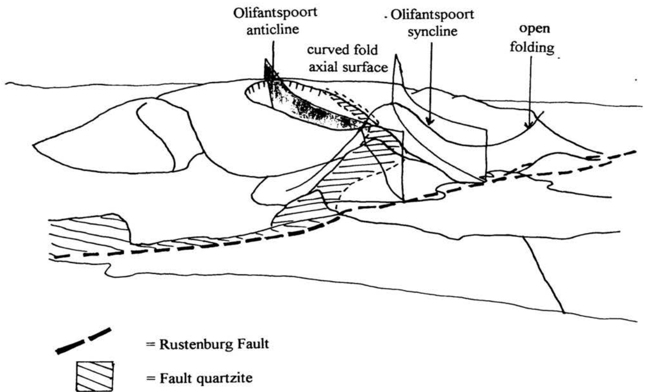
Figure 3.4: Folding at Olifantspoort. Photograph (a) is taken looking S.E., with Olifantsnek dam in the foreground. The anticline is to the north, syncline to the south. The Rustenburg Fault crosses the area between the dam and Olifantspoort (b). b. shows the inferred shape of the folding, with upright, curved fold axial surfaces and open folding.
