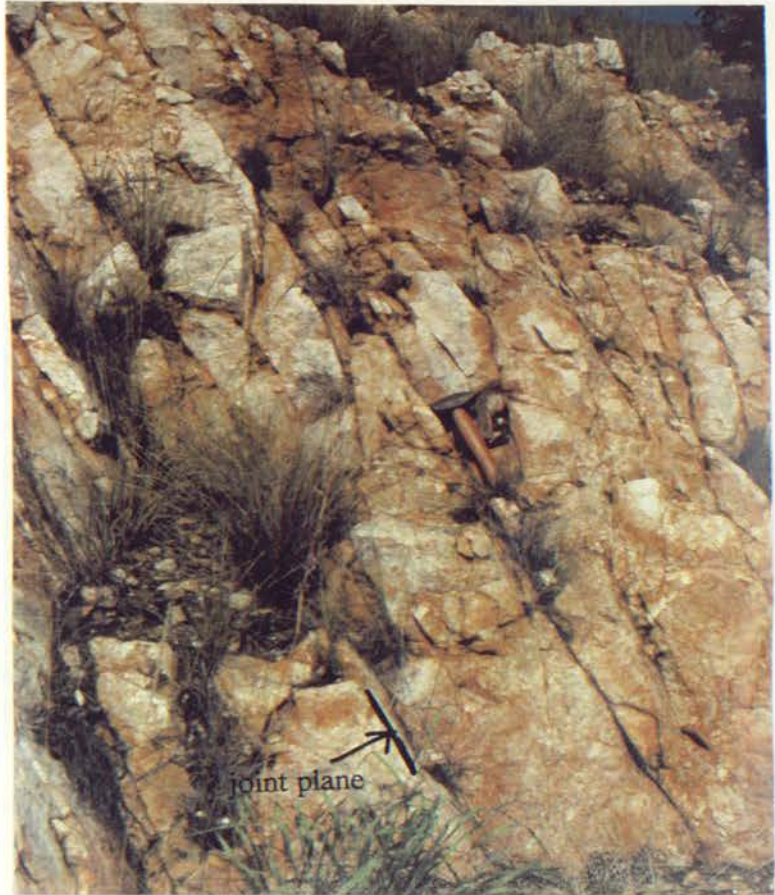
Figure 3.19: Fault quartzite at location 10, showing apparently massive character, and a joint plane of 132^{\circ} 70^{\circ} S.W..
