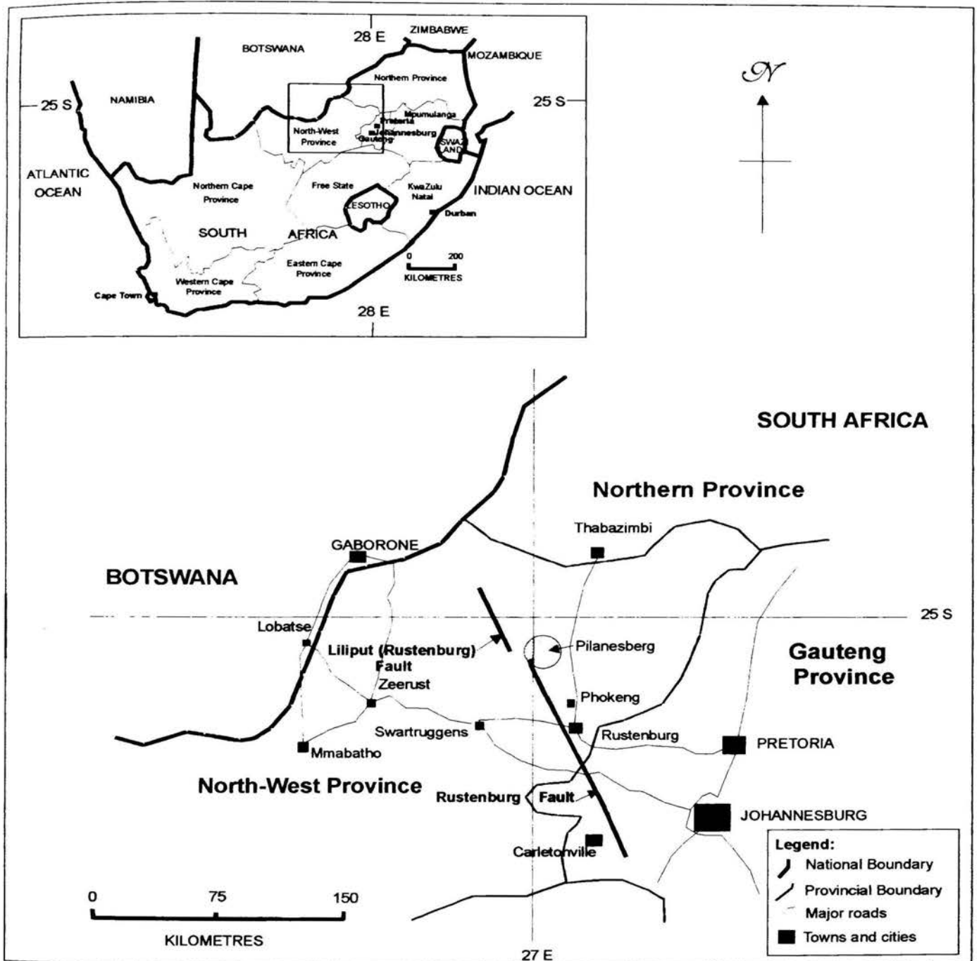
Figure 1.1: Geographical location of the Rustenburg Fault.
