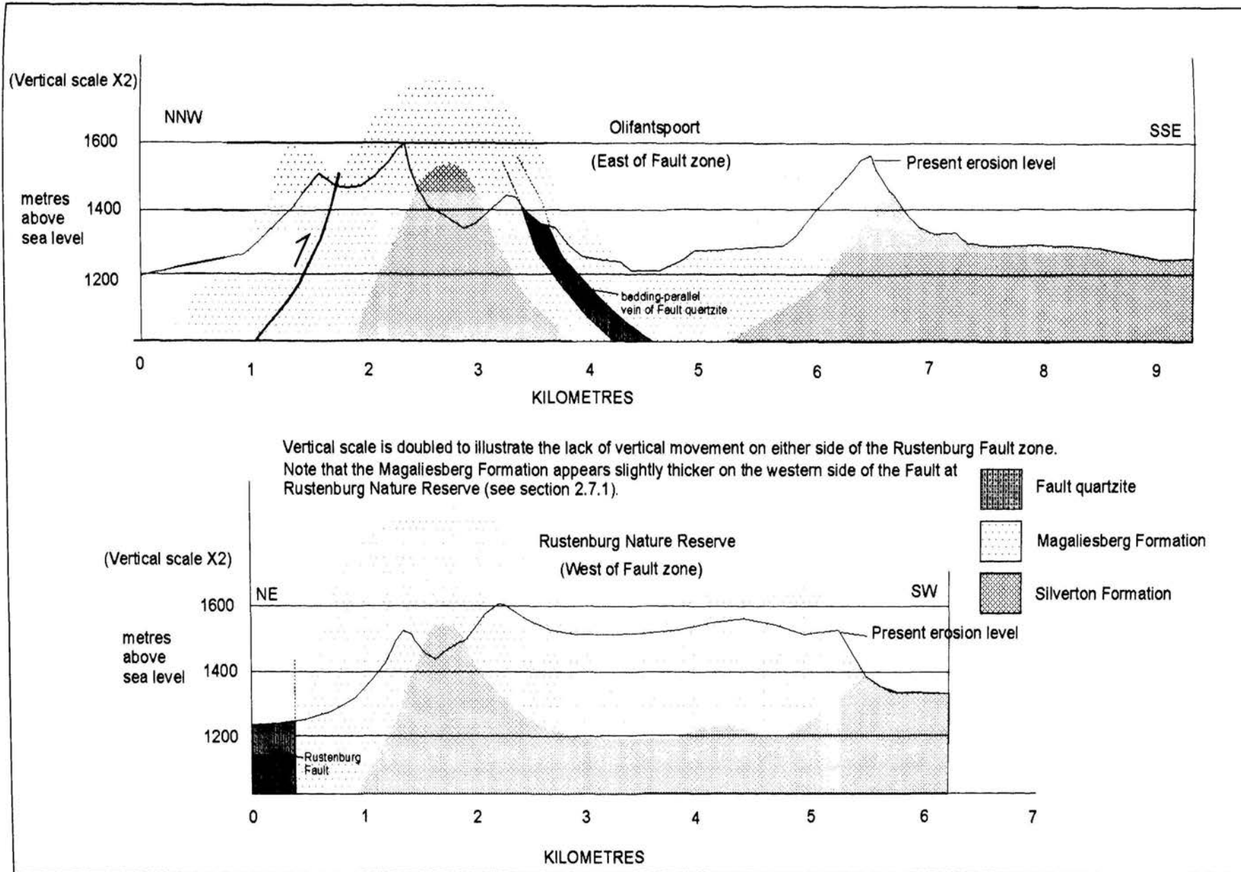
Figure 4.2: Cross sections through the Olifantspoort and Rustenburg Nature Reserve folds, showing little vertical displacement, as shown by the corresponding altitude of the projected crests of the anticline in both areas.
