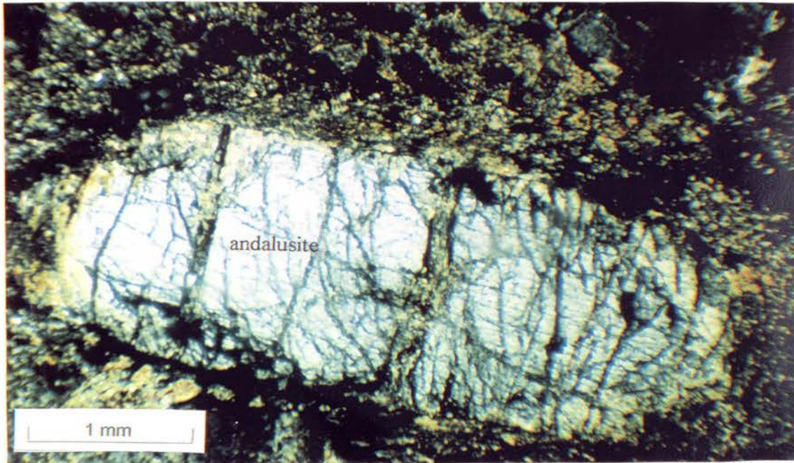
Figure 2.6: Photomicrograph of an andalusite hornfels in the Silverton Formation at 25° 56.00' S: 27° 20.50' E. Groundmass is quartz, haematite and secondary biotite. The large andalusite crystal shows the diagnostic cruciform pattern of chiastolite. The andalusite has a strong cleavage, along which biotite has grown (crossed poles).
