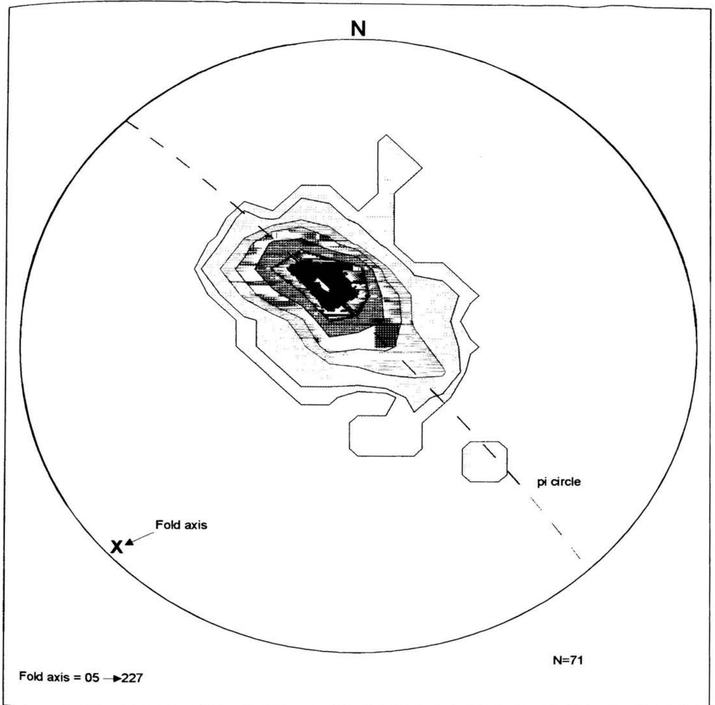
Figure 3.15: Stereographic projection of the density distribution of poles to bedding in the Magaliesberg quartzite in the area from Phokeng to Pilanesberg, west of the Rustenburg Fault. Fold axis plunges 05 → 227.
