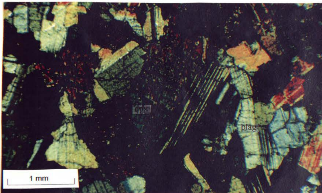
Figure 2.21: Photomicrograph of a lower, contact norite from the Bushveld Complex, showing plagioclase and orthopyroxene. The hand specimen from which this was taken shows layering of orthopyroxenes (crossed poles).
