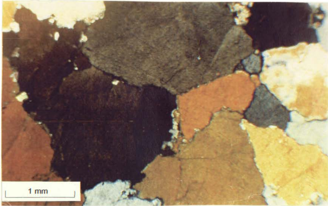
Figure 3.23: Photomicrograph of Magaliesberg quartzite at location 13, showing an average crystal size of 2mm, slight undulose extinction and pressure solution at grain boundaries.
