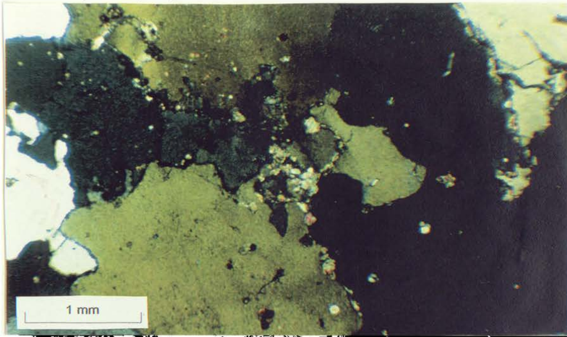
Figure 2.15: Photomicrograph of coarse recrystallised Magaliesberg quartzite from 25° 47.32' S: 27° 16.66' E, showing frequent small inclusions and plentiful small secondary metamorphic mineral crystals impeding quartz crystal growth (crossed poles).
