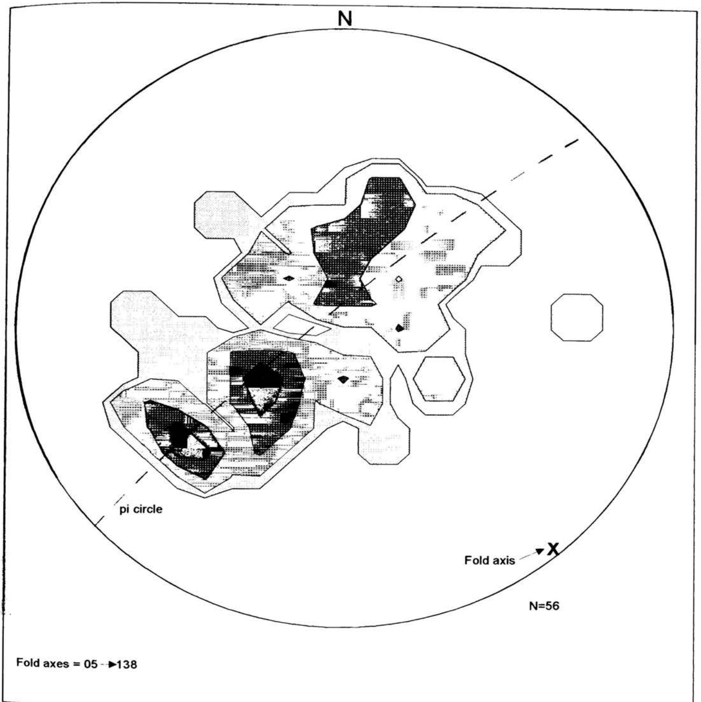
Figure 3.16: Stereographic projection of the density distribution of poles to bedding in the Magaliesberg quartzite in the area from Phokeng to Pilanesberg, east of the Rustenburg Fault, showing that variable bedding orientation may have resulted from interference folding around two fold axes.
