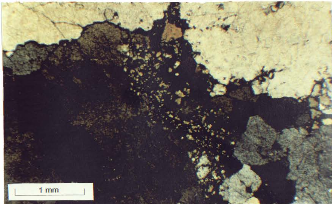
Figure 3.26: Photomicrograph from location 15, showing fine-grained quartz crystals within Fault quartzite which have failed to be recrystallised.
