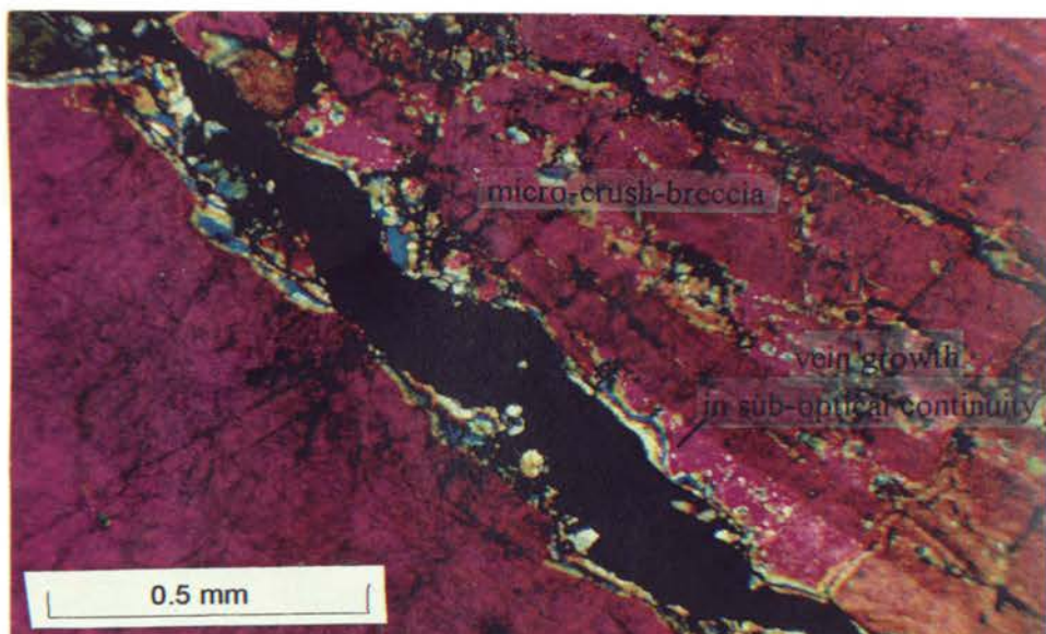
Figure 3.30: Photomicrograph showing annealing halted in progress at location 17. Vein growth in sub-optical continuity is occurring across a micro-fault filled with a micro-crush-breccia (as defined by Sibson, 1977) (thick section).
