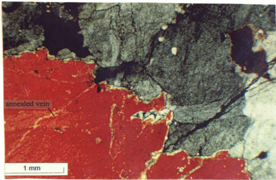
Figure 3.29: Photomicrograph from location 12, showing annealed veins grown in sub-optical continuity across quartz in crystals in Fault quartzite (thick section).
