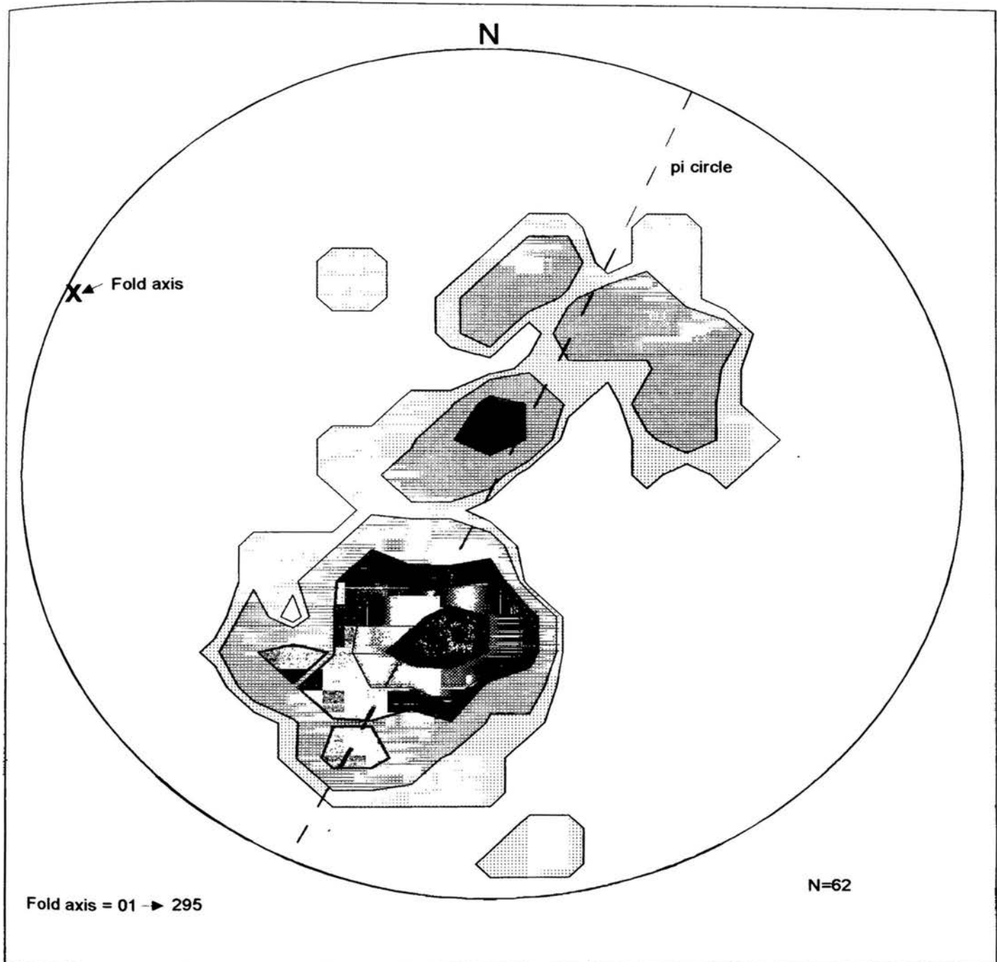
Figure 3.9: Stereographic projection of the density distribution of poles to bedding in the Olifantspoort anticline. Fold axis plunges 01 → 295.
