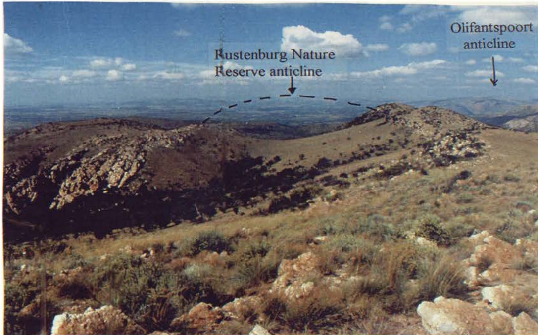
Figure 3.6: The Rustenburg Nature Reserve anticline, showing open folding with an approximately upright fold axial surface. The photograph is taken looking eastwards. Note Olifantspoort anticline just visible in the distance to the S.E..
