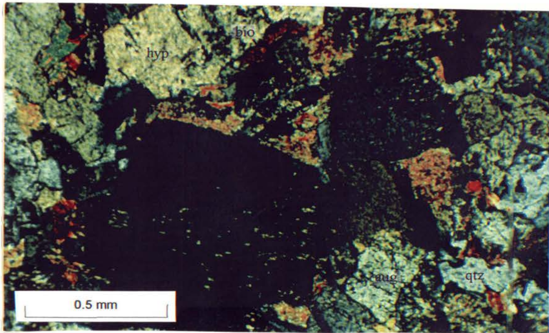
Figure 2.20: Photomicrograph of a norite sill at 25° 38.50' S: 27° 08.50' E, showing hypersphene laths, surrounded by interstitial quartz, augite and biotite (crossed poles).
