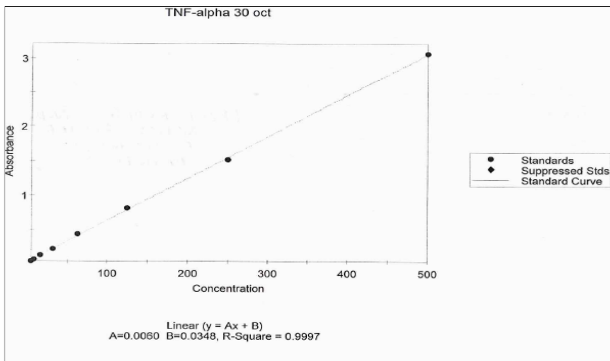
Figure 5.8: Standard curve of (a) IL-8 and (b) TNF- \alpha developed by using ELISA method
