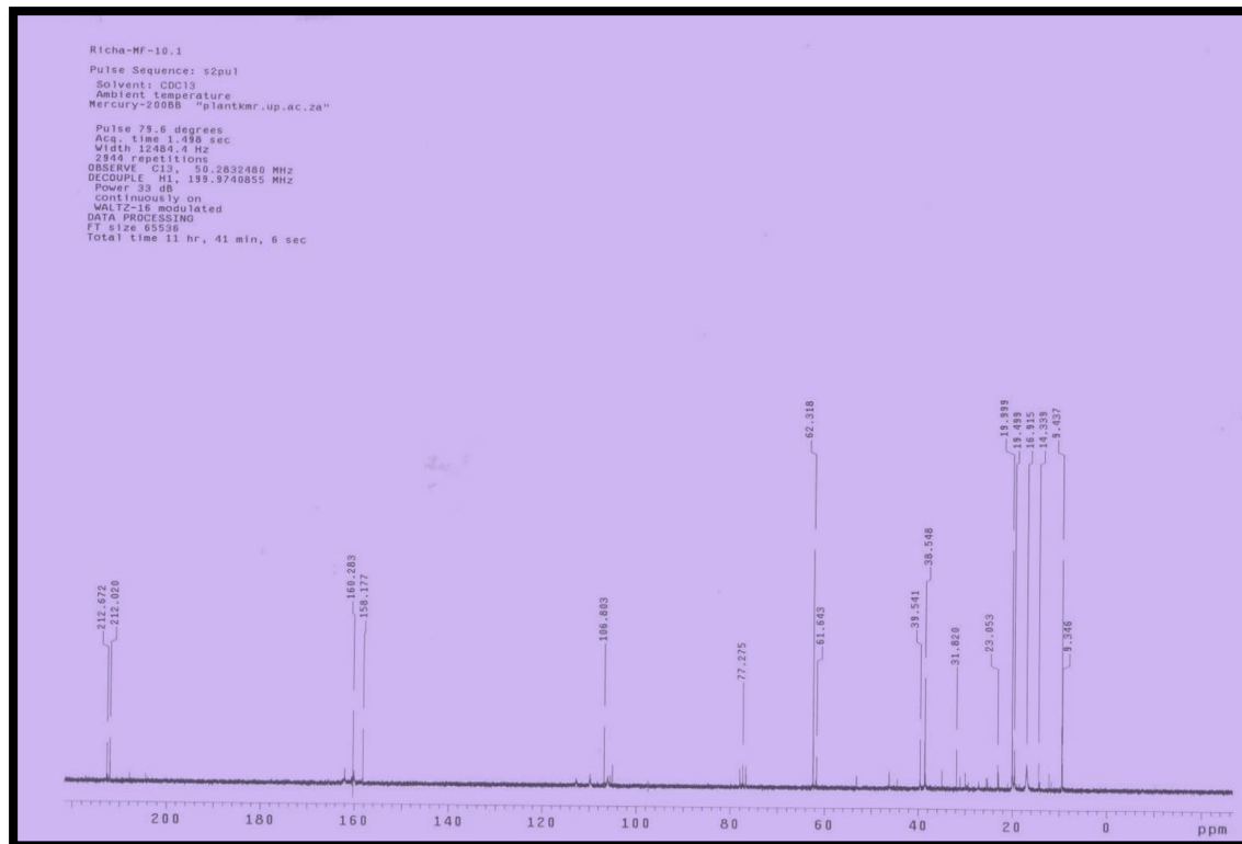
Figure 9.4: (a) ^1\text{H} -NMR and (b) ^{13}\text{C} -NMR of alpha kosin
