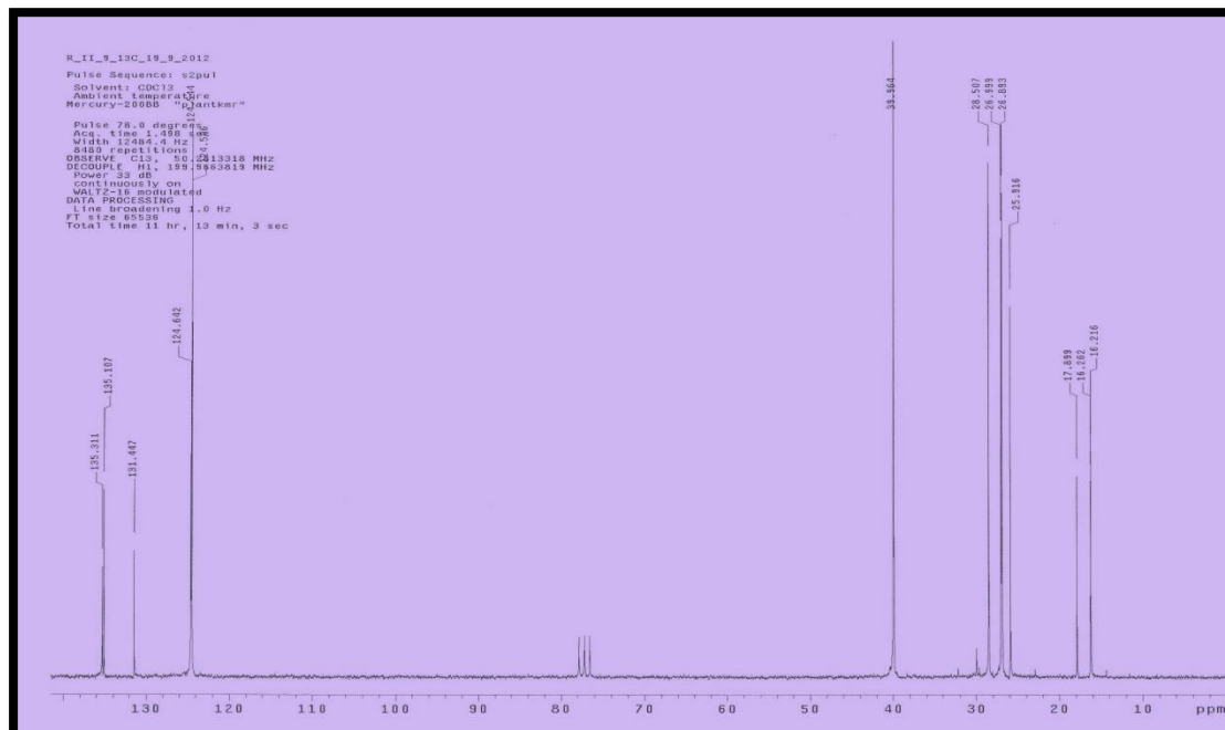
Figure 9.1: (a) ^1\text{H} -NMR and (b) ^{13}\text{C} -NMR of squalene
