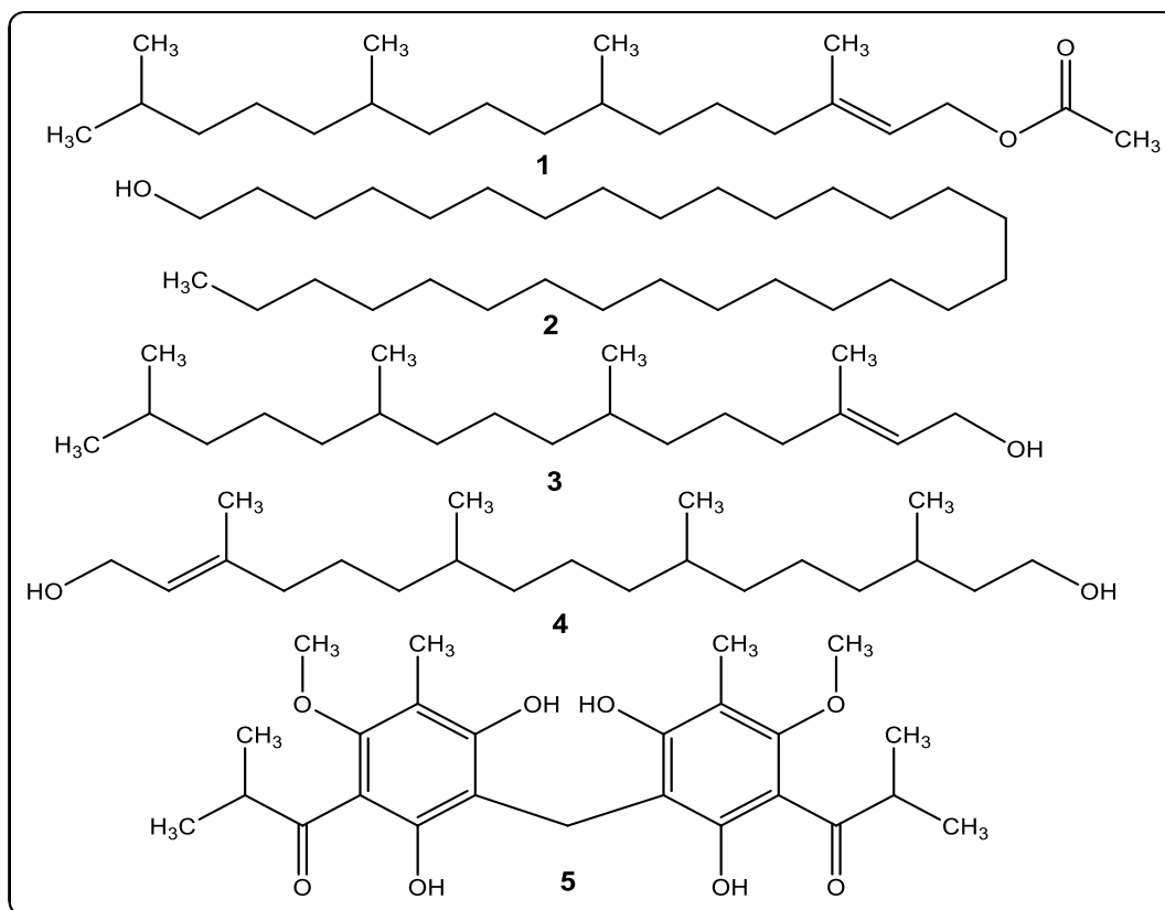
Figure 6.2: Structures of isolated compounds from ethanol extract Leucosidea sericea : phytol acetate ( 1 ), triacontanol ( 2 ), phytol ( 3 ), ( E )-3,7,11,15-tetramethylheptadec-2-ene-1,17-diol ( 4 ) and alpha kosin ( 5 )
