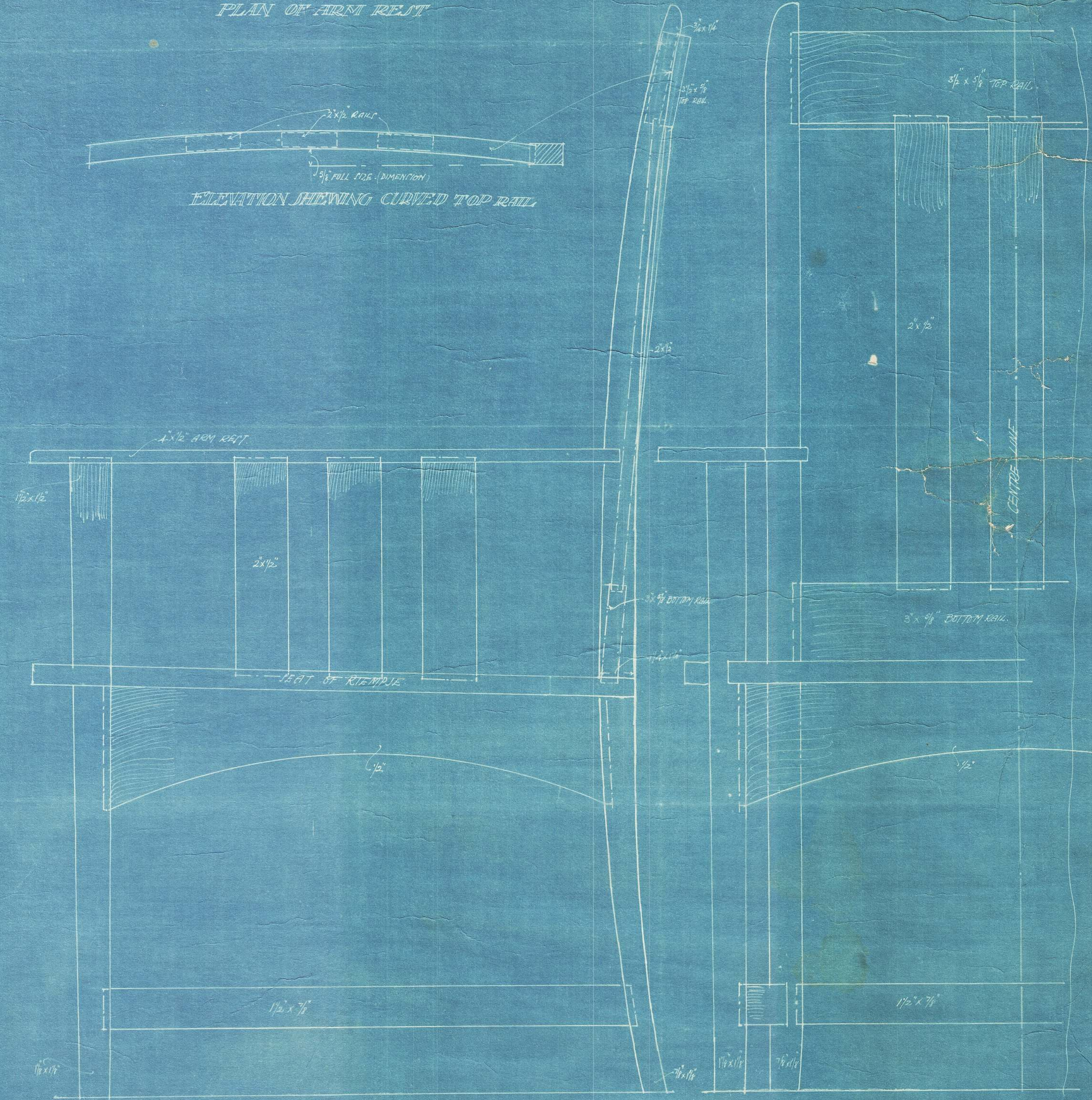
SIDE AND HALF ELEVATION OF ARM CHAIR
