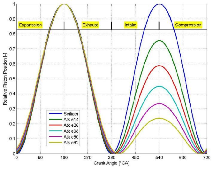
Figure 2 Relative Displacements of the used Asymmetrical Crank Mechanism The Atkinson (Atk) cycles are implemented by means of variation of the eccentric radiuses exx of the used crank mechanism. The Seiliger cycle is realized with zero eccentric radius.
