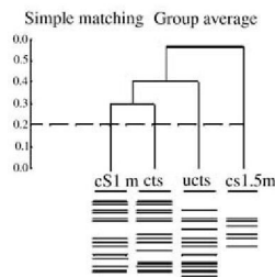
Fig. 6. (a) Cluster analysis of microbial communities at different soil layers and (b) DGGE fingerprints. Key: ucts–uncontaminated topsoil; cts–contaminated topsoil; cs1m–contaminated soil layer at 1m; cs1.5m–contaminated soil layer at 1.5m; m–marker. Lines beneath codes in (a) represent the bands detected.
