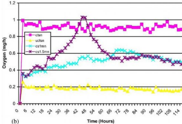
Fig. 3. Oxygen consumption by microorganisms in different layers of diesel-contaminated soil: (a) soil without added nutrients; (b) soil with added nutrients. Key: cts–contaminated topsoil, no nutrients added; ctsn–contaminated topsoil, nutrients added; ucts–uncontaminated topsoil, no
