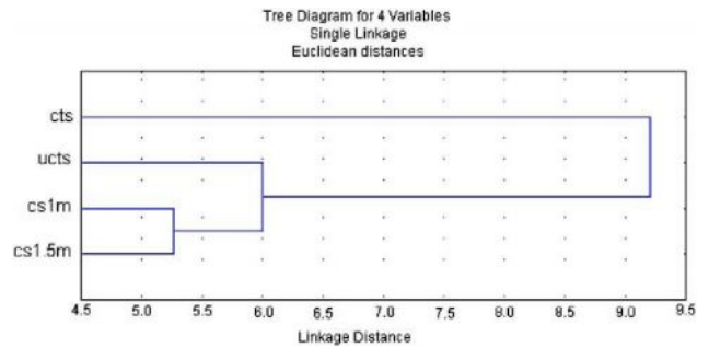
Fig. 5. Cluster analysis of different soil layers.
