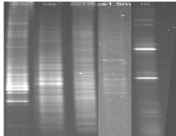
Fig. 6. (a) Cluster analysis of microbial communities at different soil layers and (b) DGGE fingerprints. Key: ucts–uncontaminated topsoil; cts–contaminated topsoil; cs1m–contaminated soil layer at 1m; cs1.5m–contaminated soil layer at 1.5m; m–marker. Lines beneath codes in (a) represent the bands detected.
