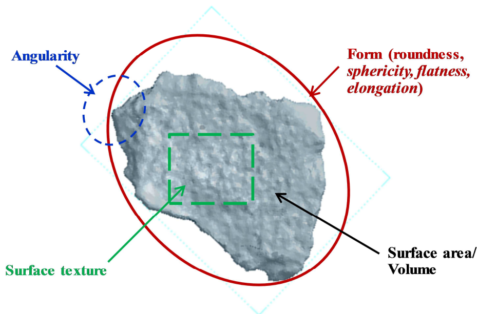
Figure 1: Fundamental aggregate shape properties (Anochie-Boateng et al., 2011).
