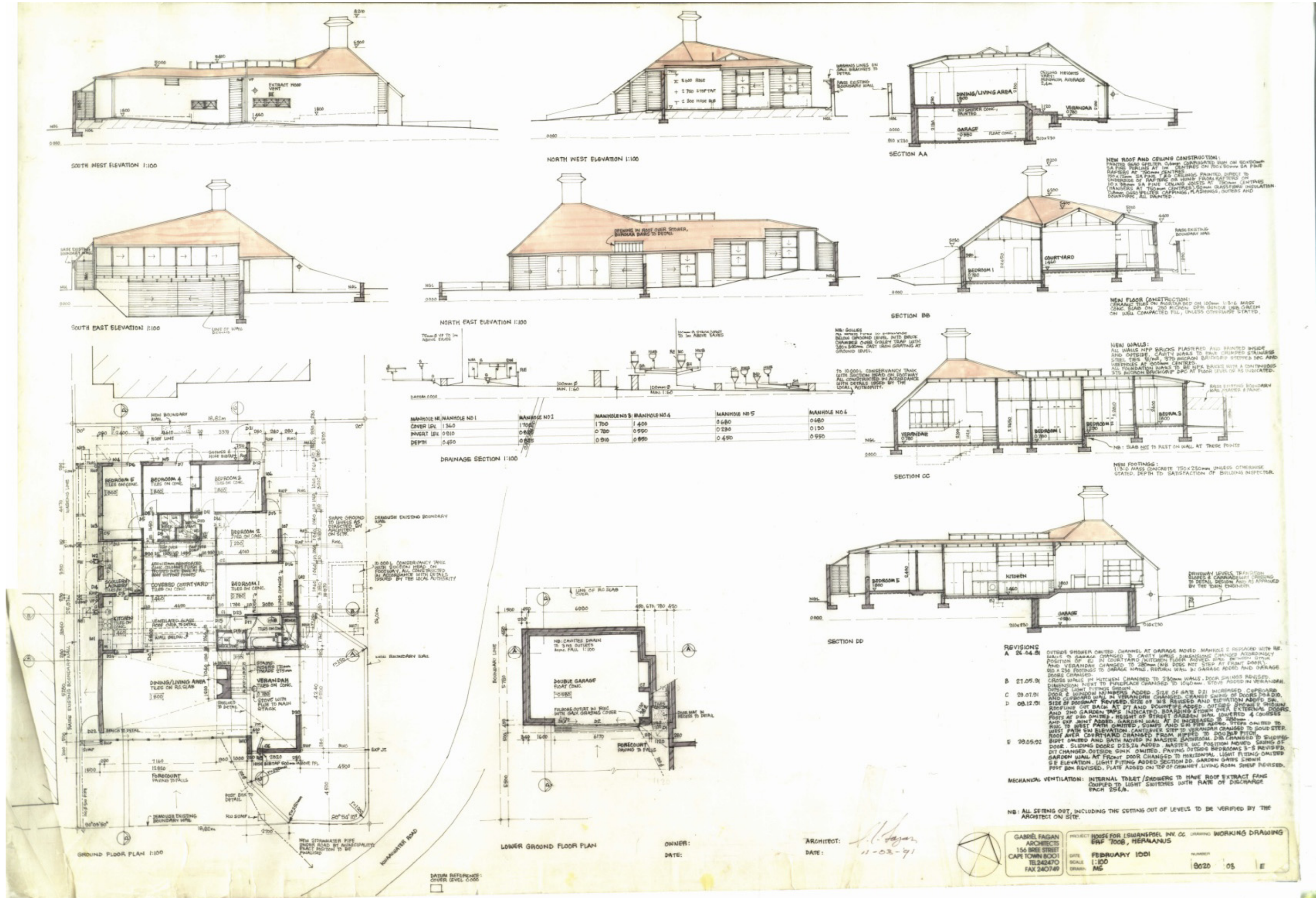
11. Working drawing
