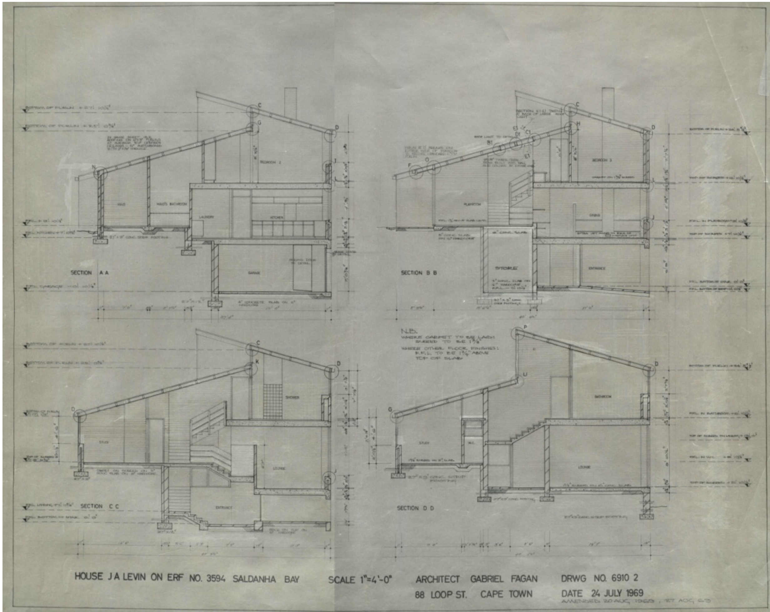
12. Working drawings
