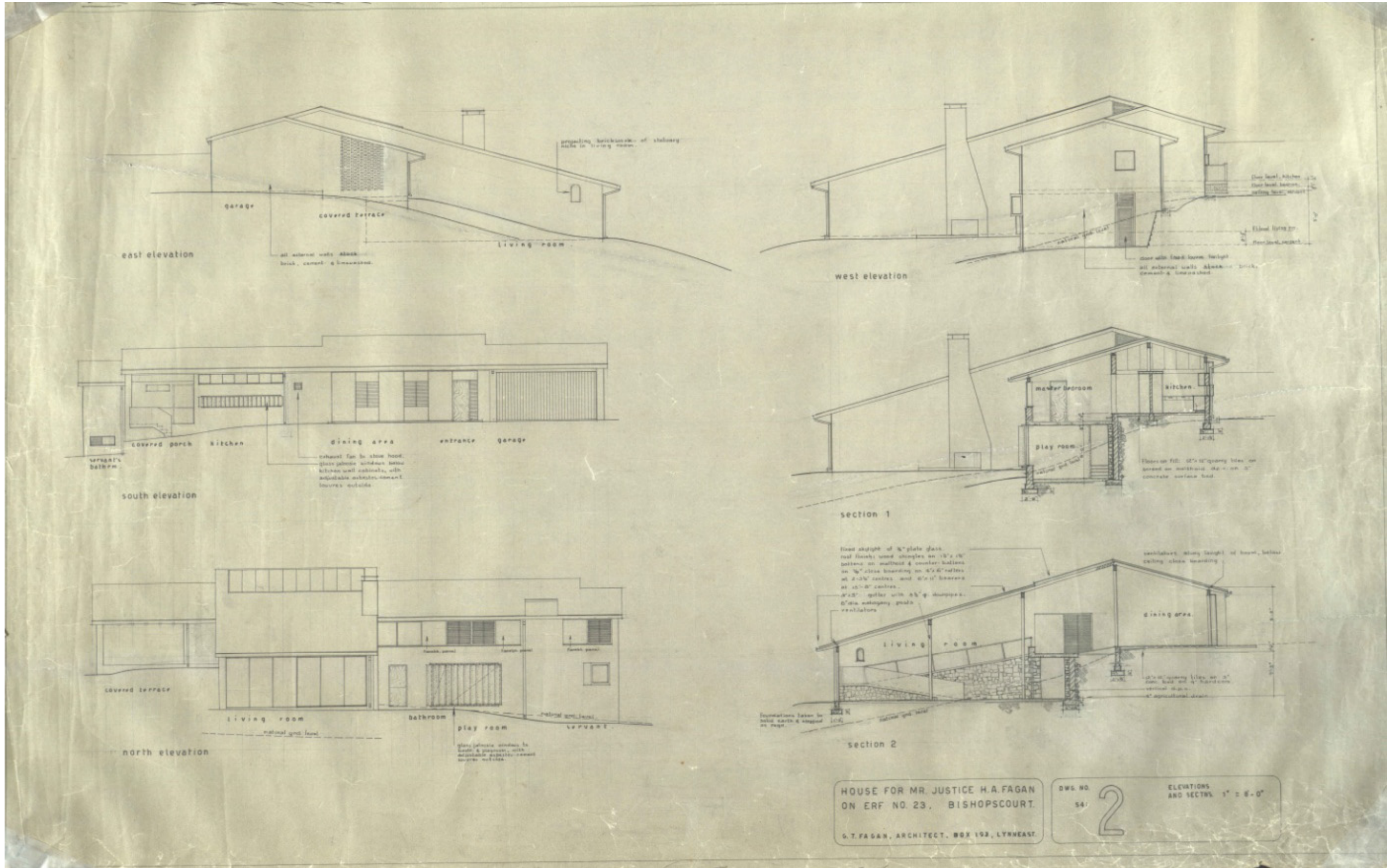
12. Working drawings
