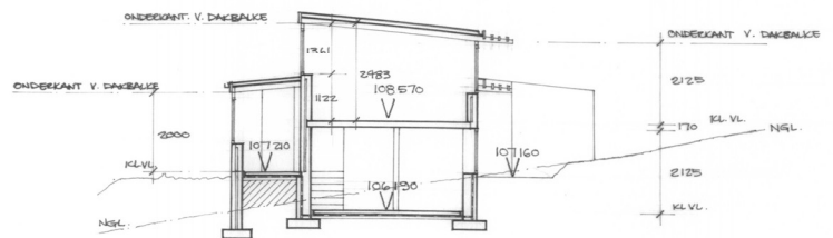
SNIT B
