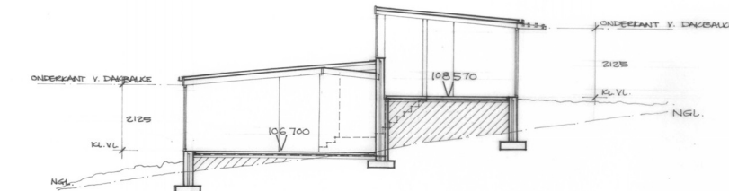
SNIT C
