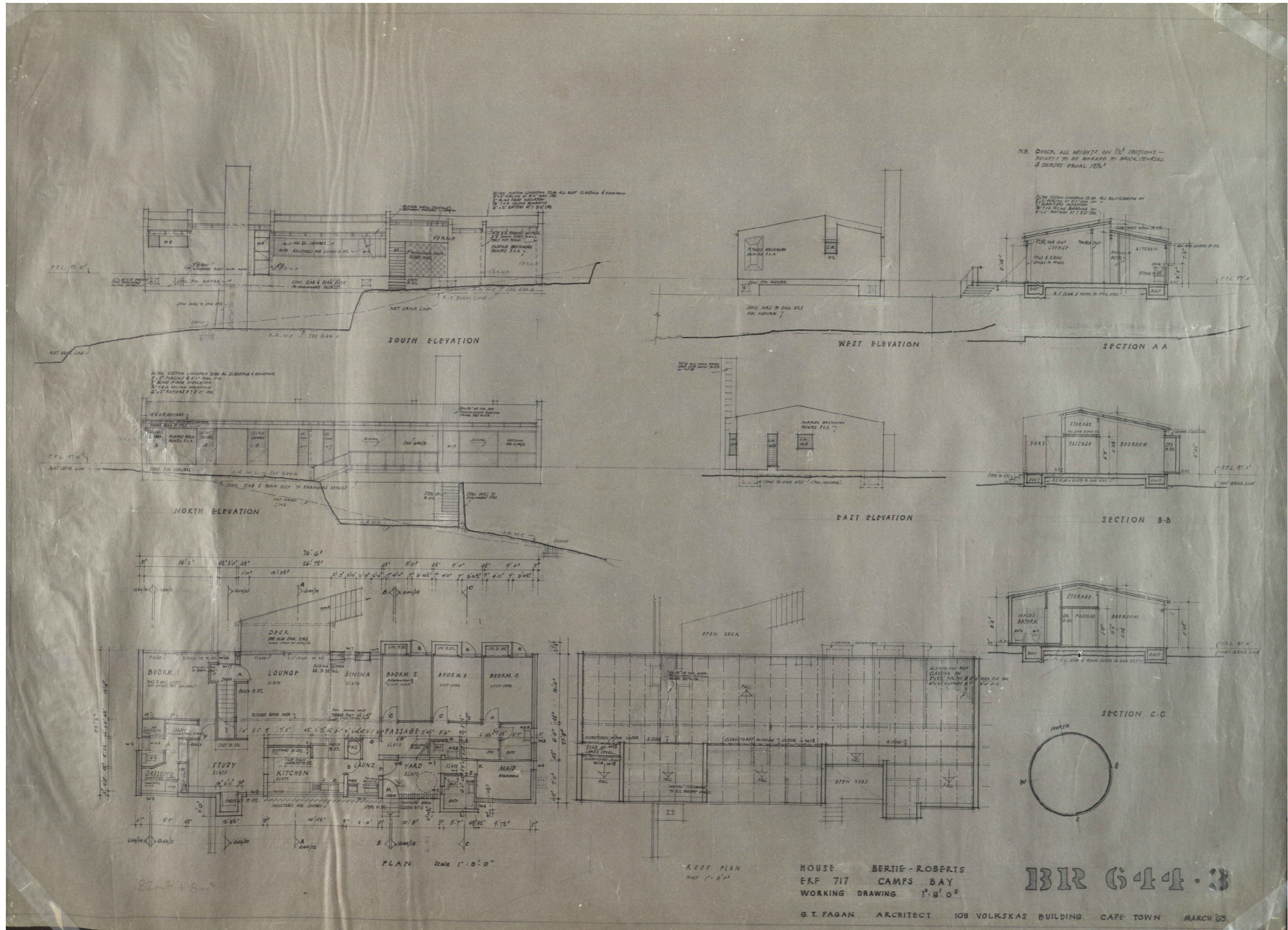
11. Working drawing
