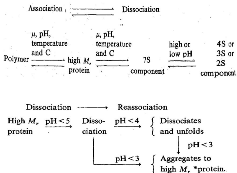
Figure 2.10 Association-dissociation of protein at varying pH condition (Prakash & Narasingo Rao, 1988)
