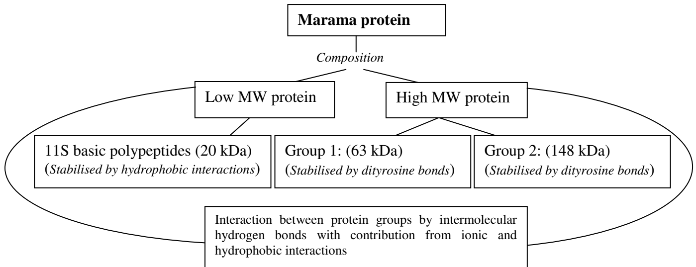
Figure 4.3 Summary diagram of proposed marama protein composition
