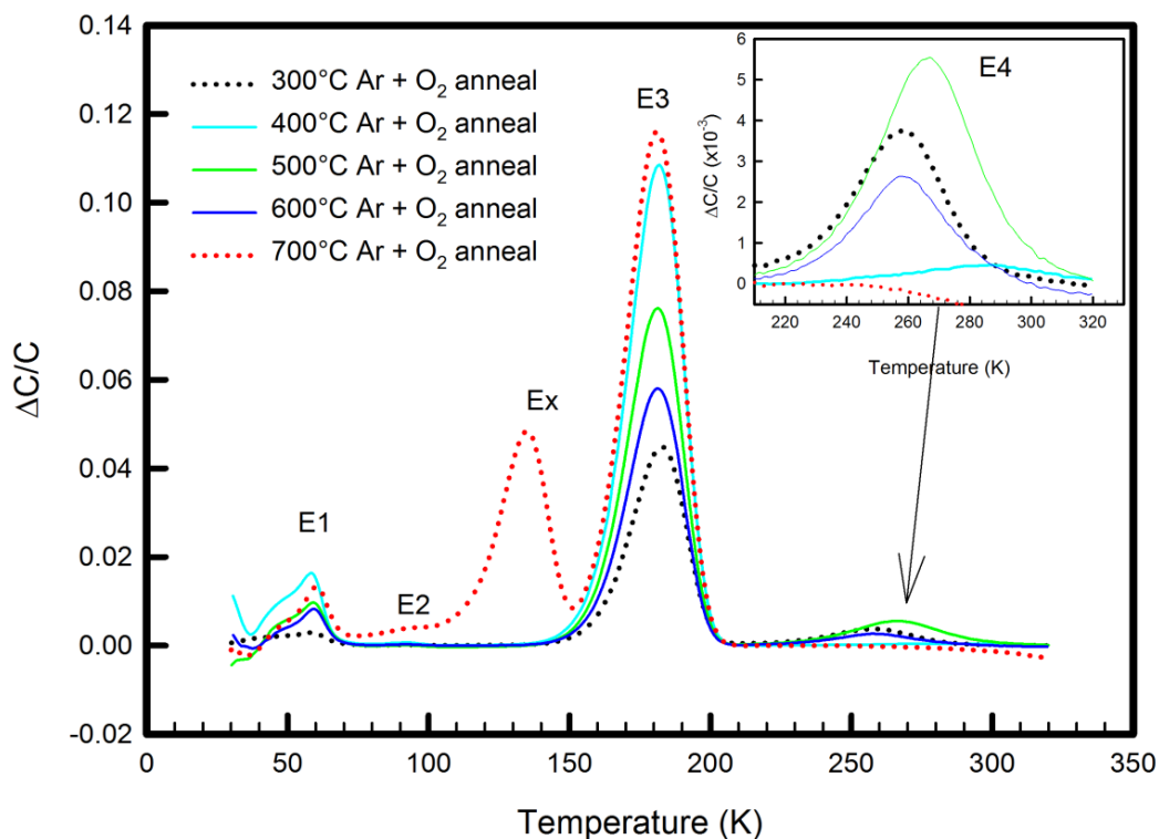
Figure 6.3.4.2: Normalized DLTS spectra of ZnO samples annealed in Ar + O 2 at different temperatures. The spectra were recorded on the 5 th of May 2012. The measurement conditions comprised of a quiescent reverse bias of 2.0 V, filling pulse V_p = 0.3 V, filling pulse width of 2.0 ms and a rate window of 100 \text{ s}^{-1} .
