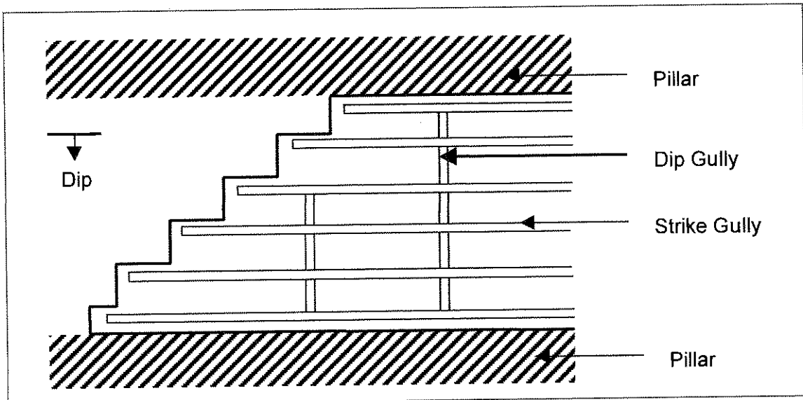
Figure 2.6 - Schematic representation of a deep level longwall-mining layout.
