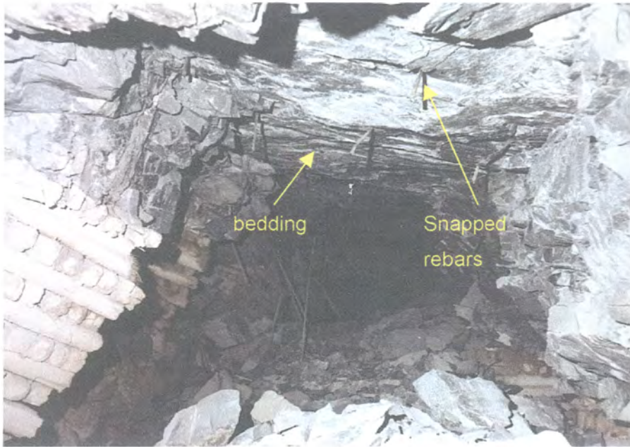
Figure 4.36 - Collapse back along a gully as a result of seismic activity. The hangingwall has collapsed between packs up to a bedding parting. Rebars are snapped or exposed
