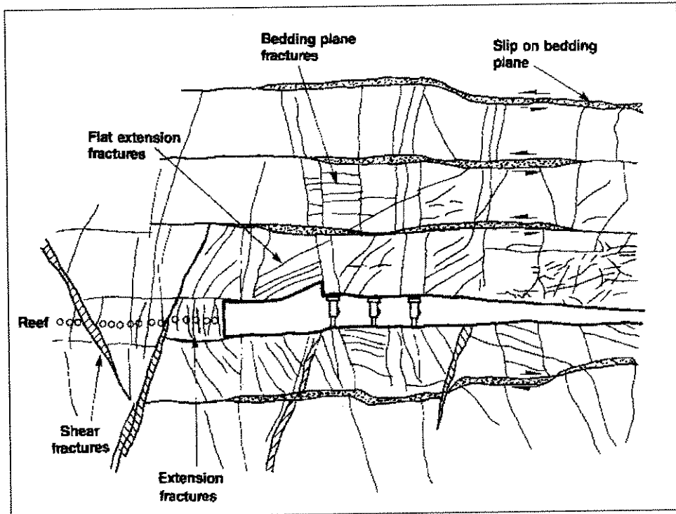
Figure 2.8 - Typical expected fracture pattern around a deep mine stope (after COMRO, 1988.)
