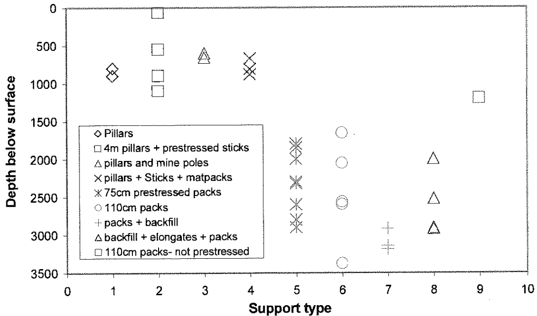
Figure 3.8 - Application of gully edge support types as a function of mining depth on gold and platinum mines, as required in mine standards
