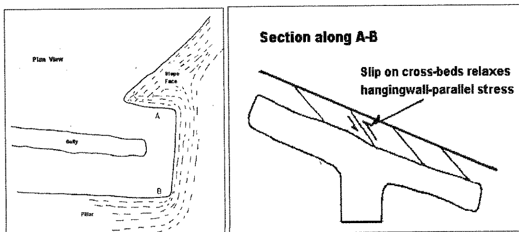
Figure 2.15 - The configuration of a wide advanced heading and a strongly underhand face as used at ERPM (after Turner, 1987)
