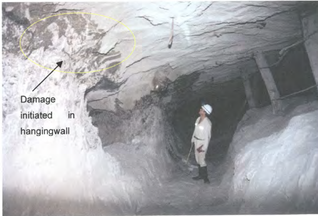
Figure 4.15 - Gully with no siding on the Merensky Reef at 800 m depth. Conditions are stable, although spalling has clearly occurred along the pillar sides. Note that pillar edge damage runs up and into the hangingwall
