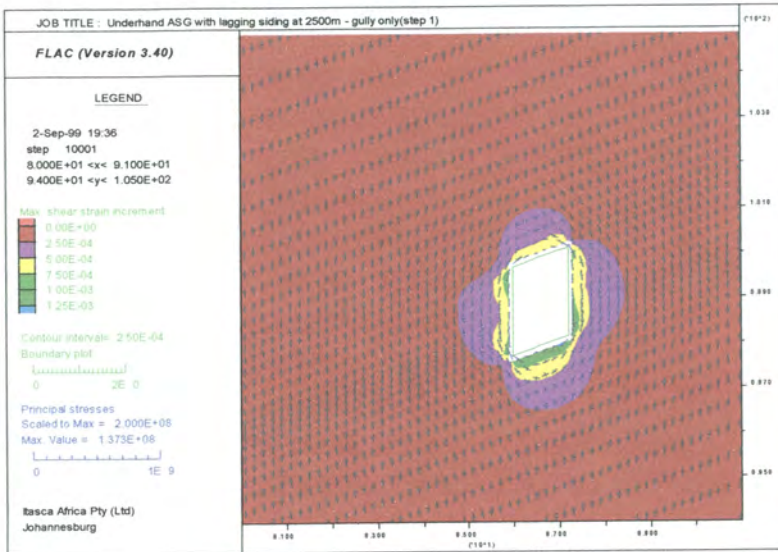
Figure 5.15 – Sequence of plots showing the change in conditions around a gully advanced as an ASG, with stope and siding subsequently excavated around it
