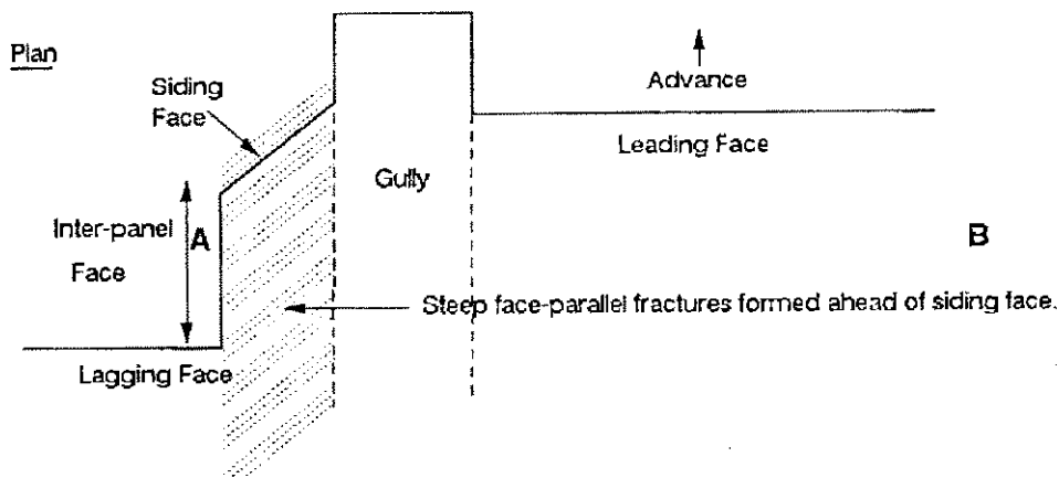
Figure 2.13 - Underhand siding face forms steep fractures to block low-inclination fracture propagation (after Turner, 1990)
