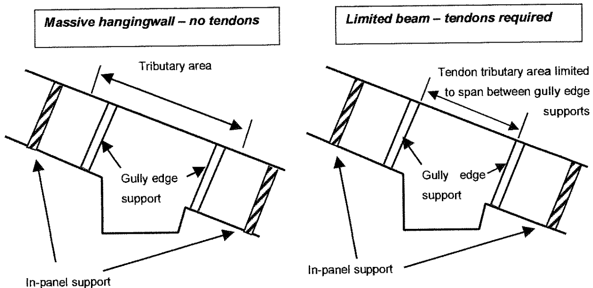
Figure 6.2 – Recommended tributary areas for calculation of required gully support pressures in low stress mining areas
