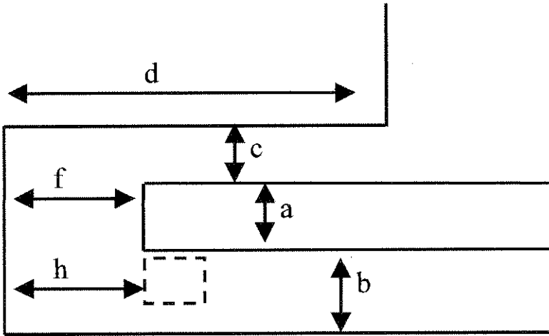
Figure 3.6 - Wide heading
