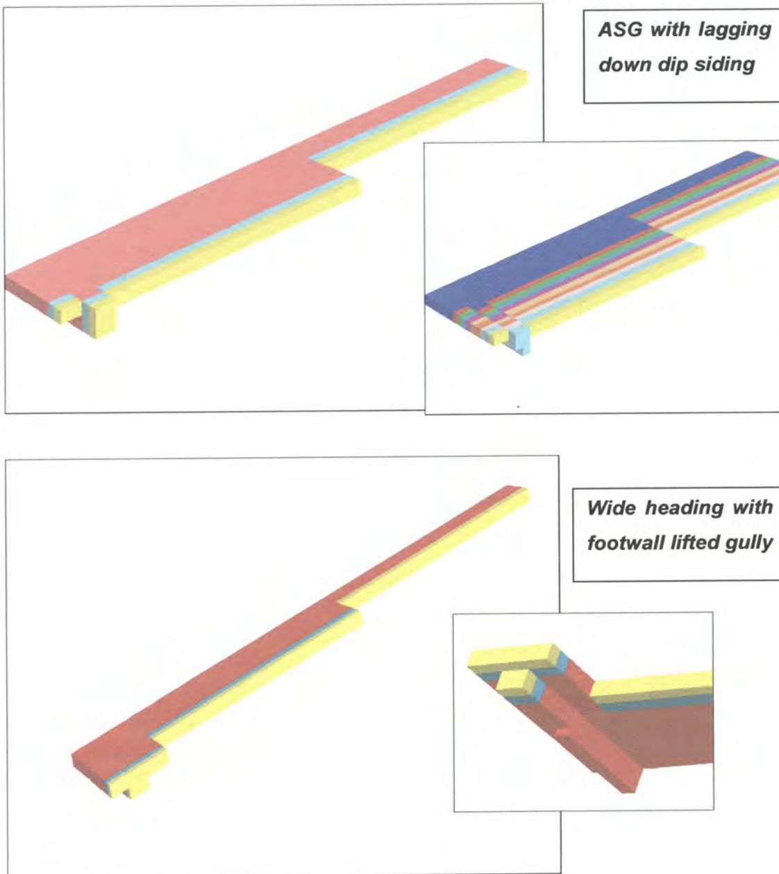
Figure 5.23 – Examples of excavations modelled using FLAC3D. Views show ASG with lagging siding and wide heading cases
