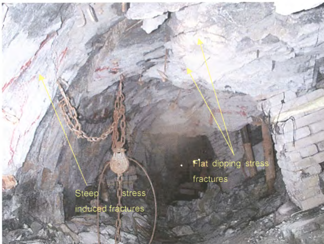
Figure 4.28 - Basal Reef - combined effect of an ASG heading, plus a lagging siding when strata is well bedded at 1700m below surface
