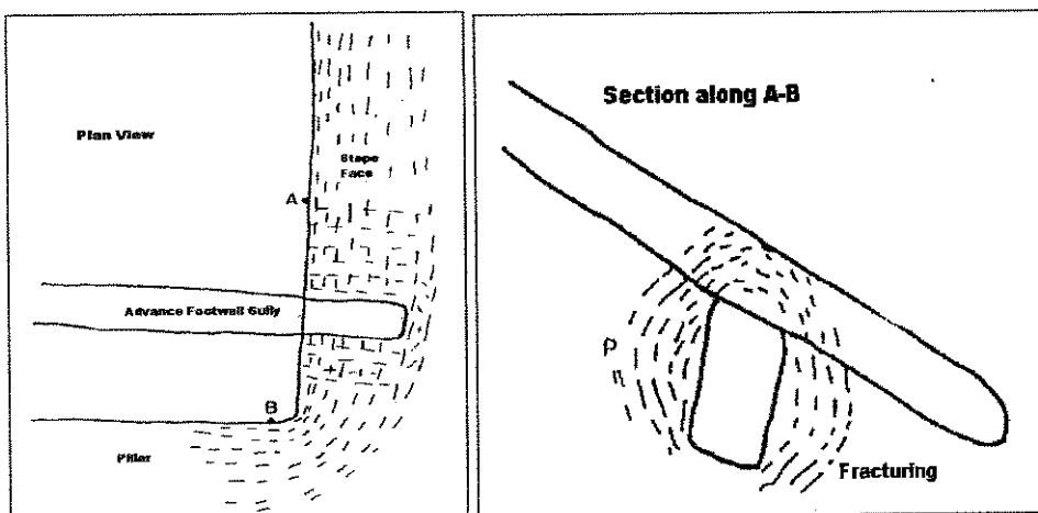
Figure 2.12 - The likely fracturing around a gully-width advance heading developed in the footwall of the stope (after Turner, 1987)
