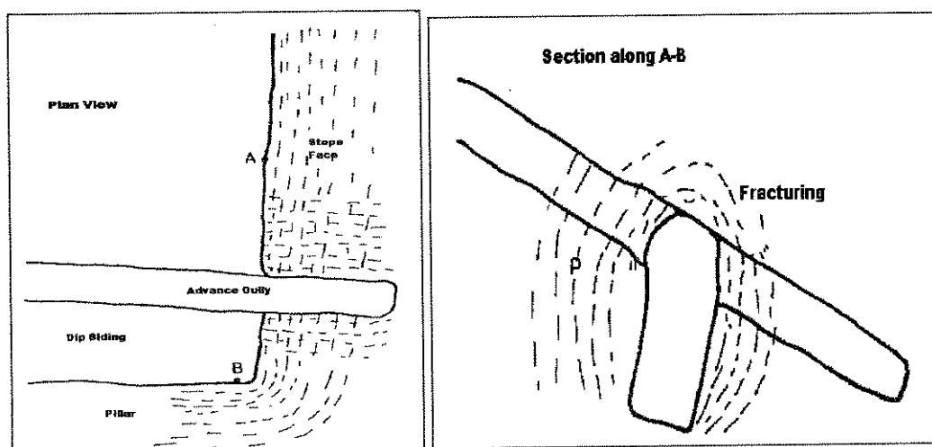
Figure 2.11 - A layout where the gully is carried ahead of the face as an advanced heading and the resultant fracture pattern (after Turner, 1987)
