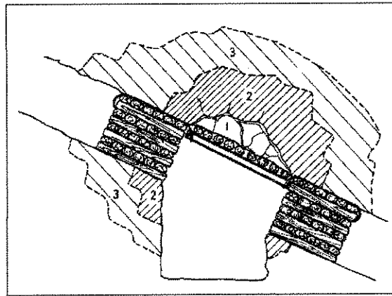
Figure 2.20 - A section through a gully indicating the three main stages of deterioration. Decking to keep the hanging in place not only provides safety but inhibits the second and third stages of deterioration in the hanging and footwall (after Cook et al. , 1972)
