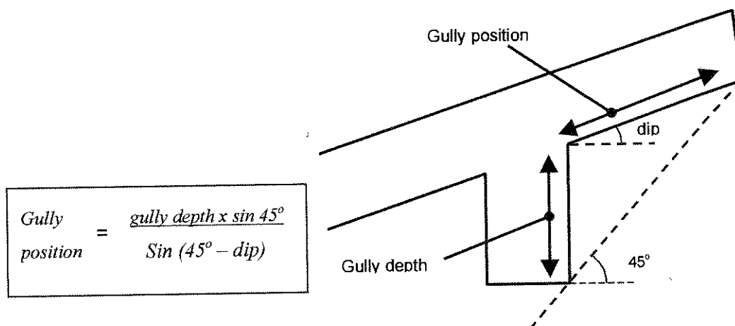
Figure 6.3 – A simple 45 degree rule for siting footwall lifted gullies in an overhand mining configuration
