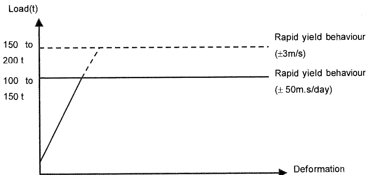
Figure 2.19 - Ideal gully pack performance. (after Roberts, 1995 and Spearing, 1995)
