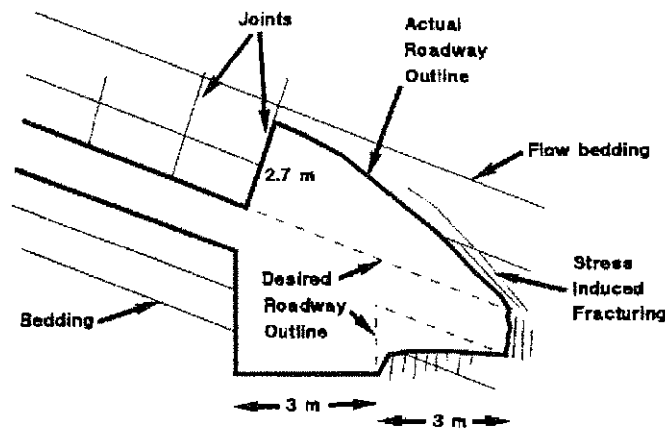
(c) Typical roadway shape which arises from fracturing and falls at the face
