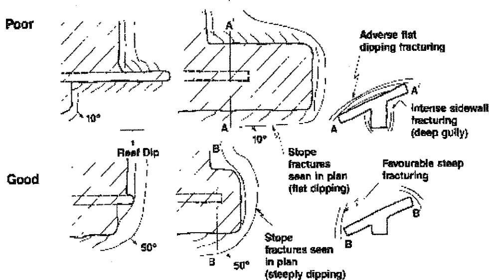
Figure 2.16 - Fracturing around gullies in deep stopes (after COMRO, 1988)
