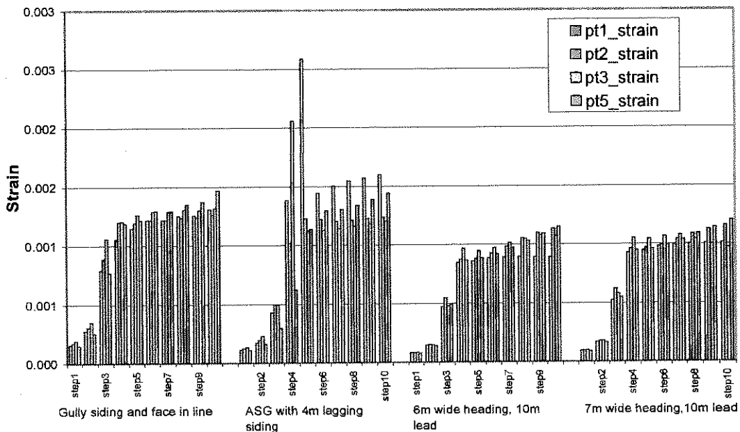
Figure 5.37 – Comparison of strains induced at monitoring points in the four sequentially mined models. Four points in one monitoring ring are shown for each mining step
