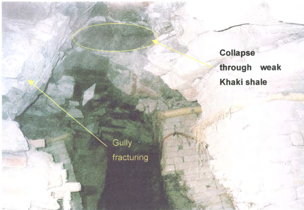
Figure 4.26 - Basal Reef – collapse of gully hangingwall due to fracturing developed around leading ASG heading at 1600m below surface
