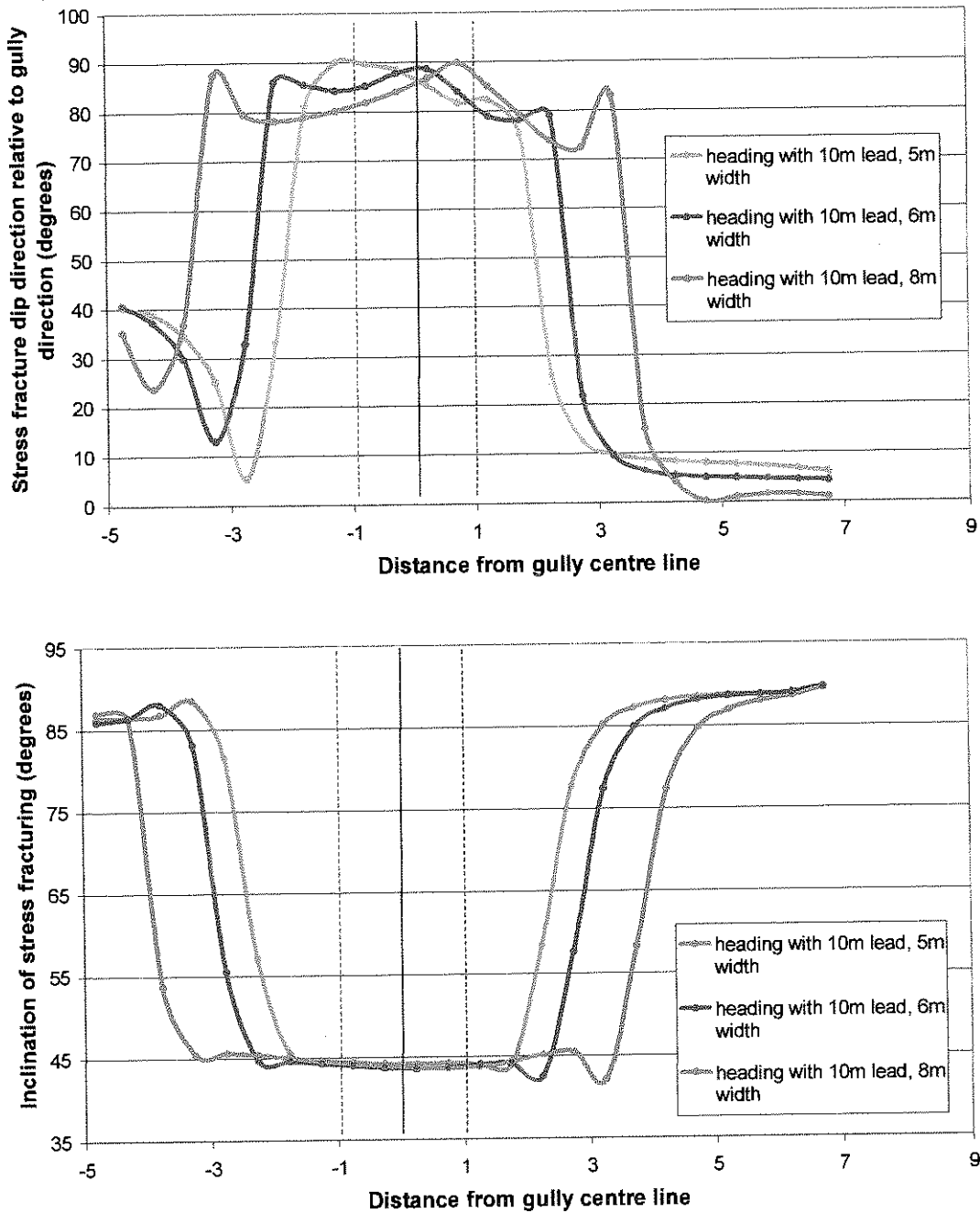
Figure 5.33 – Orientation of anticipated stress fractures in the hangingwall, around the face area of various widths of wide headings. Fracture strike relative to gully direction is shown in the upper graph, with fracture dip below. The graphs effectively represent a line of section across the gully
