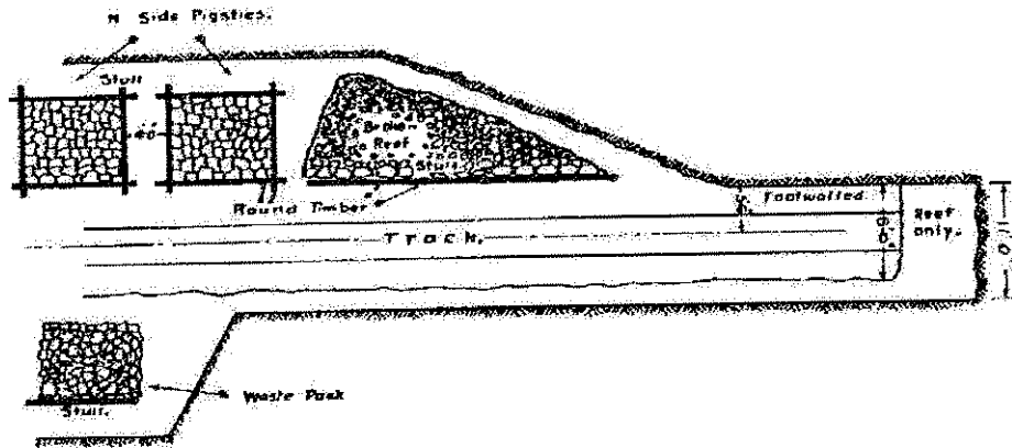
Figure 2.1 - Plan of resuing drive, used at Crown mines (after Walton, 1929)
