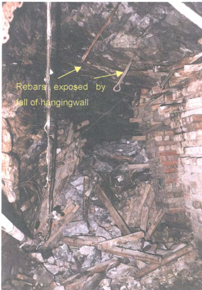
Figure 4.36 - Collapse back along a gully as a result of seismic activity. The hangingwall has collapsed between packs up to a bedding parting. Rebars are snapped or exposed
