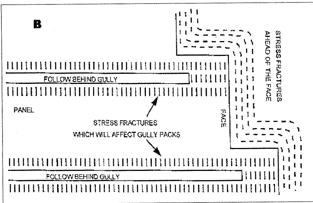
Figure 2.15 - A Schematic of expected fracture pattern for ASG configuration. B Schematic of expected fracture pattern for Follow Behind Gully configuration (after Squelch et al., 1995)
