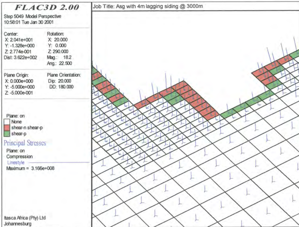
Figure 5.26 – Oblique view of a section parallel to reef at mid-height through an ASG and siding at 3000 m depth, showing the extent of rock mass damage, and principal stress tensor components indicating the stress path curving around and over the ASG heading
