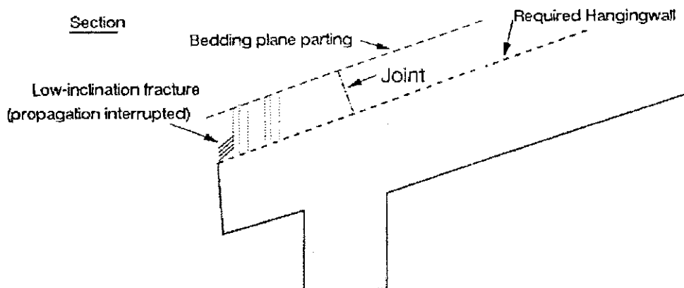
Figure 2.14 - Section through strike gully along A-B (after Turner, 1990), showing the propagation of low inclination fracture from the siding blocked by steep fractures
