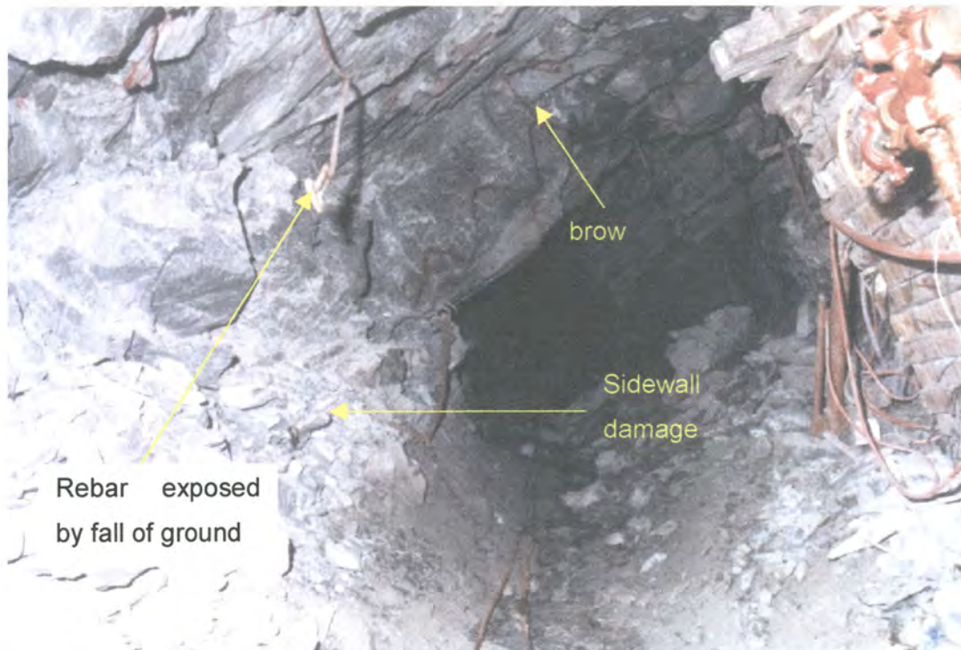
Figure 4.25 - Basal Reef - gully excavated at 2500m with no siding with stress damage causing down dip sidewall and hangingwall instability at 40° dip
