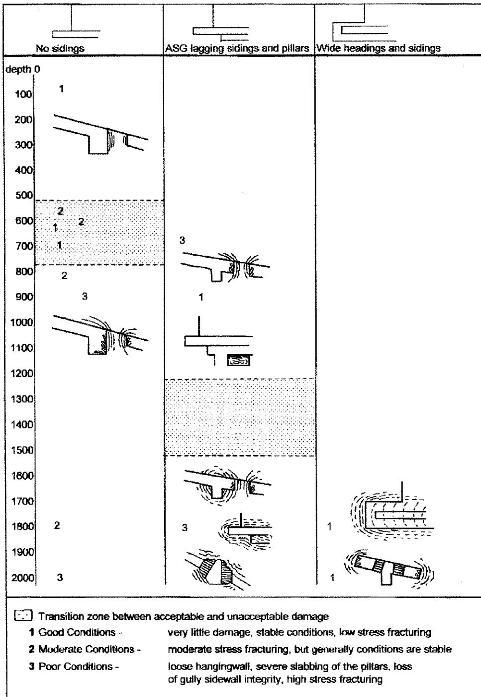
Figure 4.51 - Comparison of gully conditions versus depth in Bushveld platinum mines
