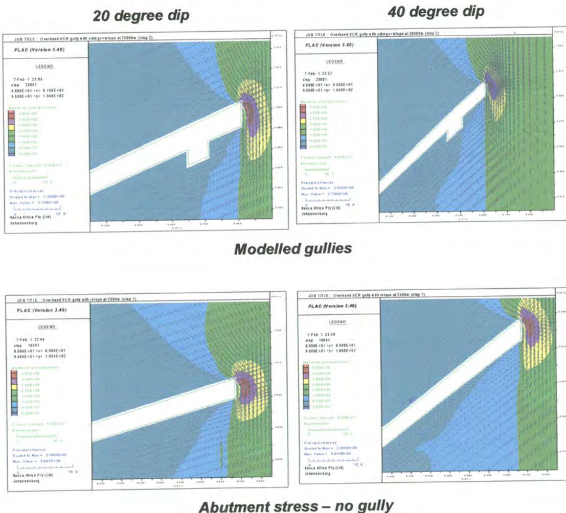
Figure 5.21 – Stress field around modelled gullies in an overhand environment (top), with generalised abutment stress conditions (below)
