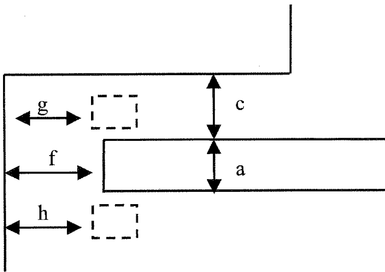
Figure 3.7 - Gully at top of the panel
