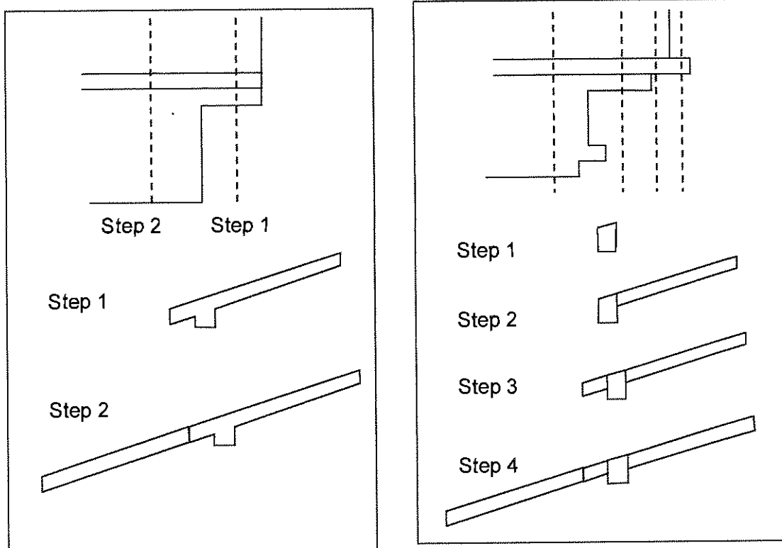
1. Gully & siding in line with face
