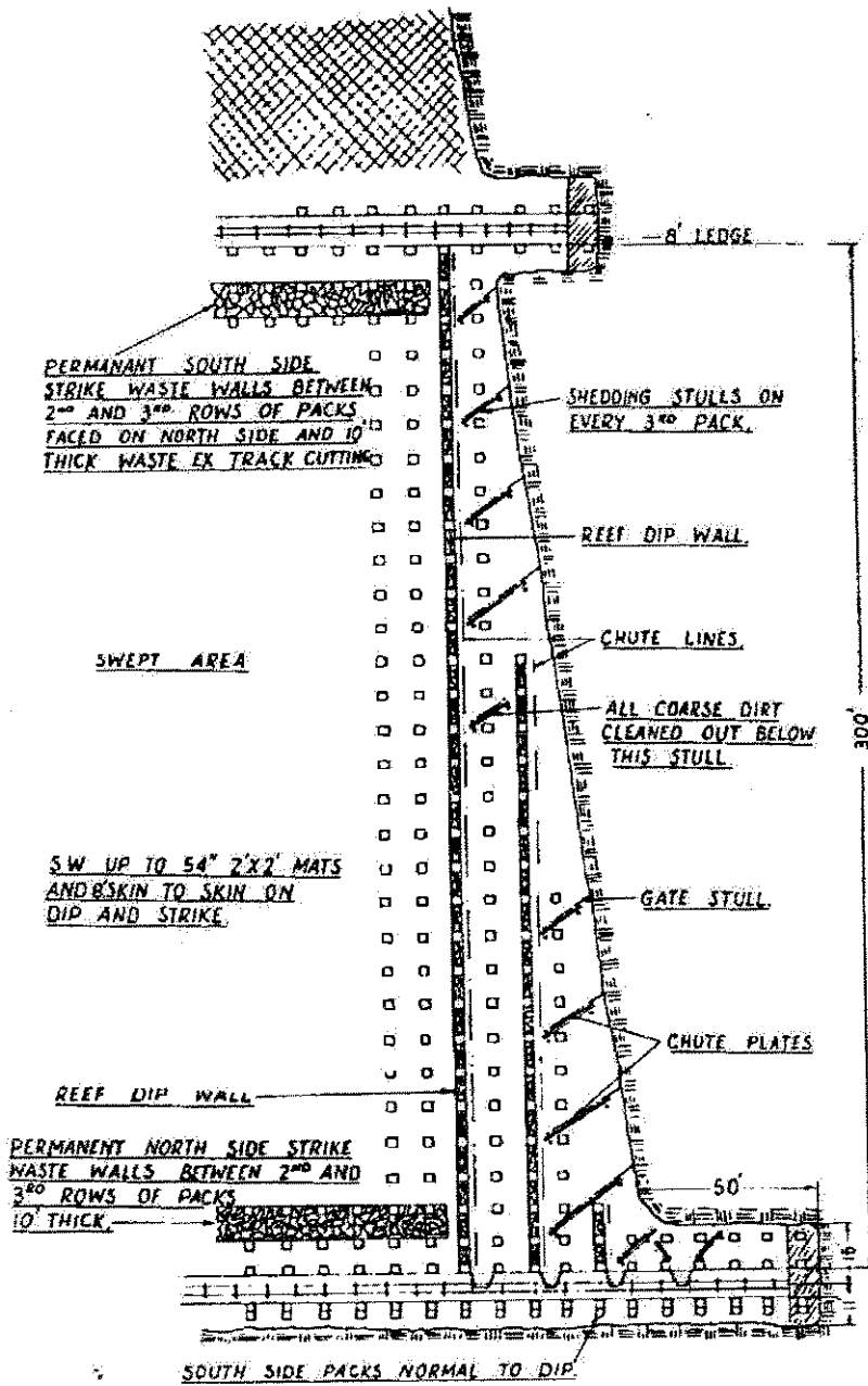
Figure 2.2 - Early application of wide headings at 2000 m to 2500 m depth at Robinson Deep (after Fouché, 1954)
