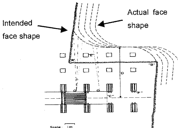
Figure 2.17 - A plan of a lead, or north side, between two panels showing the intended face shape (solid line) and the actual face shape (dashed line) (after Cook et al 1972)
