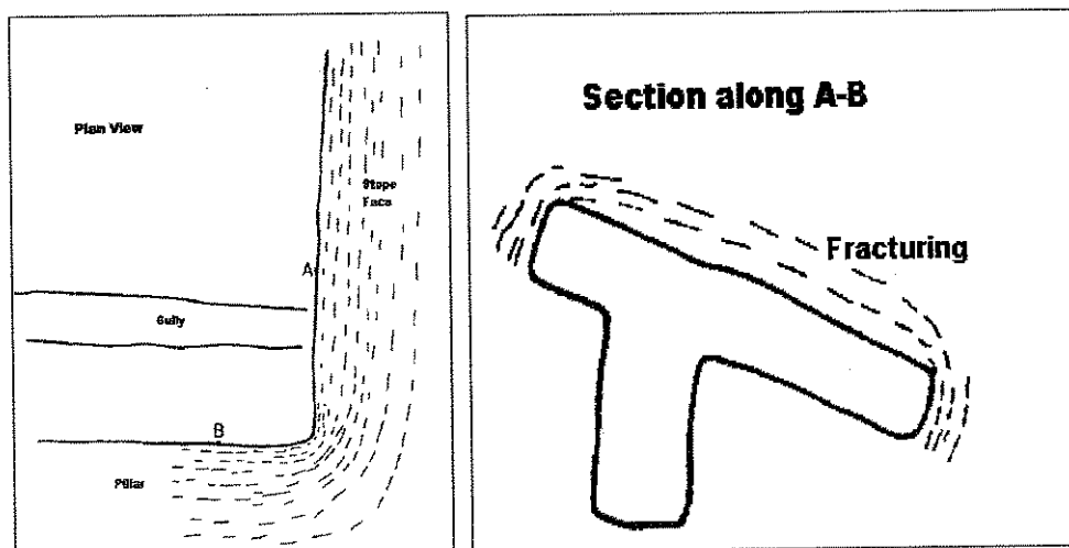
Figure 2.10 - The layout for mining with no advanced gully heading and the resultant fracture pattern (after Turner, 1987)
