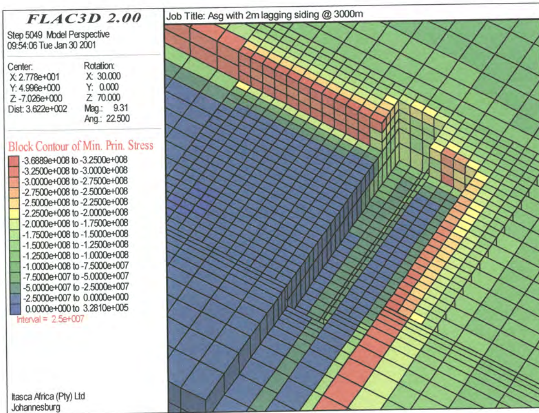
Figure 5.25 – View of an ASG model where the gully leads the stope face and siding by 2 m. The hangingwall is removed to show the model geometry and the rock mass is coloured according to stress level. Note that even a 2 m ASG at 3000 m depth appears to penetrate the high stress zone ahead of the stope face
