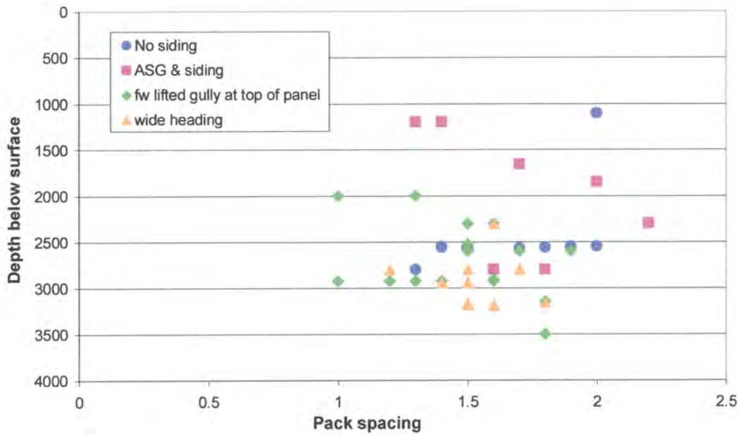
Figure 4.8 – Observed spacings of packs along gully shoulders at various gold mines industry-wide, shown versus mining depth
