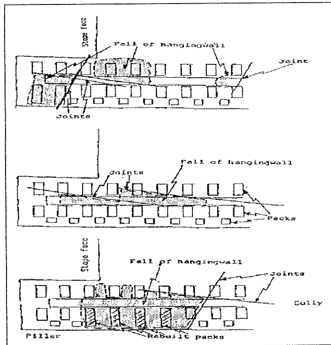
Figure 2.18 - Common falls of ground geometries and distributions, with respect to gullies and wide headings adjacent to stabilising pillars in Carbon Leader Reef (after Turner, 1987)
