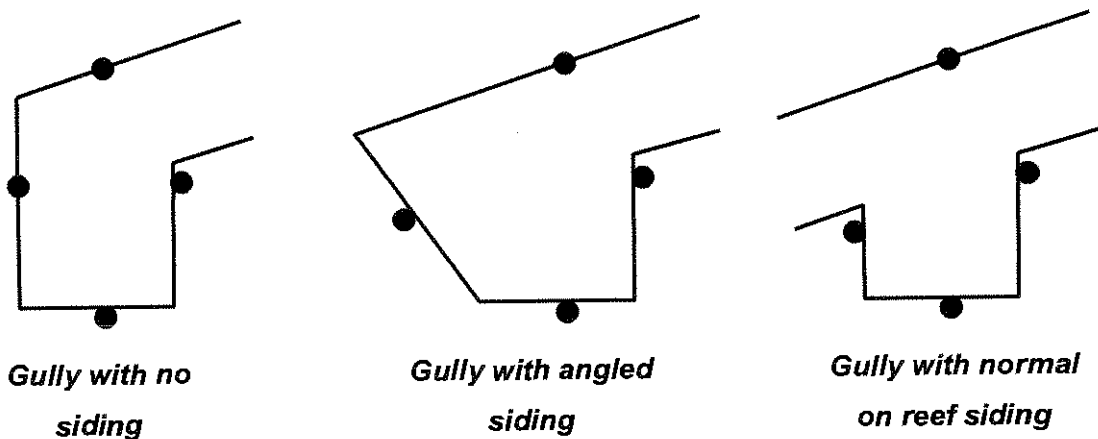
Figure 5.5 – Sketch sections of gully geometries modelled, showing monitoring points used in the analysis
