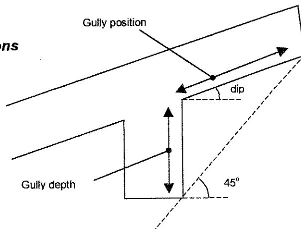
Figure 5.22 – A simple 45 degree rule for siting footwall lifted gullies in an overhand mining configuration
