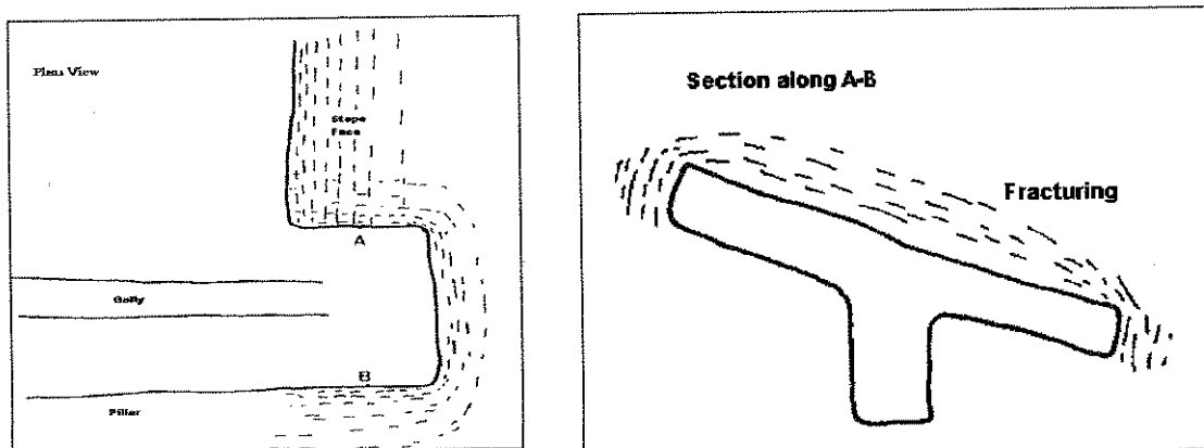
Figure 2.9 - The layout and resulting fracture pattern for mining with a 10m wide heading advanced 5-10m ahead of the face (after Turner, 1987)
