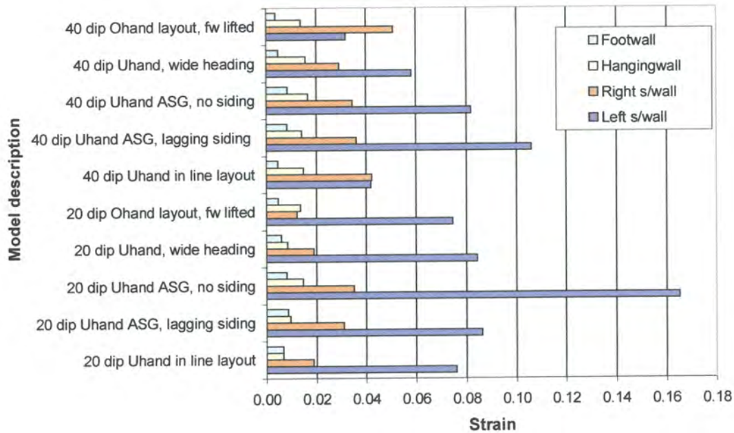
Figure 5.19 – Comparison of final strains induced in gully boundaries throughout each model analysis (20 and 40 degree dip cases, 2500 m)
