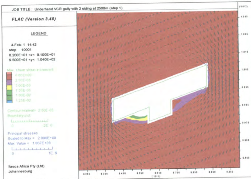
Figure 5.17 – Rock mass behaviour when gully is excavated in a wide heading. In the top view only the heading and gully are excavated, with the up dip slope added in the lower view
