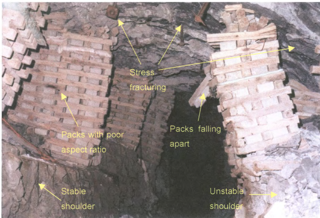
Figure 4.33 – VCR - Typical conditions that may develop along a gully created as an ASG with lagging siding under high stress
