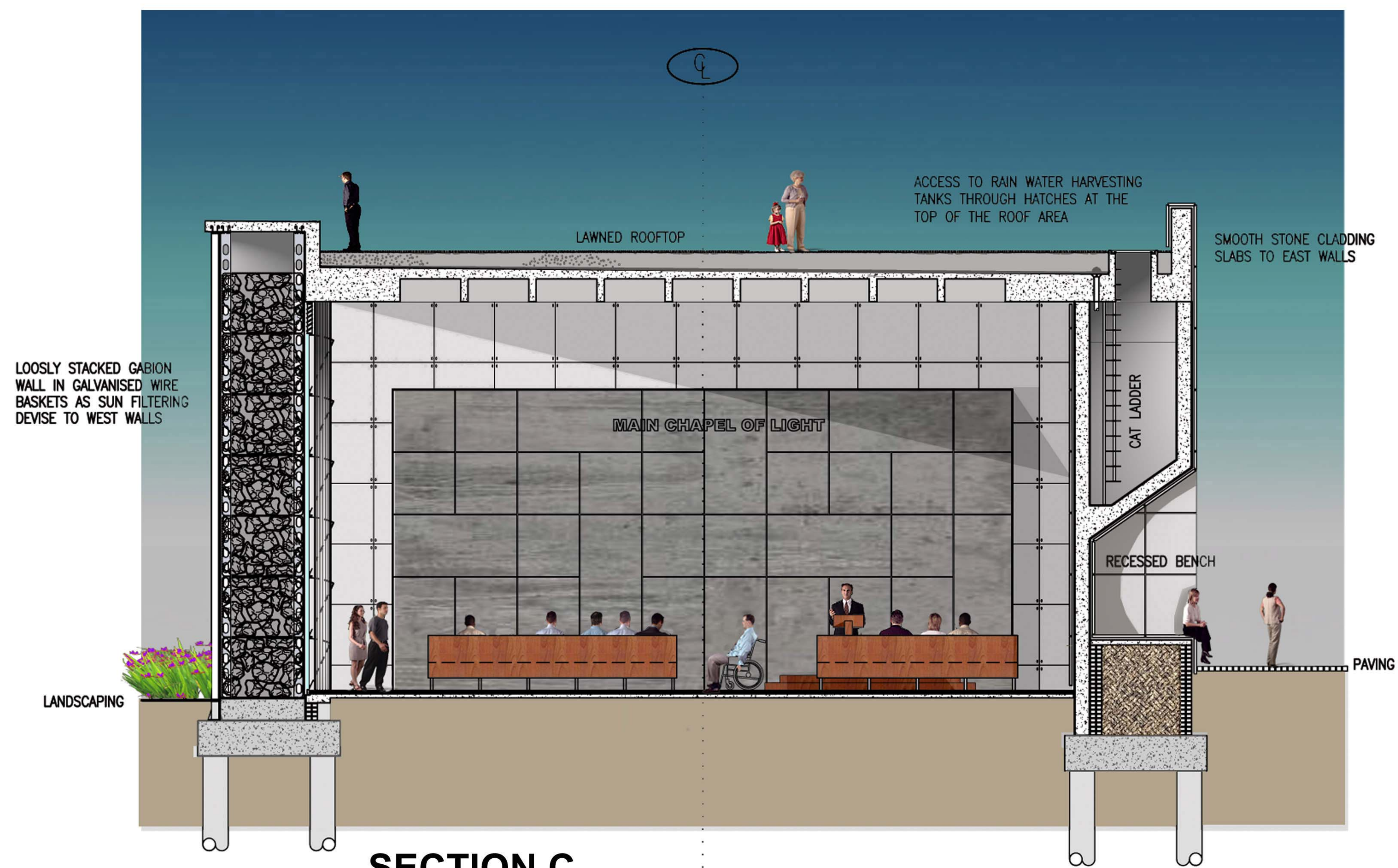
SECTION C SCALE 1:50 MAIN CHAPEL OF LIGHT
