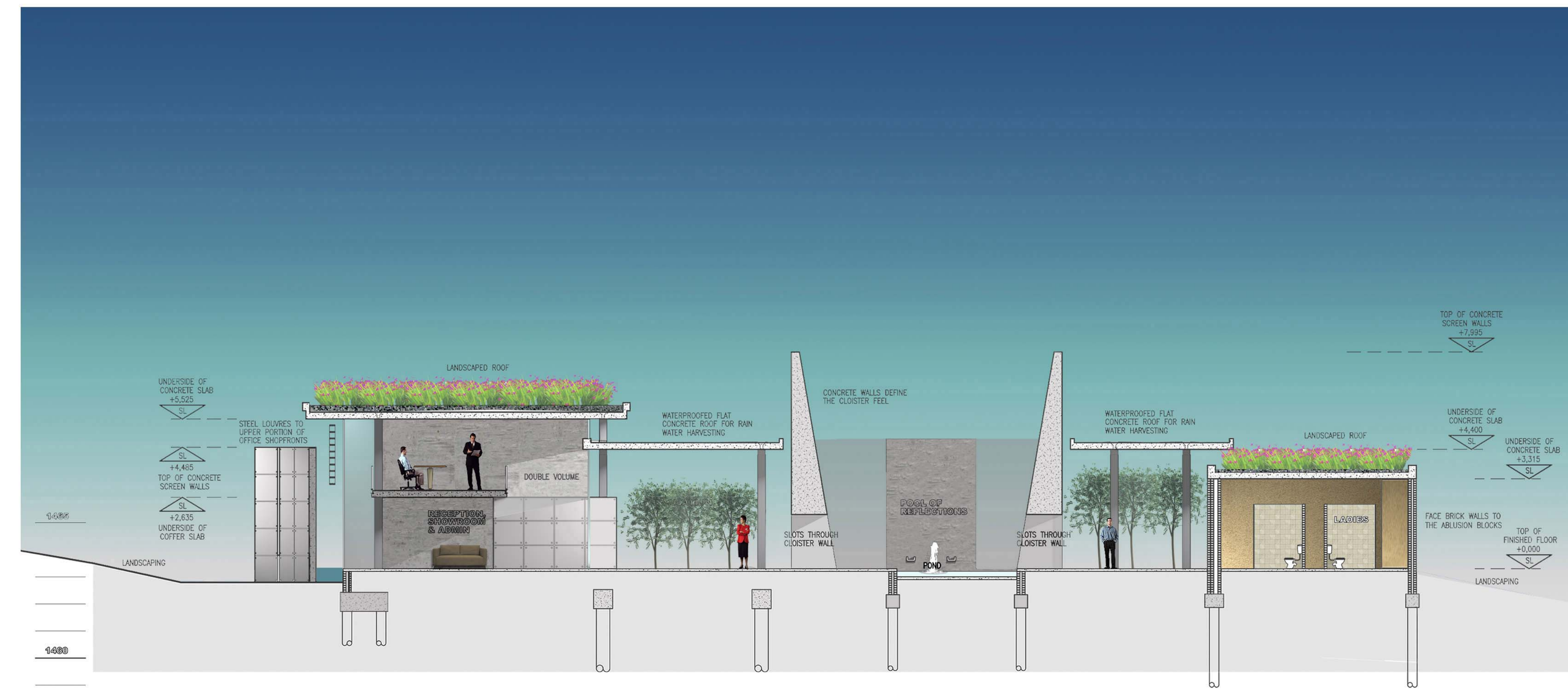
SECTION B-B SCALE 1:100 WELCOMING CENTRE
