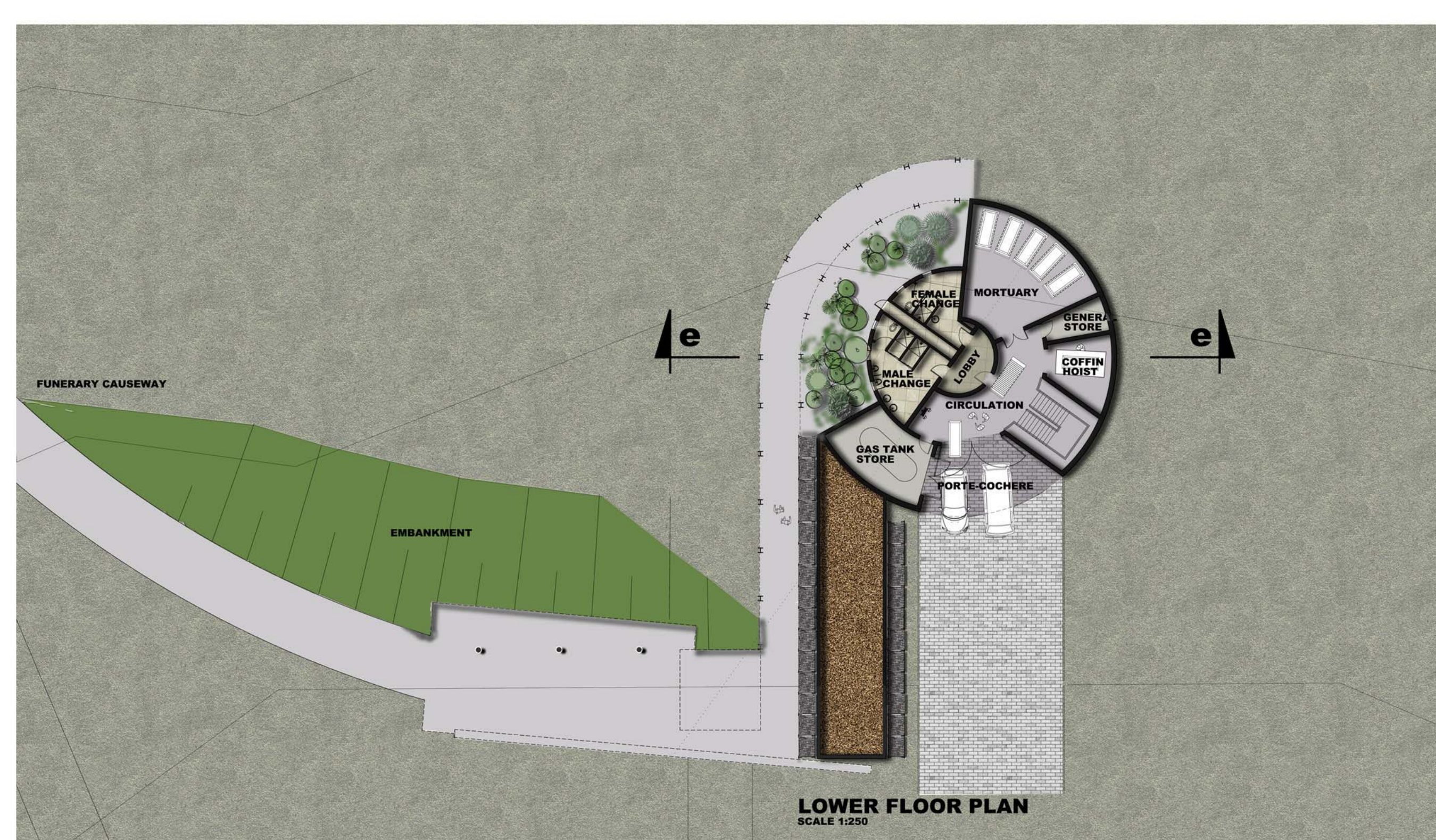
LOWER FLOOR PLANS SCALE 1:250
