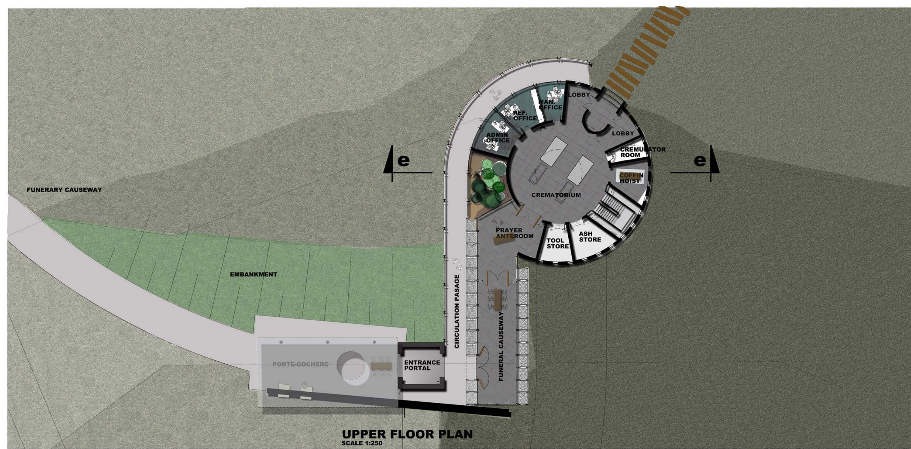
UPPER FLOOR PLANS SCALE 1:250
