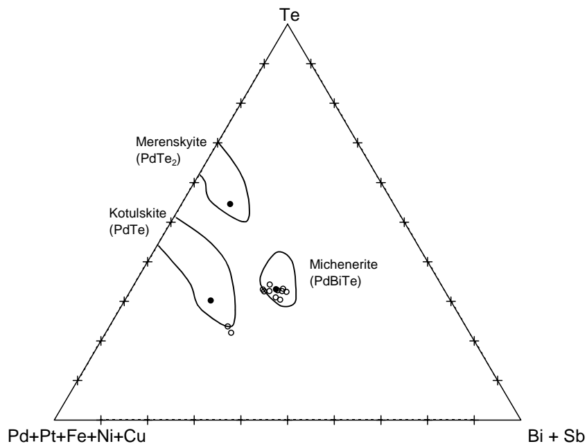
Figure 5: Composition (at %) of natural Pd-Pt-Bi-Te minerals from Mimosa Mine in the Great Dyke of Zimbabwe (Oberthür, 2002c). The curved lines enclose the compositional fields of the respective minerals reported in the literature (Wilson et al. , 1993).
