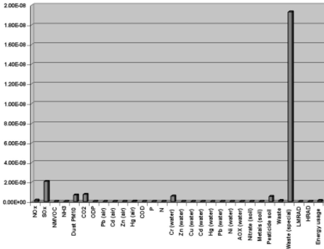
Figure 3.8: Normalisation results of the Ecopoints procedure
