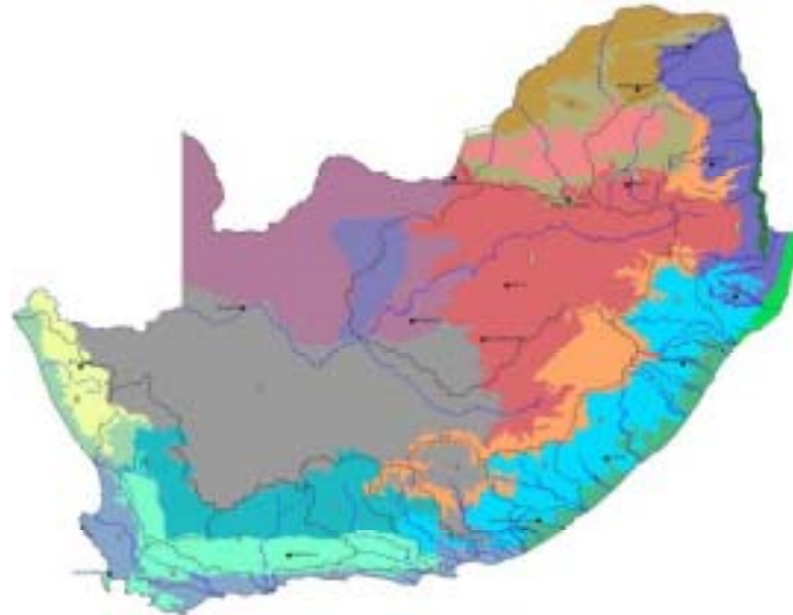
Figure 4.2: Eco-regions of South Africa [23]
