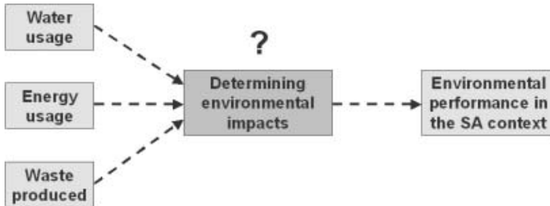
Figure 1.15: Assessing environmental performances from limited parameters
