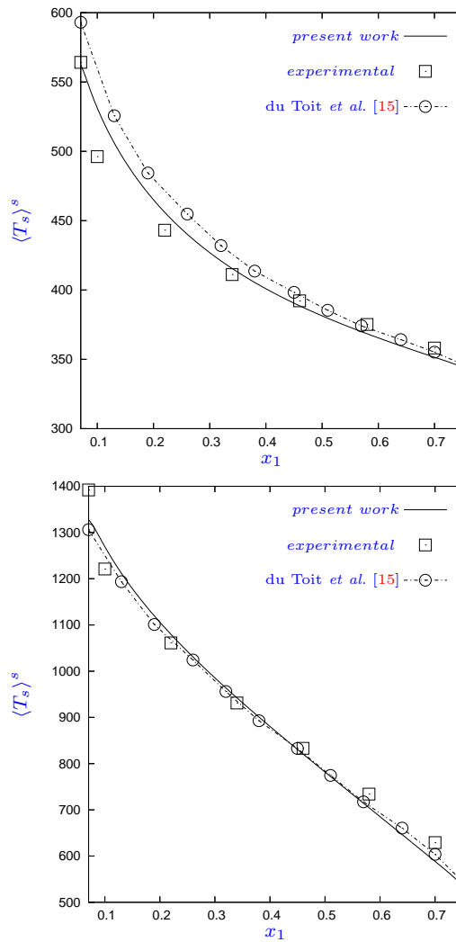
Figure C.1: Predicted pebble temperature distribution at 0.09 m vertical elevation compared to experimental measurements for 5 kW (left) and 35 kW (right).
