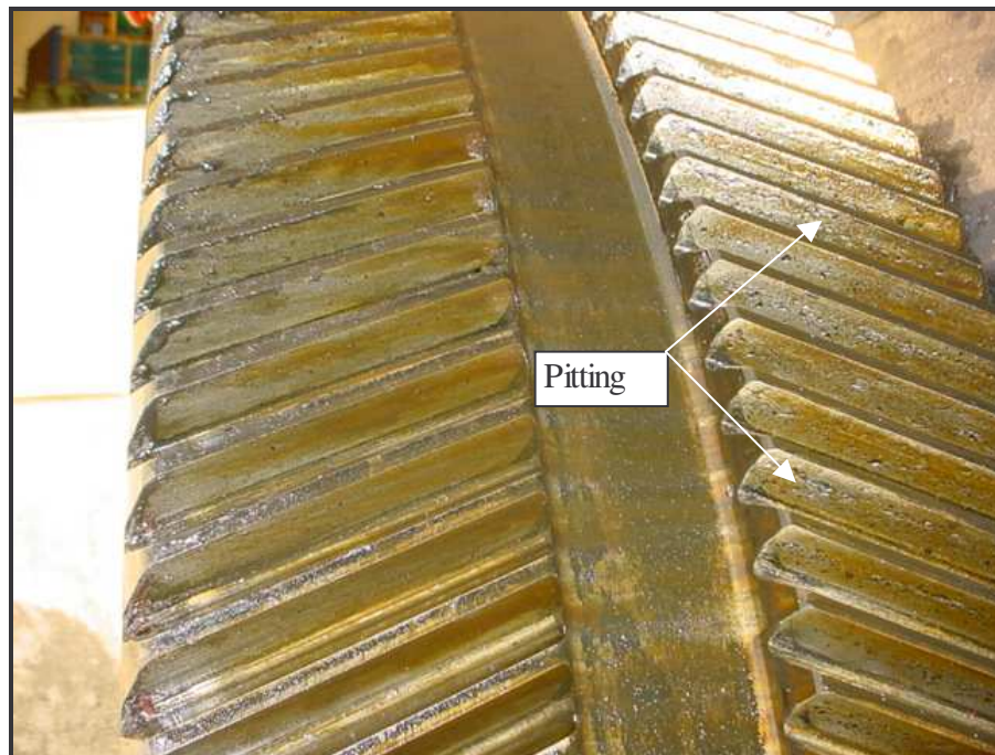
Figure 4.12: Bull gear showing pitting on one set of teeth.
