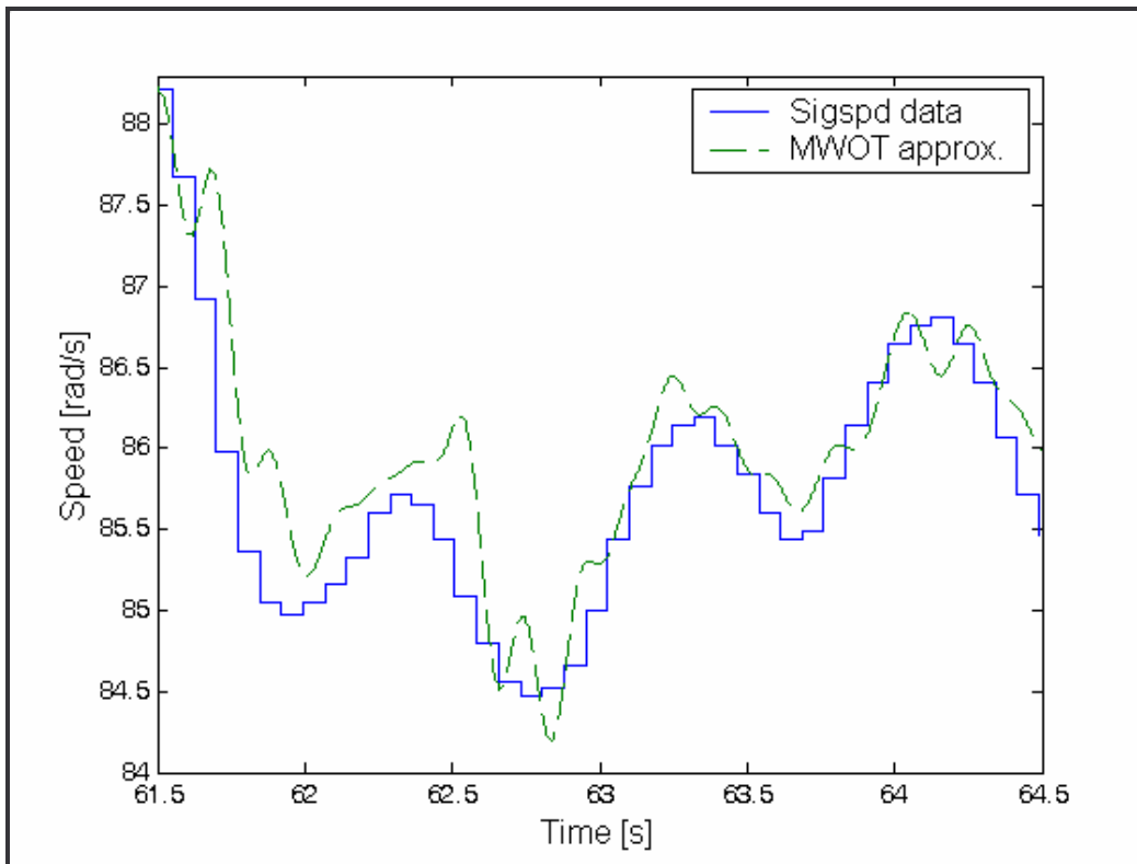
Figure 3.11: Showing the difference between sigspd.m data and MWOT data using segments with a length of 4096 points.
