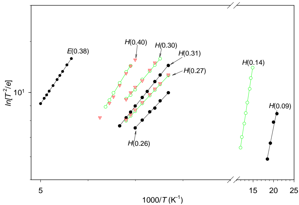
Fig. 10-6. The Arrhenius plots of the defects created in n-Ge after 3 keV sputtering with Ar ions with a dose of 1 \times 10^{14} \text{ cm}^{-2} for as-sputtered and recorded after a month (solid black circles), after annealing at 225°C (open green circles) and after annealing at 275°C (open red triangles).
