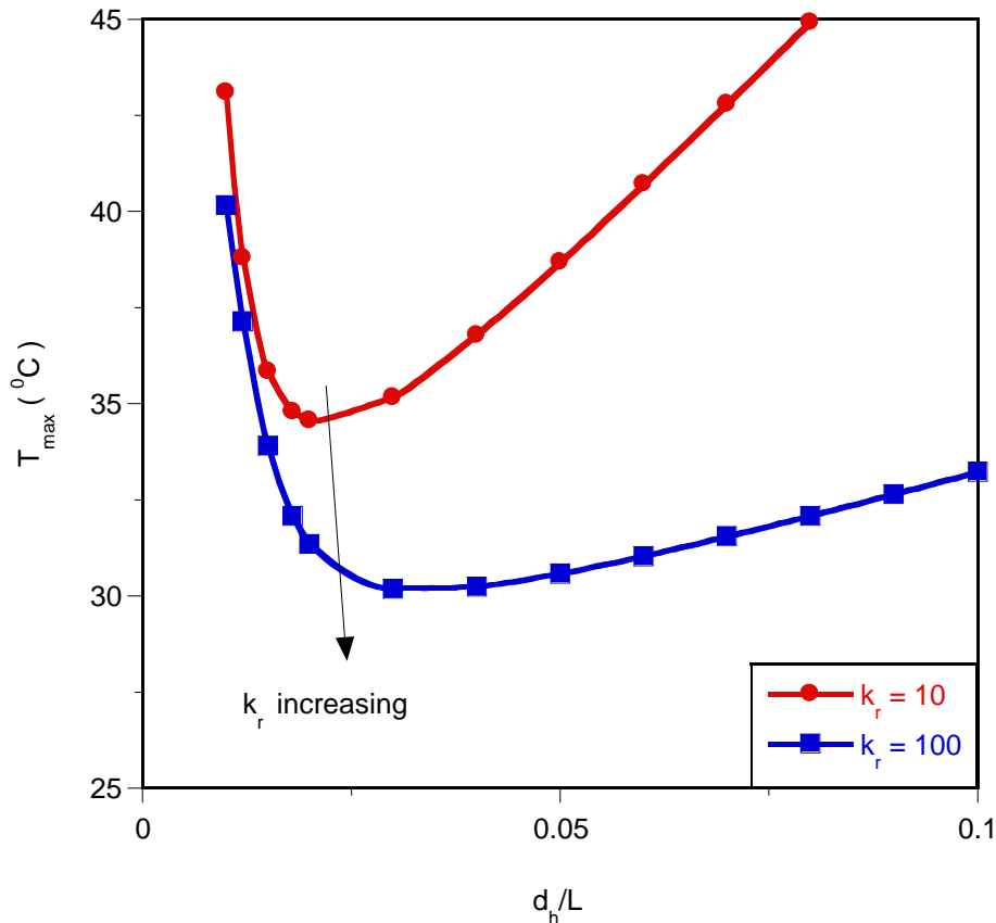
Figure 7.11 : Effect of a thermal conductivity ratio, k_r , on the peak temperature at a Bejan number of 10^8 and porosity of 0.2
