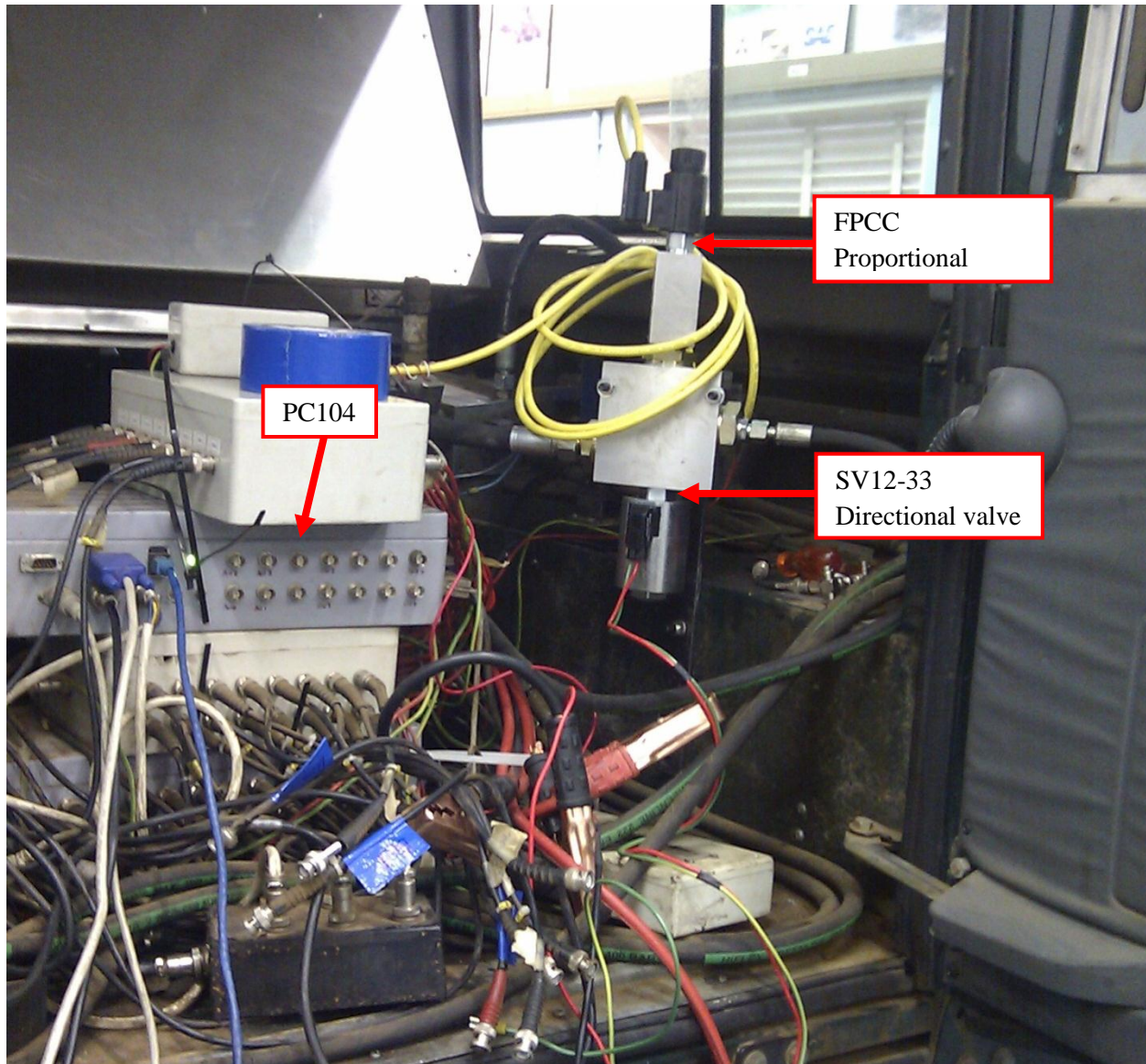
Figure 77 Valves for the rear suspension unit during characterisation
