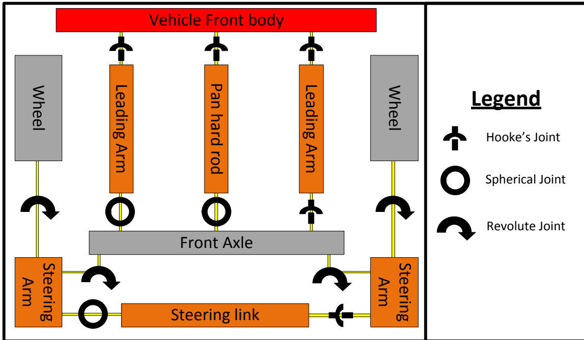
Figure 22 Schematic of the front suspension (Thoresson, 2007).
