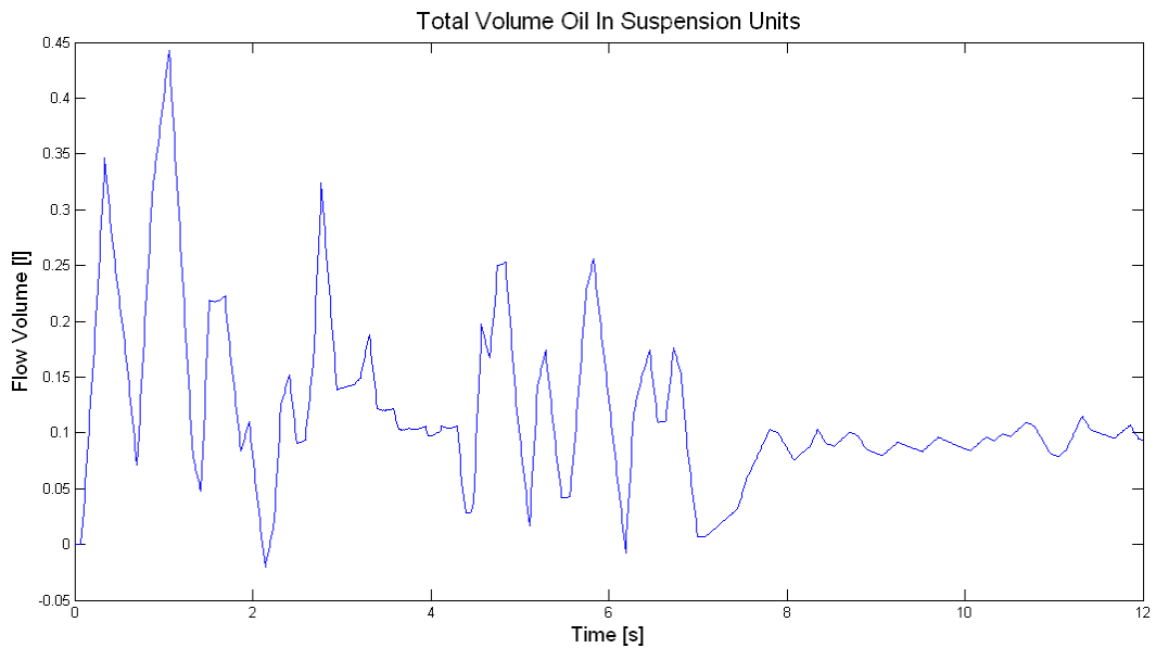
Figure 50 Total volume of oil pumped into the suspension
