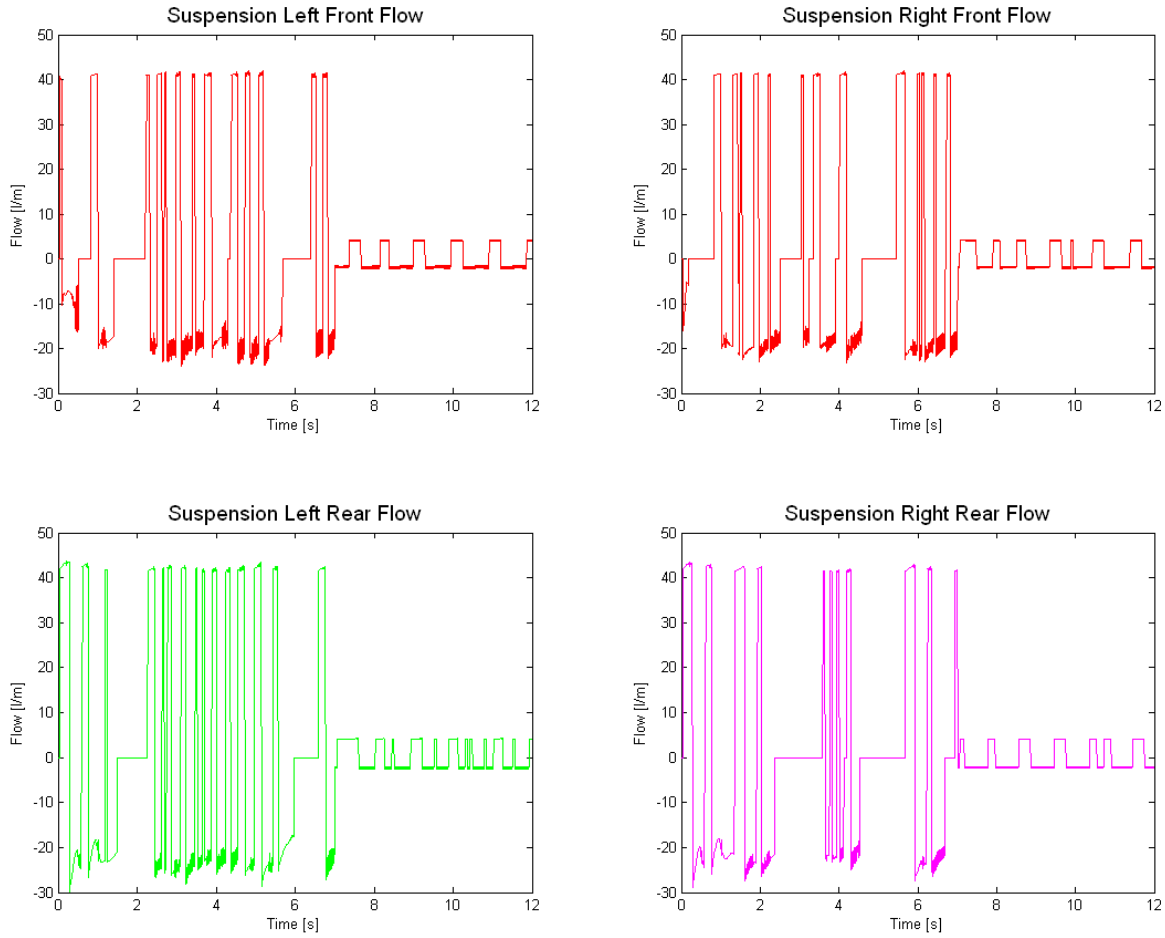
Figure 44 Flow rates for each suspension unit
