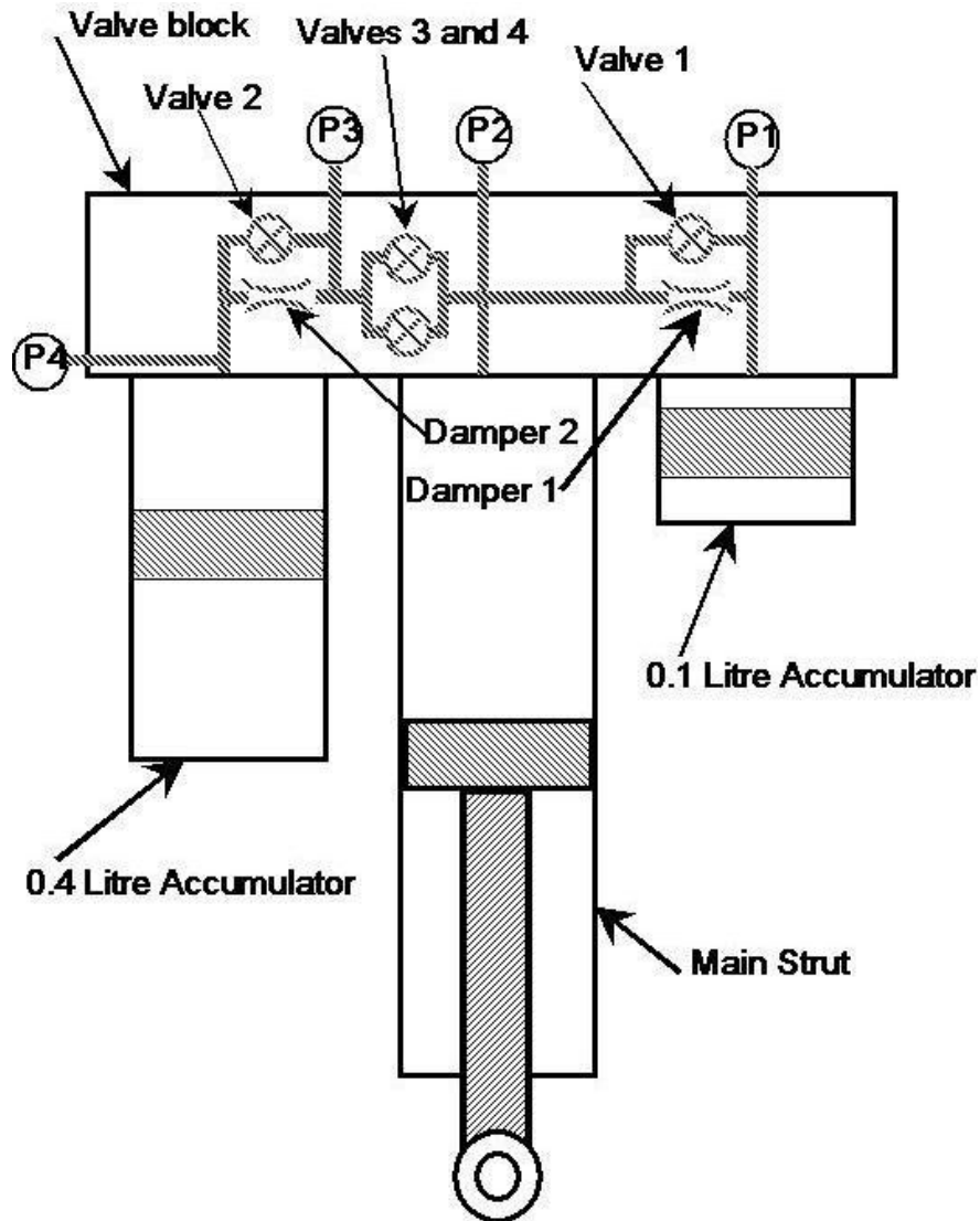
Figure 13 Schematic diagram of the 4S 4 (Els, 2006)
