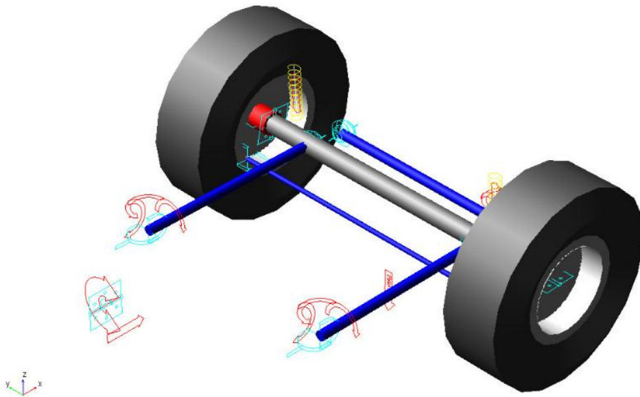
Figure 23 Front suspension in ADAMS model (Thoresson, 2007).
