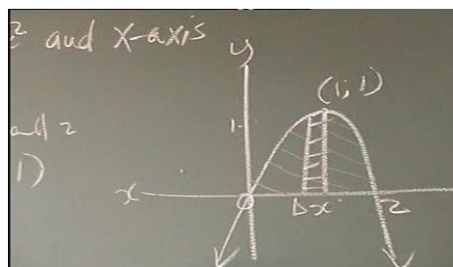
Figure 8.8: The parabola using a \Delta x strip
