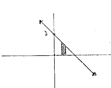
Figure 5.7: A line representing a solid
