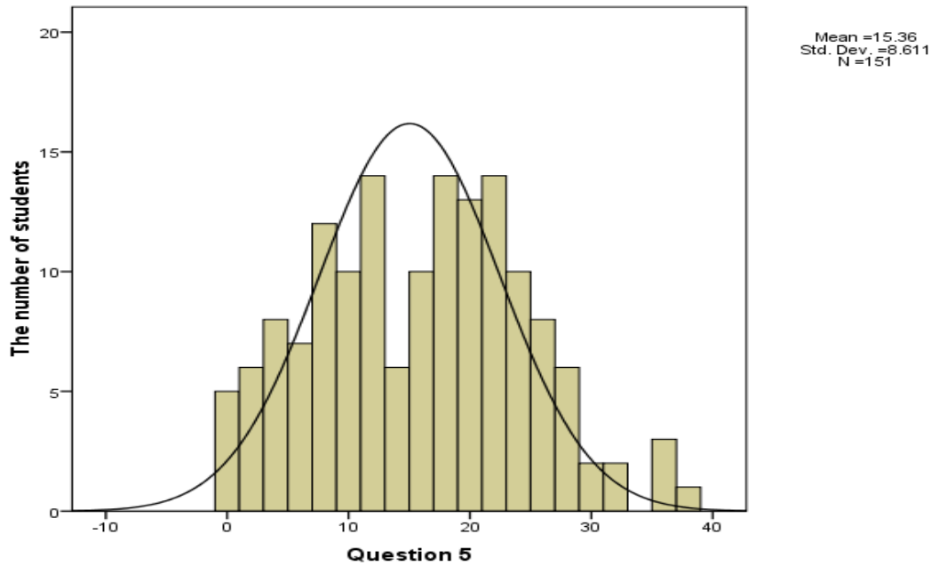
Figure 7.1: Performance in Question 5
