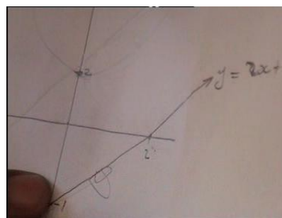
Figure 8.24: The straight line
