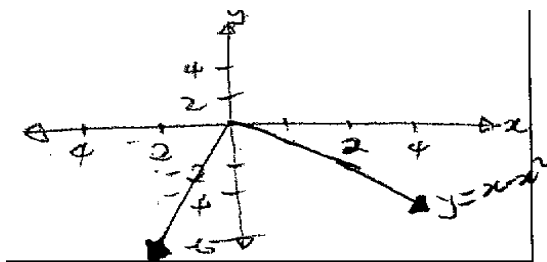
Figure 5.3: Straight lines as parabolas
