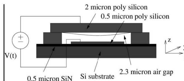
Figure 4.8: Schematic views of fixed-fixed beam microstructure used as pressure sensor [56].
