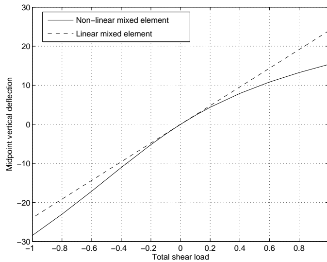
Figure 3.9: Load-displacement graph for Cook's membrane problem, which illustrates softening and hardening response.
