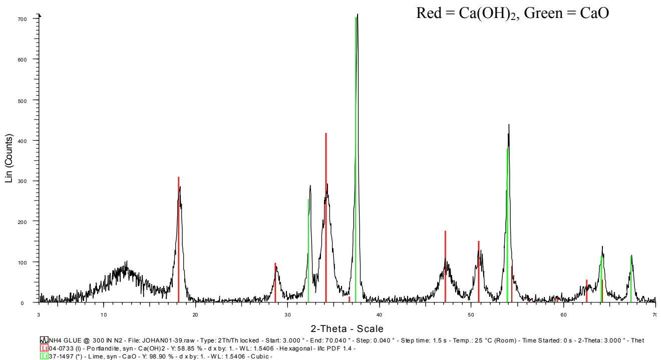
Figure 4-24 Calcium gluconate monohydrate heated at 1000°C for 5 minutes (air)
