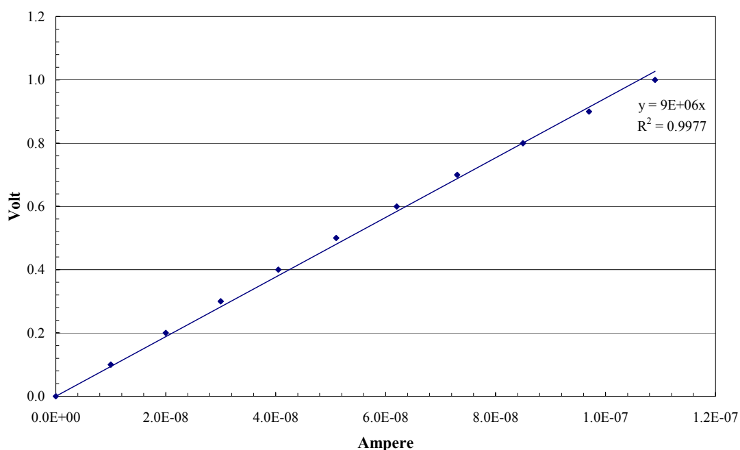
Figure 4-33 Conductivity measurements for embedded coked ammonium gluconate
